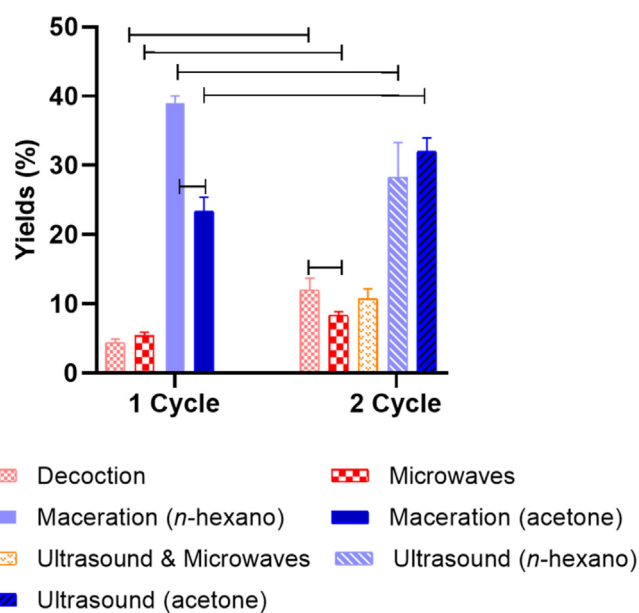
Figure 1. Yields obtained from different extraction methods. The bars represent the significant p -values comparing first and second cycle yields: decoction - 0.0017; microwave - 0.0009; maceration x ultrasound with n -hexane - 0.0215; maceration x ultrasound with acetone - 0.0056.
