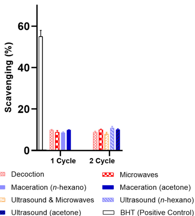
Figure 2. Graph of the antioxidant activity from the percentages of absorbance obtained by the extracts of each method.
