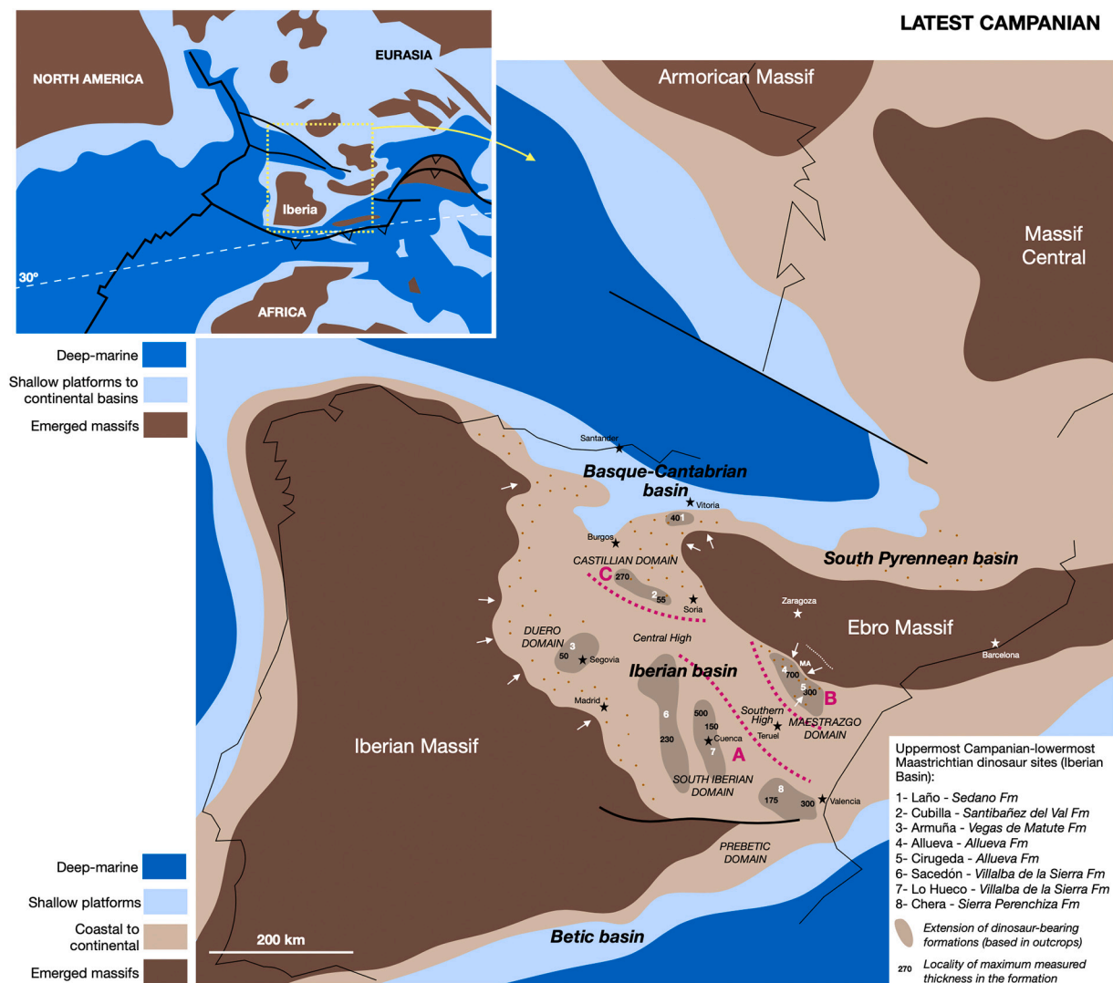
Fig. 14. Palaeogeography of Iberia at the end of the Campanian indicating the extension of the formations including upper Campanian–lowermost Maastrichtian fossil sites with titanosaur sauropods. Data mostly compiled from Floquet (1991), Alonso et al. (1993), García et al. (2004), Gil et al. (2010), Gómez-Gras et al. (2016), Vacherat et al. (2017), and Martín-Chivelet et al. (2019a). The inset in the upper left have been modified from Barrier et al. (2018). Notice that the dinosaur-bearing formations cover different chronostratigraphic intervals (see Fig. 15). White arrows indicates the source areas for terrigenous input. The white dashed line in the Ebro massif shows the northern extension of the post-rift Cenomanian-Santonian outcrops (see Aragües et al., 1981) previous to the uplift of the Montalbán anticline (MA). Three zones A-B-C (in purple) had different subsidence evolution in the Iberian basin (see text for explanation). (For interpretation of the references to colour in this figure legend, the reader is referred to the web version of this article.)
