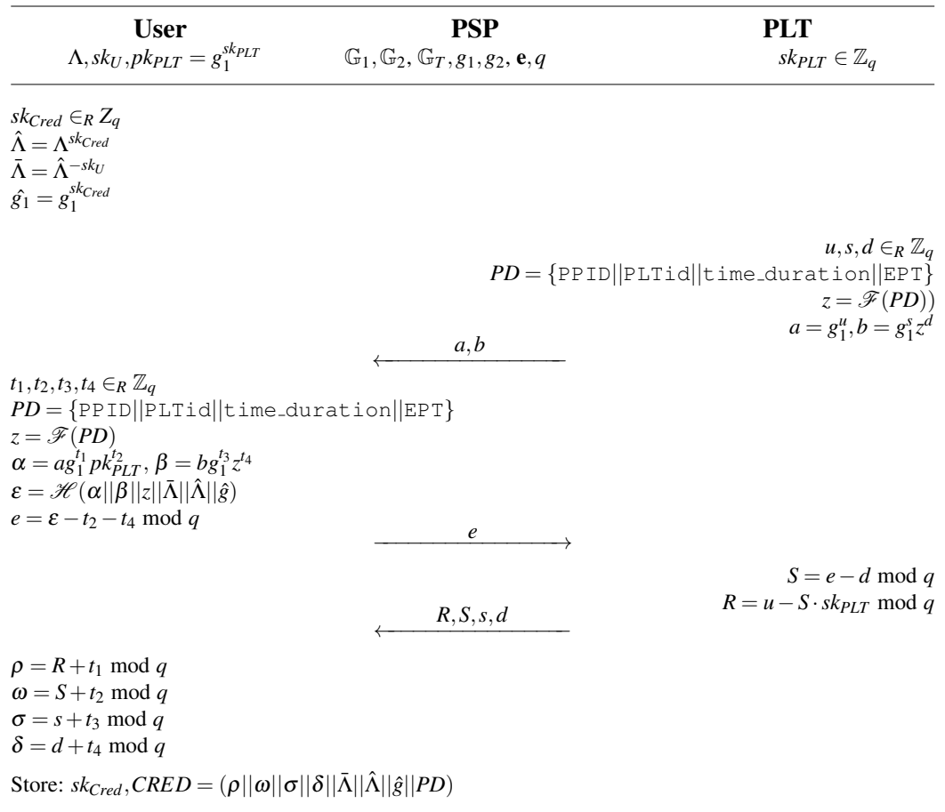
Figure 8 Issue algorithm.
