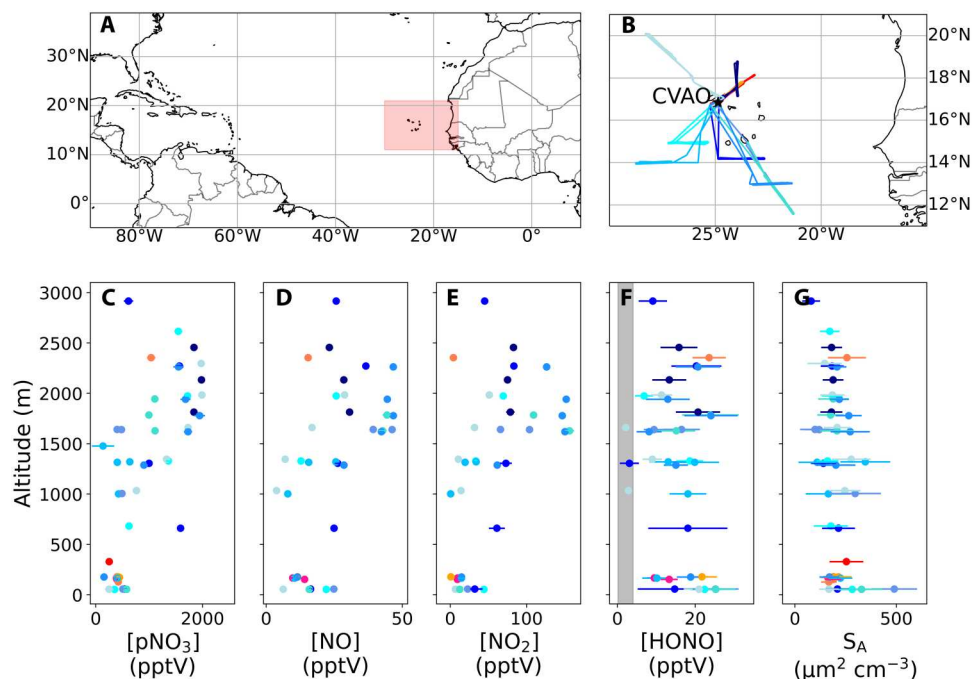
Fig. 1. Flight tracks and vertical profiles of \text{pNO}_3^- , NO, \text{NO}_2 , HONO, and aerosol surface area during ARNA-1 (August 2019) and ARNA-2 (February 2020). (A) Map over the region, where the red box is the area shown in (B). (B) Flight tracks from ARNA-1 in red colors and ARNA-2 in blue colors, alongside the location of the CVAO. The vertical profiles of (C) \text{pNO}_3^- , (D) NO, (E) \text{NO}_2 , (F) HONO, and (G) aerosol surface area are colored by their respective flight tracks as shown in (B). Each data point is an average of an SLR. The gray vertical line in (F) shows the range of calculated HONO gas-phase source-only concentrations for each SLR during the flights. The error bars represent the 1\sigma uncertainties described in Supplementary Text.
