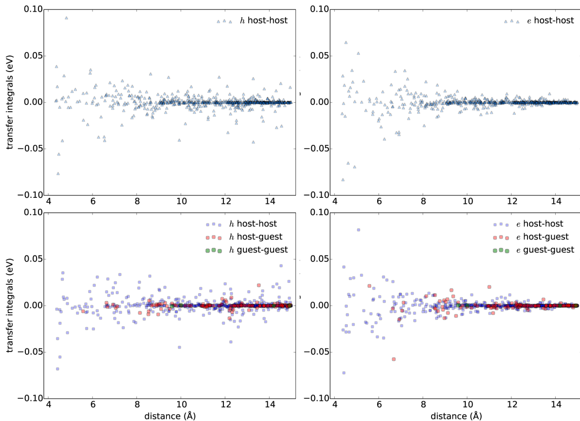
Figure 5. Transfer integral ( J_{ij}^c , see text) as a function of the separation between the centers of mass for holes (left) and electrons (right), in the pure host (top) and host-guest structure (bottom).
