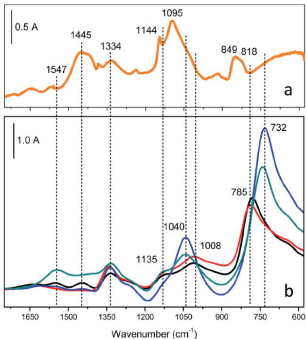
Fig. 5 FTIR absorbance spectra of PVA in KBr (section a) and mono-metallic Ru/ZrO 2 (black curve), bimetallic AuRu/ZrO 2 (red curve), AuRu/Y ZrO 2 (blue curve) and AuRu/La ZrO 2 (cyan curve) catalysts collected upon outgassing at 100 °C for 30 minutes (section b). The spectra in section b have been normalized on the weights of the pellets.
