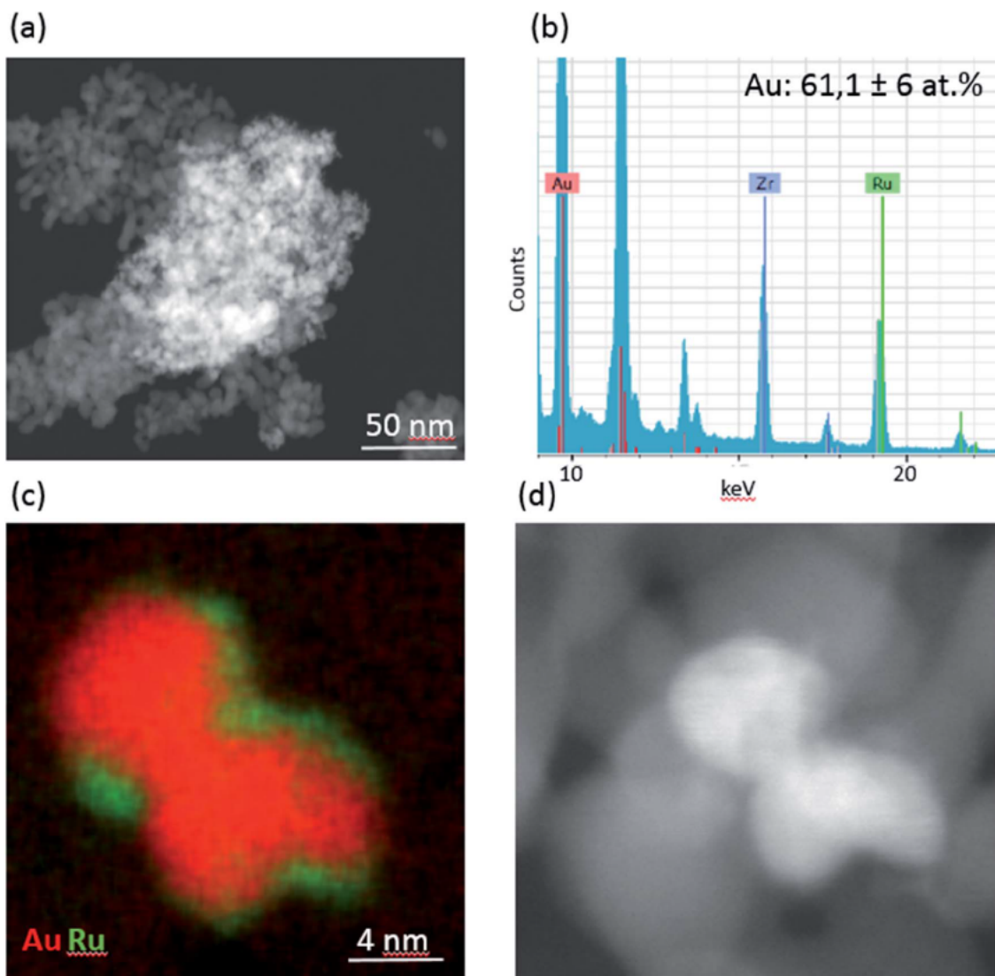
Fig. 4 HAADF-STEM overview image of the AuRu/ZrO 2 sample (section a), EDX spectra of the Au-L \alpha and Ru-K \alpha lines (section b), giving a mean Au concentration of 61.1 ± 6 at% (measurement of 10 different NP aggregates with a size of approximately 100 nm), quantified EDXS mapping (section c; Au, red and Ru, green), showing the Ru NPs on top of the Au NP, and the corresponding HAADF image (section d).
