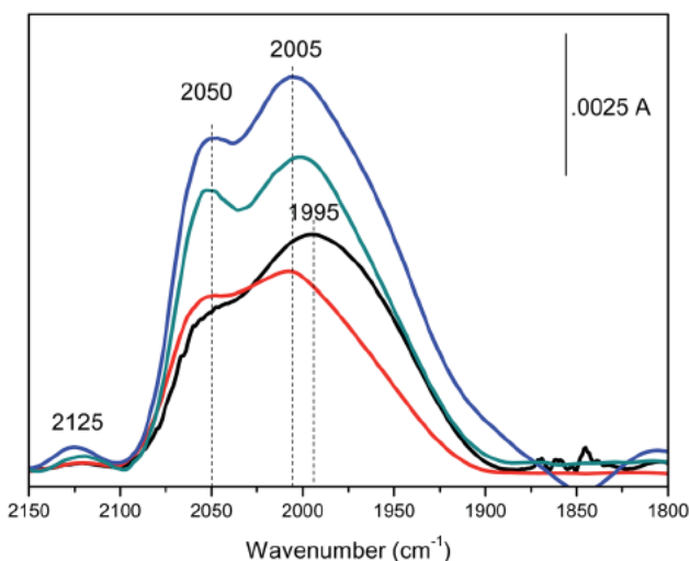
Fig. 6 FTIR difference spectra collected upon the adsorption of 15 mbar CO at RT and subsequent outgassing at RT on monometallic Ru/ZrO 2 (black curve) and bimetallic AuRu/ZrO 2 (red curve), AuRu/Y ZrO 2 (blue curve) and AuRu/La ZrO 2 (cyan curve) catalysts. The spectra have been normalized on the weights of the pellets.
