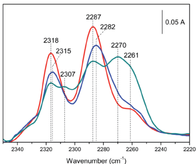
Fig. 9 FTIR difference spectra collected upon the adsorption of 2 mbar \text{CH}_3\text{CN} at RT on bimetallic AuRu/ZrO 2 (red curve), AuRu/Y-ZrO 2 (blue curve) and AuRu/La-ZrO 2 (cyan curve) catalysts. The spectra have been normalized on the weights of the pellets and on the specific surface areas of the supports.
