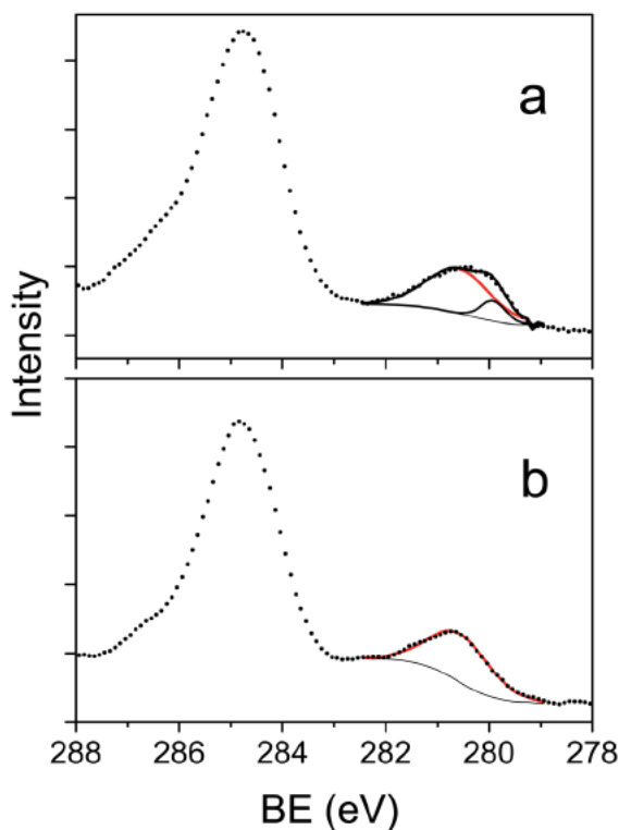
Fig. 8 Ru 3d XP spectra (circles) for the samples Ru/ZrO 2 (a) and Au Ru/ZrO 2 (b), along with the curve-fits. In both sections, the red line is the peak corresponding to the Ru n+ species, whereas in section (a) the peak of Ru 0 species is also reported as a black line.
