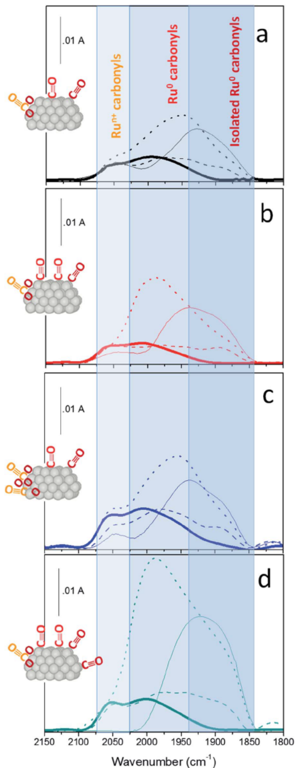
Fig. 7 FTIR difference spectra collected upon adsorption of 15 mbar CO at RT and subsequent outgassing at RT (bold curves), admission of 2-propanol (5 mbar) at RT (dashed curves), thermal treatment at 100 °C in a 2-propanol atmosphere (fine curves) and further admission of CO (15 mbar) at RT after preliminary outgassing at the same temperature (dotted curves) on monometallic Ru/ZrO 2 (section a) and bimetallic AuRu/ZrO 2 (section b), AuRu/Y-ZrO 2 (section c) and AuRu/La-ZrO 2 (section d) catalysts. Sketches of the different Ru carbonyls are displayed in each section.
