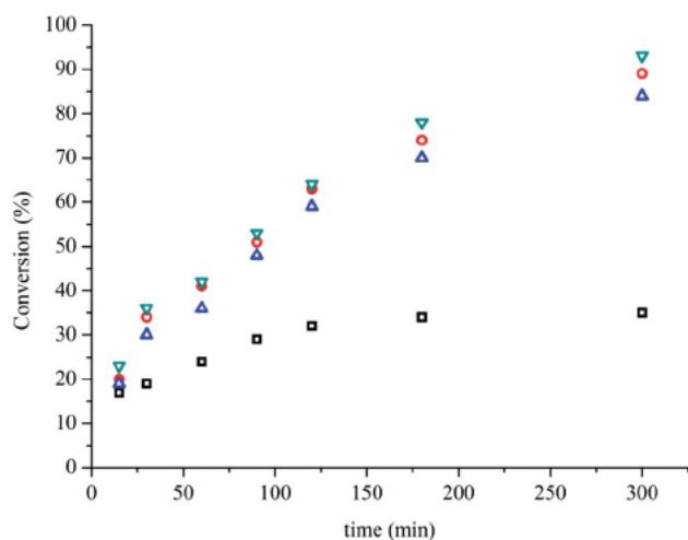
Fig. 1 Reaction profile for monometallic Ru/ZrO 2 (black squares), bimetallic AuRu/ZrO 2 (red circles), AuRu/Y ZrO 2 (blue triangles) and AuRu/La ZrO 2 (cyan triangles) catalysts.
