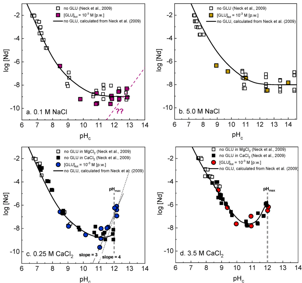
Fig. 2. Solubility of \text{Nd}(\text{OH})_3(\text{s}) in the presence of [\text{GLU}]_{\text{tot}} = \text{constant} = 10^{-3} \text{ M} and (a) 0.1 M NaCl; (b) 5.0 M NaCl; (c) 0.25 M \text{CaCl}_2 ; (d) 3.5 M \text{CaCl}_2 . Empty symbols in the figures correspond to solubility data determined under analogous conditions but absence of gluconate (Neck et al., 2009). Solid lines represent the solubility of \text{Nd}(\text{OH})_3(\text{s}) in the absence of gluconate calculated with the thermodynamic and SIT activity models reported in Neck et al. (2009).
