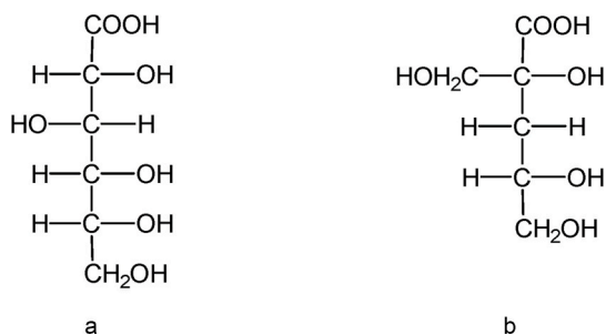
Fig. 1. Chemical formula of (a) D-gluconic acid ( C_6H_{12}O_7 , HGLU) and (b) \alpha -Isosaccharinic acid ( C_6H_{12}O_6 , HISA).
