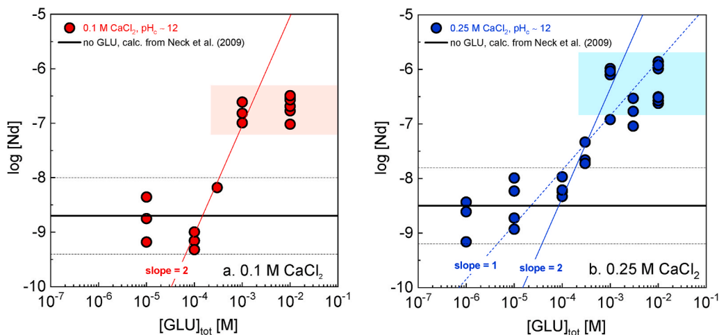
Fig. 3. Solubility of \text{Nd}(\text{OH})_3(\text{s}) at \text{pH}_c \approx 12 in the presence of 10^{-6} \text{ M} \leq [\text{GLU}]_{\text{tot}} \leq 10^{-2} \text{ M} and (a) 0.1 M \text{CaCl}_2 ; (b) 0.25 M \text{CaCl}_2 . Solid lines represent the solubility of \text{Nd}(\text{OH})_3(\text{s}) in the absence of gluconate calculated with the thermodynamic and SIT activity models reported in Neck et al. (2009).
