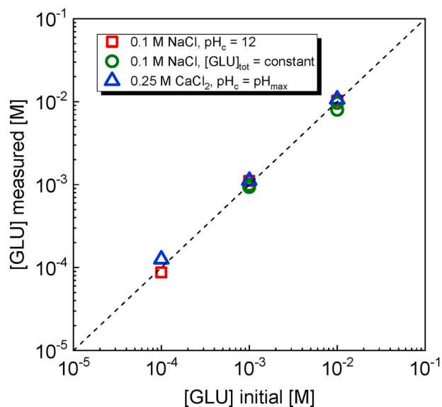
Fig. 4. Comparison of initially dissolved gluconate concentration with [\text{GLU}]_{\text{tot}} experimentally determined by TOC after equilibration with \text{Nd}(\text{OH})_3(\text{s}) in 0.1 M NaCl and 0.25 M \text{CaCl}_2 solutions. Series 0.1 M NaCl, \text{pH}_c = \text{constant} \approx 12 : [\text{GLU}]_{\text{ini}} = 10^{-2} , 10^{-3} and 10^{-4} M. Series 0.1 M NaCl, [\text{GLU}]_{\text{tot}} = \text{constant} : [\text{GLU}]_{\text{ini}} = 10^{-3} M, \text{pH}_c = 8.48, 9.80, 10.89, 11.87, 12.34, 12.86 ; [\text{GLU}]_{\text{ini}} = 10^{-2} M, \text{pH}_c = 10.86 . Series 0.25 M \text{CaCl}_2 , \text{pH}_c = \text{constant} = \text{pH}_{\text{max}} : [\text{GLU}]_{\text{ini}} = 10^{-2} M, \text{pH}_c = 12.01 ; [\text{GLU}]_{\text{ini}} = 10^{-3} M, \text{pH}_c = 12.17 , [\text{GLU}]_{\text{ini}} = 10^{-4} M, \text{pH}_c = 12.15 .
