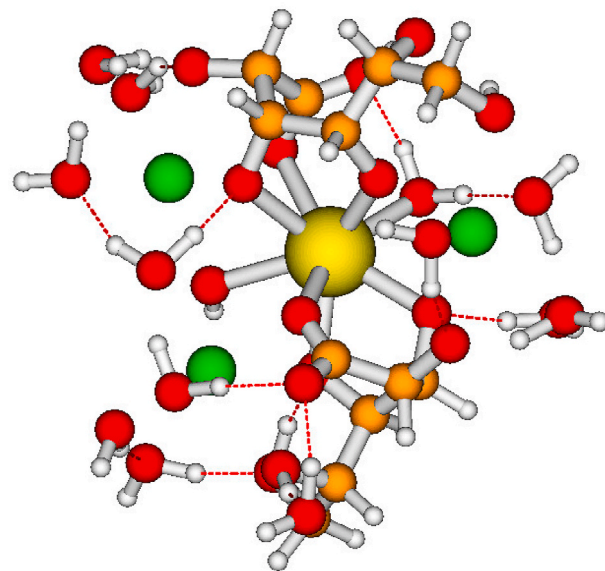
Fig. 9. Structure of the ternary complex Ca 3 NdOH(GLU ·3H ) 2 (aq) as optimized by DFT calculations. Colour code: Nd: yellow; Ca: green; O: red; C: orange; H: grey.
