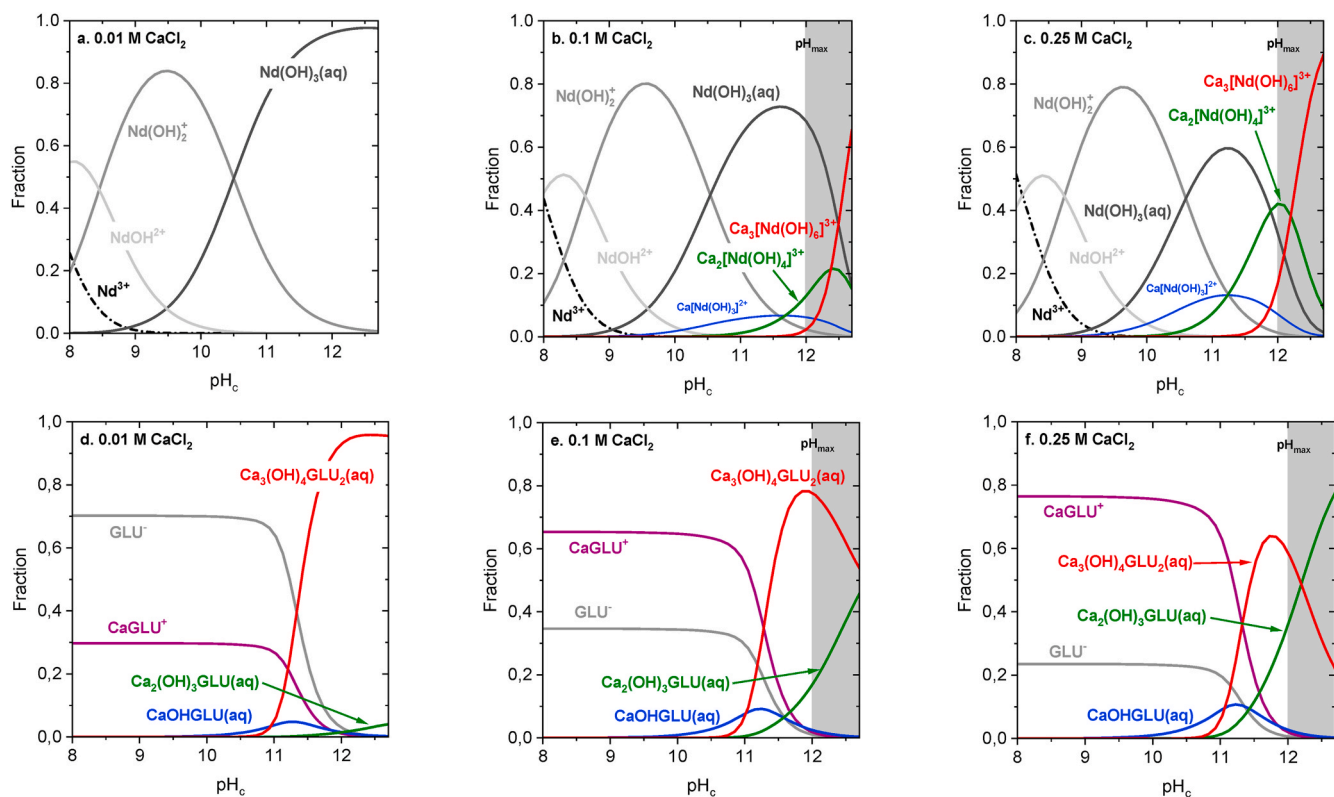
Fig. 8. Fraction diagrams of Nd(III) calculated for (a) 0.01 M CaCl 2 ; (b) 0.1 M CaCl 2 ; (c) 0.25 M CaCl 2 using thermodynamic data reported in Neck et al. (2009). Fraction diagrams of gluconate calculated for [GLU] tot = 10 -3 M and (d) 0.01 M CaCl 2 ; (e) 0.1 M CaCl 2 ; (f) 0.25 M CaCl 2 using thermodynamic data reported in Pallagi et al. (2014). pH c in 0.1 and 0.25 M CaCl 2 systems buffered to pH max ≈ 12 due to the precipitation of Ca(OH) 2 (shaded region in figures b, c, e and f).
