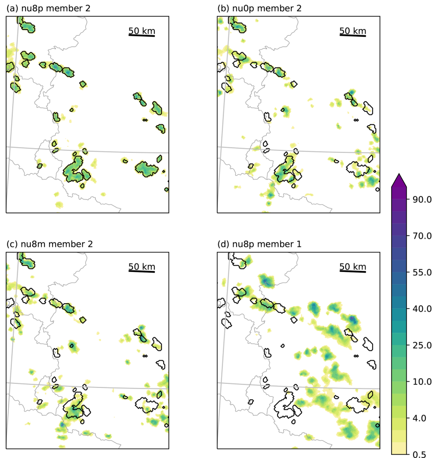
Figure 5. Snapshot of hourly precipitation at 16:00 UTC for the weak forcing case (11 August). Member 2 of IBC sub-ensembles (a) nu8p , (b) nu0p and (c) nu8m and (d) member 1 of nu8p in the central western part of Germany (see blue box in Fig. 2). Black contours indicate grid points that have a larger value than the 99th percentile value in the nu8p sub-ensemble of member 2. The red circle in (a) indicates single convective cells discussed in the text.
