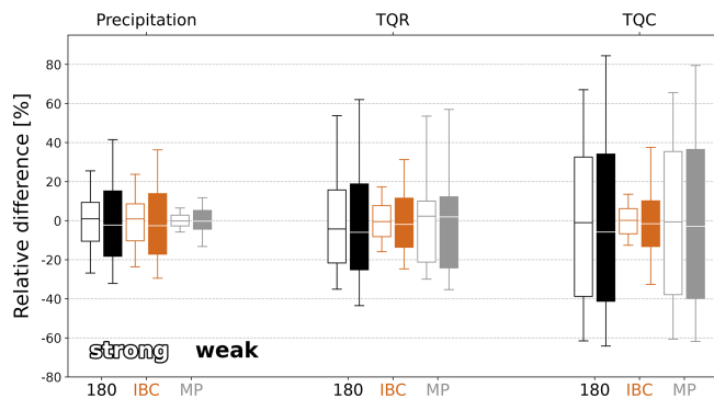
Figure 10. Relative differences in the 180-member ensemble (black), the averaged IBC sub-ensembles (orange) and averaged combined microphysical sub-ensembles (grey) aggregated over 5 d in August 2020 conditional on synoptic control. Relative differences in precipitation, total column rainwater content (TQR) and total column cloud water content (TQC) are displayed using filled boxes for weak forcing situations. Box plots show bootstrapped medians, interquartile ranges, and the 5th and 95th percentiles in that order. For details see the text.
