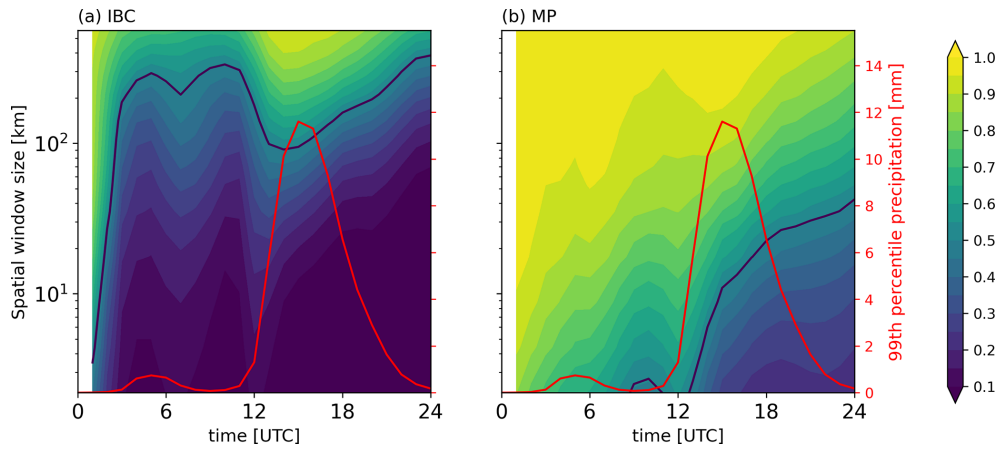
Figure 6. Ensemble mean FSS values of hourly precipitation calculated across scales ranging from 2 to 560 km in the German domain for the weak forcing case of 11 August. The IBC sub-ensembles’ mean FSS is depicted in panel (a) and the combined microphysics sub-ensembles’ mean FSS in panel (b). The black lines show believable scales of mean FSS. The red lines (right axis) show the time series of the mean 99th percentile value of hourly precipitation.
