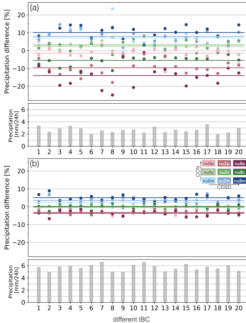
Figure 3. Relative difference in daily area-averaged precipitation (in %) with respect to combined microphysical (MP) sub-ensemble means sharing the same initial and lateral boundary conditions (IBC) for the (a) weak and (b) strong forcing cases. The columns below indicate absolute precipitation values of the 20 different MP sub-ensemble means. The nine colours indicate all combinations of microphysical configurations (as in Fig. 1a). The coloured lines show the averages.
