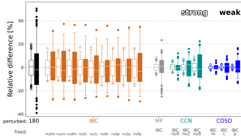
Figure 4. Box and whisker diagram showing the relative differences of daily area-averaged precipitation of individual ICON-D2 members belonging to various (sub-)ensembles. The perturbations ( x labels in colour) and different fixed configurations (grey x labels) are indicated. 180 is the abbreviation of the entire ensemble and IBC, MP, CCN and CDS are for the different sub-ensembles. The bars, boxes, whiskers and dots show medians, interquartile ranges, 5th and 95th percentiles, and outliers, respectively. Filled boxes represent weak control (11 August) and open boxes strong synoptic control (17 August).
