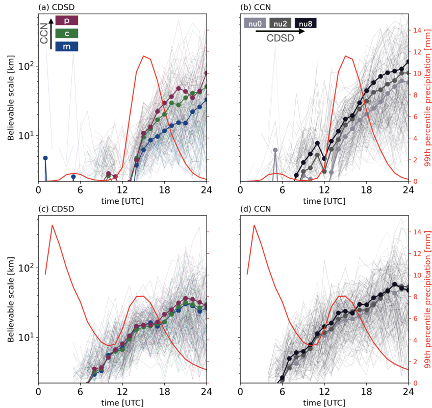
Figure 8. Time series of FSS believable scales of hourly precipitation for every combination of (a) the CDS and (b) CCN sub-ensemble for the weak forcing case in the German domain. In (a) blue, green and red lines indicate simulations with maritime, continental and polluted CCN content, respectively. In (b) light grey, dark grey and black lines indicate scales with the broad, intermediate and narrow CDS. Bold lines with circles indicate mean values of FSS believable scales sharing the same perturbation. The red lines (right axis) show time series of the mean 99th percentile value of hourly precipitation. Panels (c) and (d) show the results for the strong synoptic forcing case.
