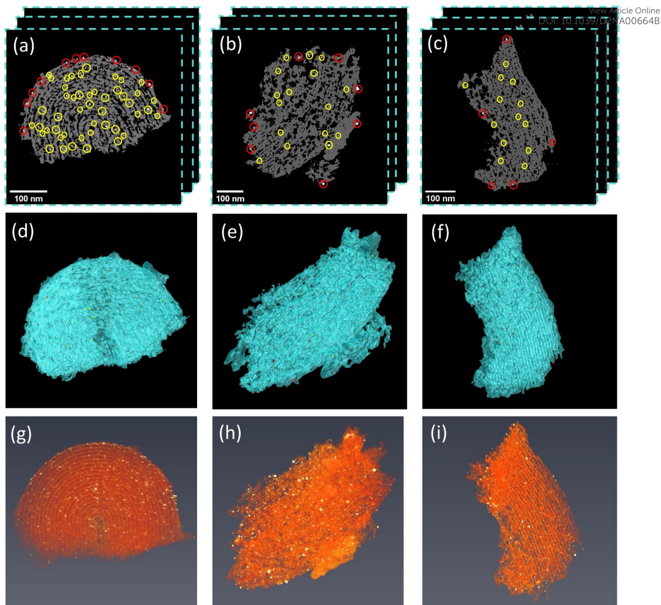
Figure 6. Typical 2D slices from the reconstructed volume of Pd@CMK3 (a) before and after FA decomposition reaction (b) in batch reactor and (c) in fixed bed reactor; The corresponding (d–f) surface renderings and (g–i) volume rendering. The red and yellow circles in a–f highlight Pd nanoparticles on internal and external support surface.
