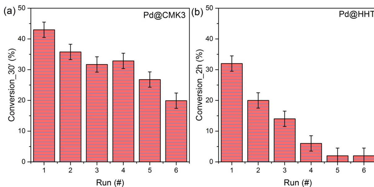
Figure 3. Stability test during FA decomposition with a similar initial conversion: (a) Pd@CMK3 after 30 minutes of reaction time and (b) Pd@HHT after 2 hours of reaction time.
