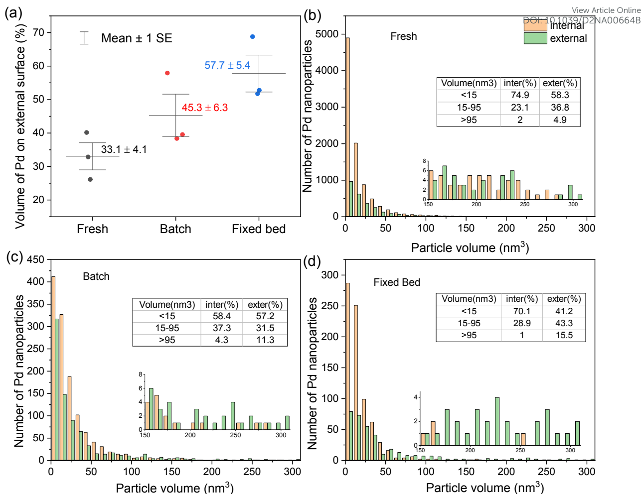
Figure 7. (a) The fraction of Pd NPs on the external surface for the fresh and used catalysts; number of particles distributed on the internal and external support surface of Pd@CMK3 in the (b) fresh state, (c) after reaction in the batch reactor and (d) after reaction in the fixed bed reactor. The inserted tables in b-d show the relative volume of Pd NPs with a certain volume range on the internal and external surface. The inserted histograms are closeup views of the limited data of particles with volume larger than 150 nm 3 .
