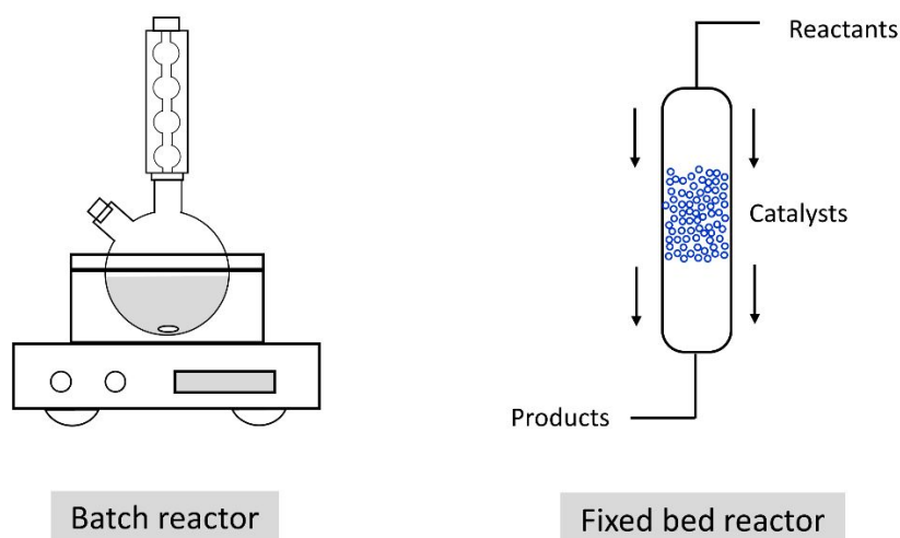
Figure 1. Schematic diagram of a typical lab-used batch and fixed bed reactor.
