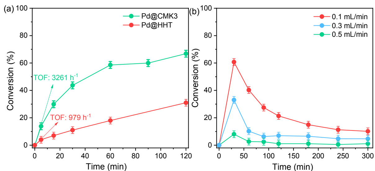
Figure 2. Catalytic performance of Pd@CMK3 and Pd@HHT (from [33]) during FA decomposition. (a) FA conversion as a function of reaction time on Pd@CMK3 and Pd@HHT
