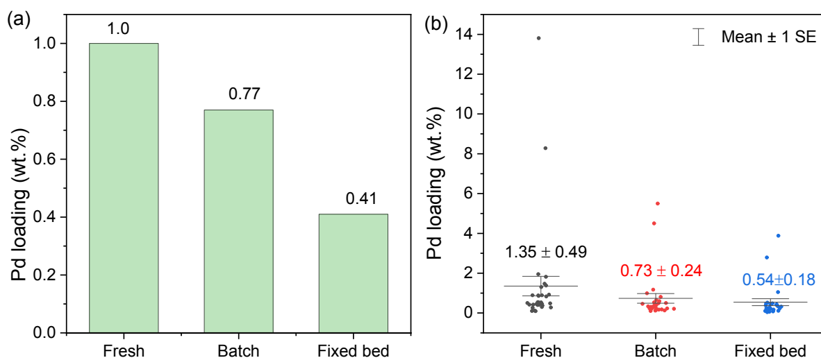
Figure 5. Pd loading of Pd@CMK3 catalysts measured by (a) ICP-AES and (b) EDX based on around 30 regions of interest for each catalyst. SE in EDX data represents standard error, a standard deviation (Std.) of the sampling distribution of a statistic. SE = Std./\sqrt{n} , n is sample observations.
