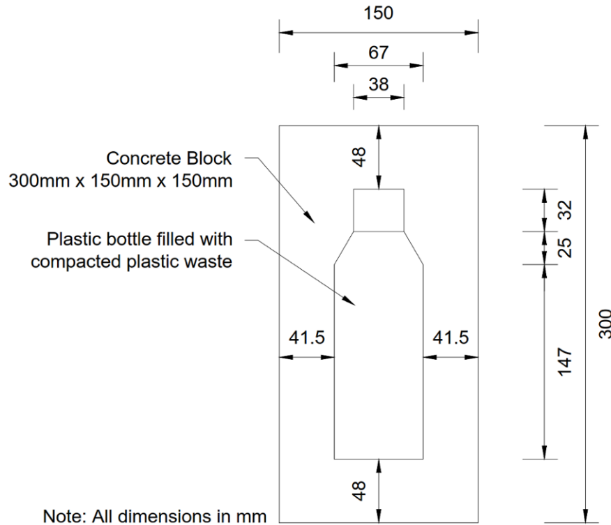
Fig. 3. Proposed Concrete Encased Ecobrick Design.
