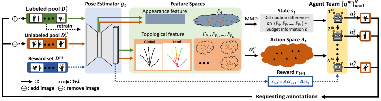
Figure 1. Overview of our MATAL framework for hand pose estimation (MATAL for human body pose estimation shares the similar structure). The solid lines describe the data flow at the t^{\text{th}} active learning iteration and dot lines are that of the (t+1)^{\text{th}} iteration. Given a labeled sample pool D_t^L and an unlabeled sample pool D_t^U , our active learning framework works as follows: 1) We first project both the D_t^U and D_t^L to the feature spaces with the pose estimator g_t , then construct the state s_t and action space A_t from the feature spaces. The state s_t records the differences between D_t^U and D_t^L in the feature spaces, and the consumption of annotation budget. The action space A_t contains the projection of D_t^U in the feature spaces. Each action a_t \in A_t corresponds to a unique image in D_t^U and describes the novelty, representativeness and appearance of the image. 2) The agent team follows the Q -learning [45] framework and evaluates the state-action pair (s_t, a_t) to determine a set of actions \{a_t^m\}_{m=1}^N of raising corresponding images for annotation. 3) We then update D_{t+1}^U and D_{t+1}^L by moving new annotated images from D_t^U to D_t^L . The pose estimator is retrained on D_{t+1}^L to obtain g_{t+1} . 4) The reward r_{t+1} , which measures the improvement of pose estimator’s prediction accuracy on D^{re} as Acc_{t+1} - Acc_t , is used to optimize the agent team.
