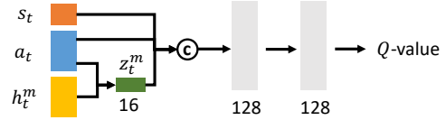
Figure 2. The architecture of the m^{th} agent in the team. Note that each agent shares the similar model architecture but with its own parameters. a_t and h_t^m are first fed into a linear layer with ReLU activation to generate feature z_t^m \in \mathbb{R}^{16} . z_t^m , a_t and s_t are then concatenated and passed through three linear layers with ReLU activation in between to output the Q -value.
