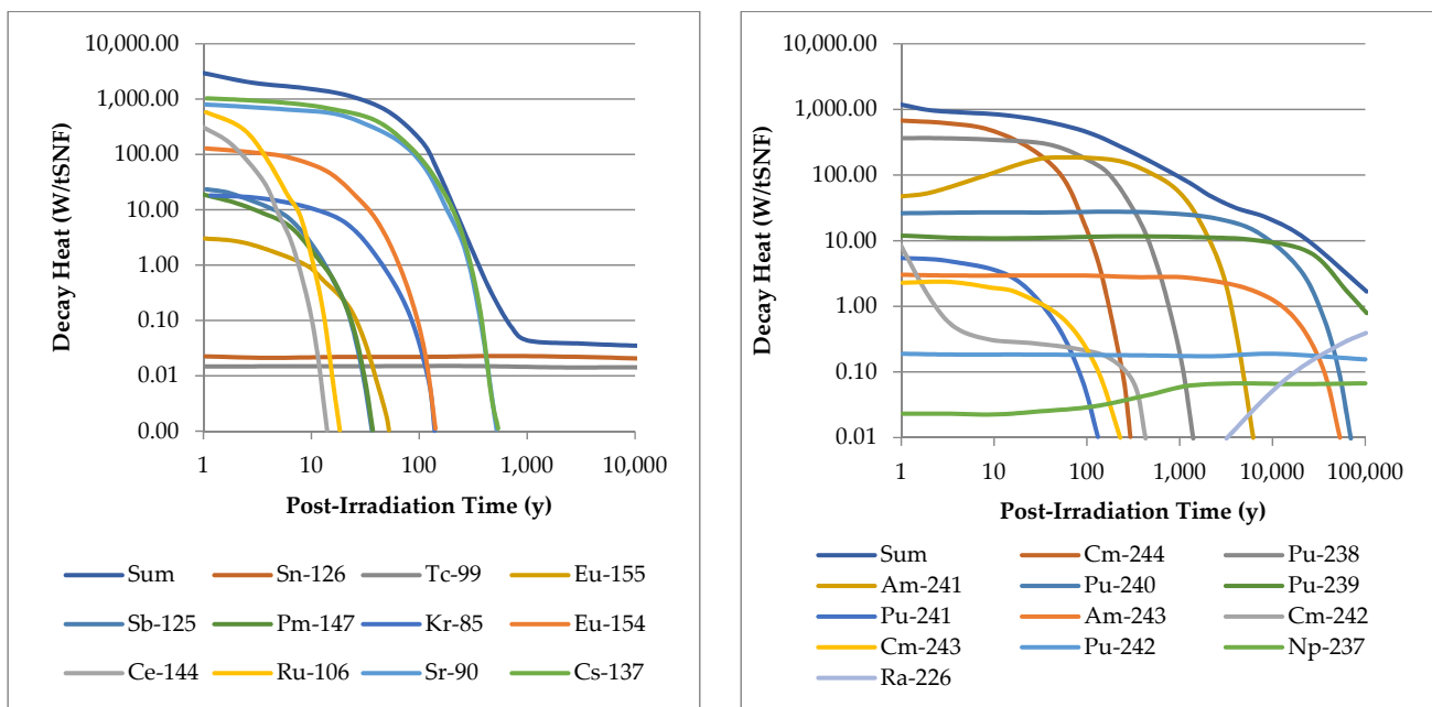
Figure 3. Sources of decay heat for HBU PWR (VVER) fuel with time from primary fission product ( left ) and actinide ( right ) isotopes. Graphical data extracted from reference [32]. NB: axes are logarithmic scale.
