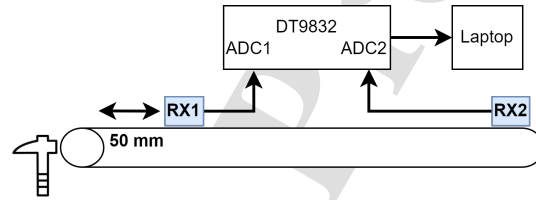
Figure 4: Experimental setup for hammer hit (ToF) measurement.
