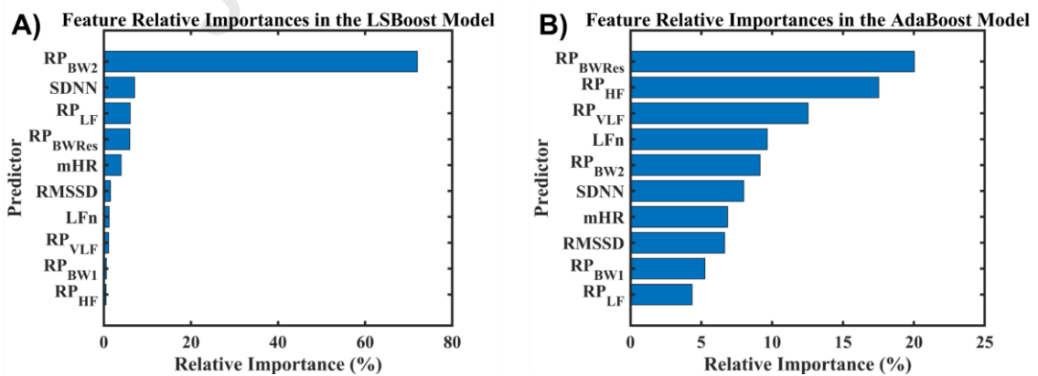
Figure 7. Feature importance for both the LSBoost and AdaBoost models. A) Relative importance of the ten features through the tree base classifiers in the LSBoost Model. B) Relative importance of the ten features included in the AdaBoost Model, computed using LIME.
