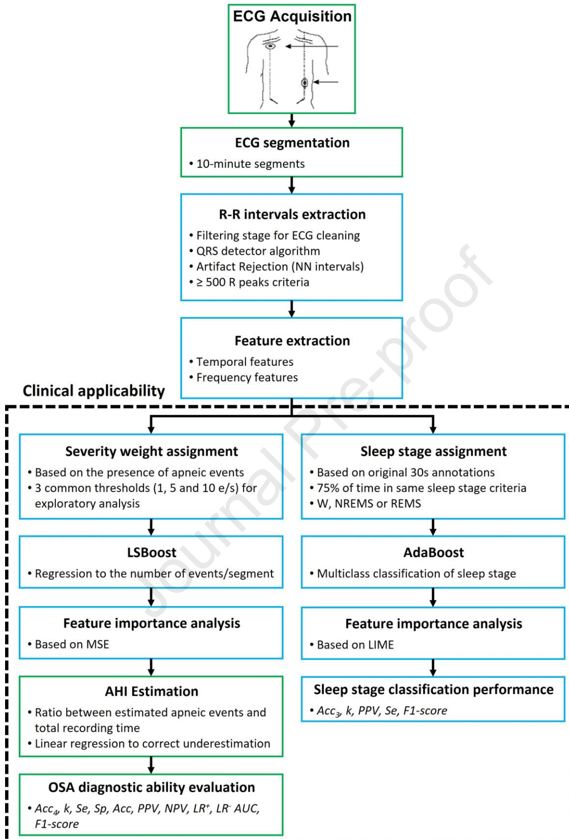
Figure 1. Flowchart of the protocol followed across the study from the ECG acquisition to the evaluation of the clinical applicability of the characterization of HRV segments following two approaches: OSA diagnostic ability (left branch) and sleep stage classification (right branch). Green boxes means that the corresponding stage of the protocol was applied per subject. Blue boxes means that it was a segment-level stage.
