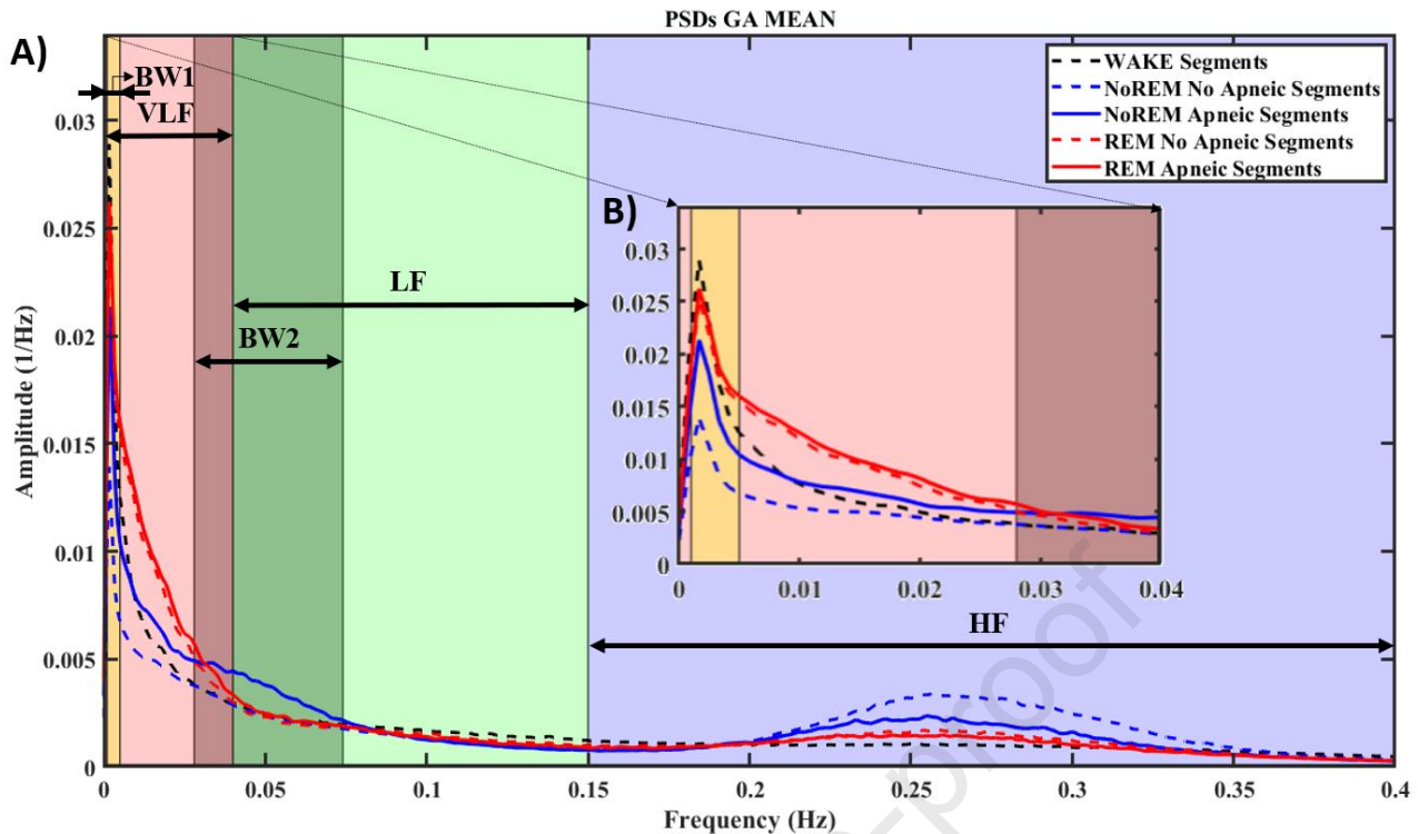
Figure 2. A) Averaged PSDns in the 0-0.4 Hz range for five types of segments in the training set. Shaded areas represent those frequencies corresponding with the three classic spectral HRV bands (VLF: 0-0.04 Hz; LF: 0.04-0.15 Hz; HF: 0.15-0.4 Hz) and two of the pediatric OSA-specific frequency bands (BW1: 0.001-0.005 Hz; BW2: 0.028-0.074 Hz). B) Zoomed area in the VLF range.
