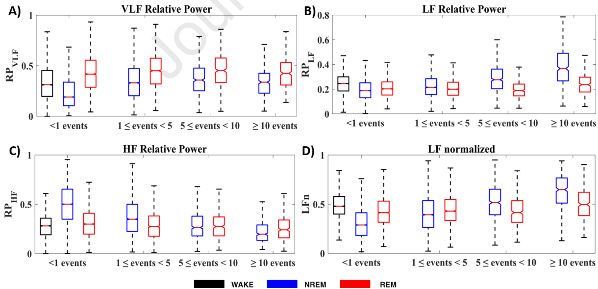
Figure 4. Boxplot distribution of the frequency features in the classic HRV frequency bands computed for each type of segment included in the study in the training set. A) RP_{VLF} boxplots; B) RP_{LF} boxplots; C) RP_{HF} boxplots; D) LFn .
