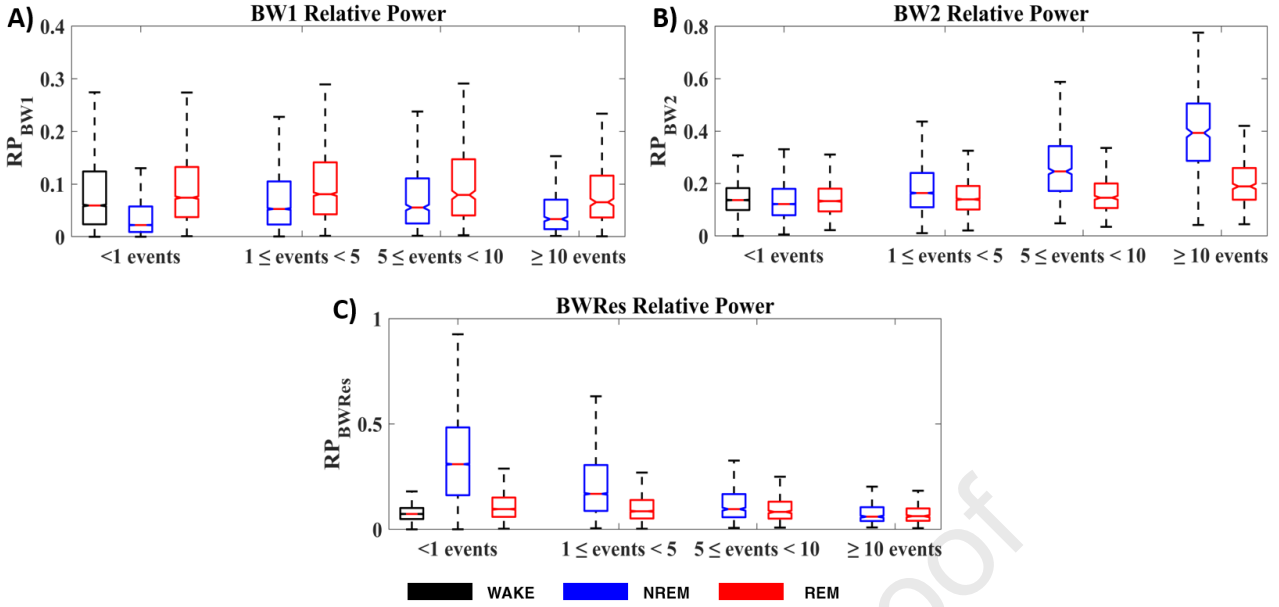
Figure 5. Boxplot distribution of the frequency features in the pediatric OSA-specific HRV frequency bands computed for each type of segment included in the study in the training set. A) RP_{BW1} boxplots; B) RP_{BW2} boxplots; C) RP_{BWRes} boxplots.
