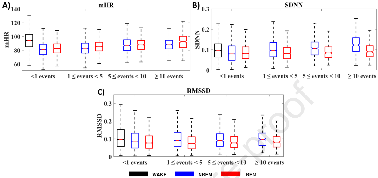
Figure 3. Boxplot distribution of the temporal features computed for each type of segment included in the study in the training set. A) mHR boxplots; B) SDNN boxplots; C) RMSSD boxplots.
