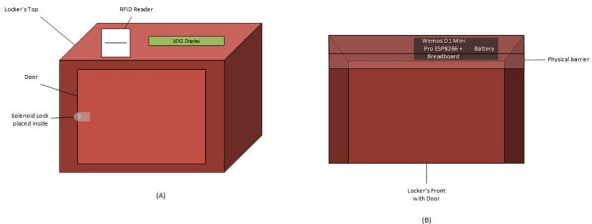
Fig. 3. Prototype 3D Model.
