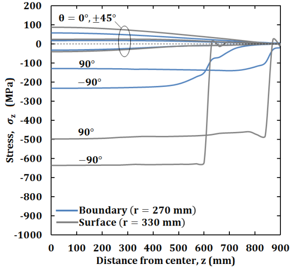
Figure 6 (A) Bimetallic work roll surface r = 330 mm and the HSS/DCI boundary r = 270 mm focusing on the lines \theta = -90^\circ, -45^\circ, 0^\circ, 45^\circ, 90^\circ , (B) stress \sigma_r , (C) stress \sigma_\theta , (D) stress \sigma_z when P/P_{\text{total}} = 1.0
