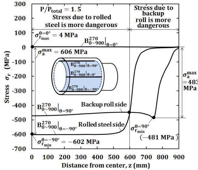
Figure 11 Rolling stress \sigma_r at \theta = 0^\circ , \theta = 90^\circ and \theta = -90^\circ along z -direction on the boundary r = 270 mm of the work roll when P/P_{\text{total}} = 1.5
