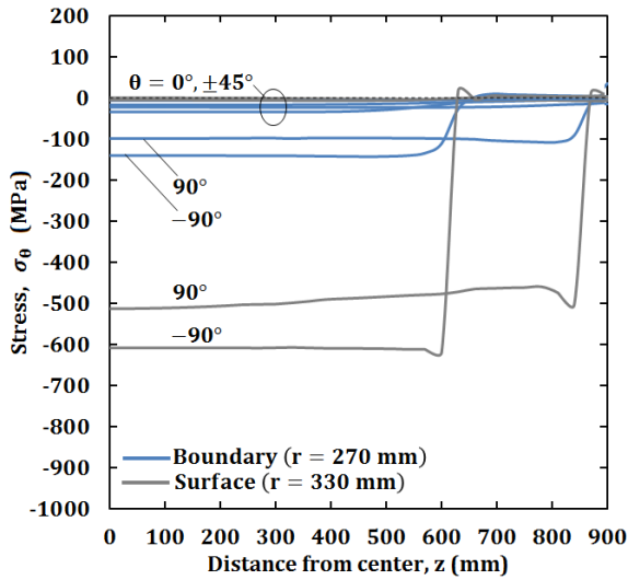
(A) Work roll surface and HSS/DCI boundary focusing on the lines \theta = -90^\circ, -45^\circ, 0^\circ, 45^\circ, 90^\circ
