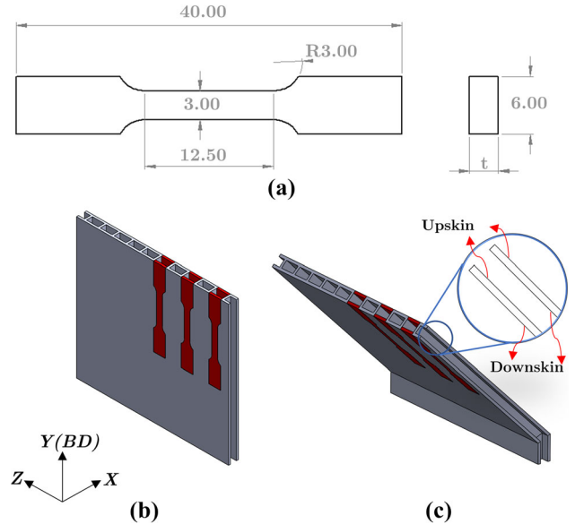
Fig. 1—(a) Dimensions of miniature tensile specimens. All dimensions are in mm, (b) Extraction of tensile specimens from the part fabricated with 90 deg build angle, (c) Extraction of tensile specimens from the part fabricated with 45 deg build angle. BD is build direction.
