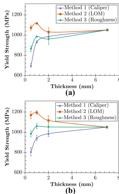
Fig. 14—Yield strength (YS) from Method 1, Method 2, and Method 3 for build angle of (a) 90 deg and (b) 45 deg.
