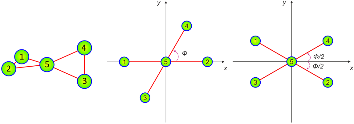
Figure 1: Equilibrium structure of the \text{H}_5^+ molecular ion (left panel) and definitions of the geometric (GE, middle panel) and bisector (BE, right panel) embeddings, whereby \phi corresponds to the torsional coordinate.
