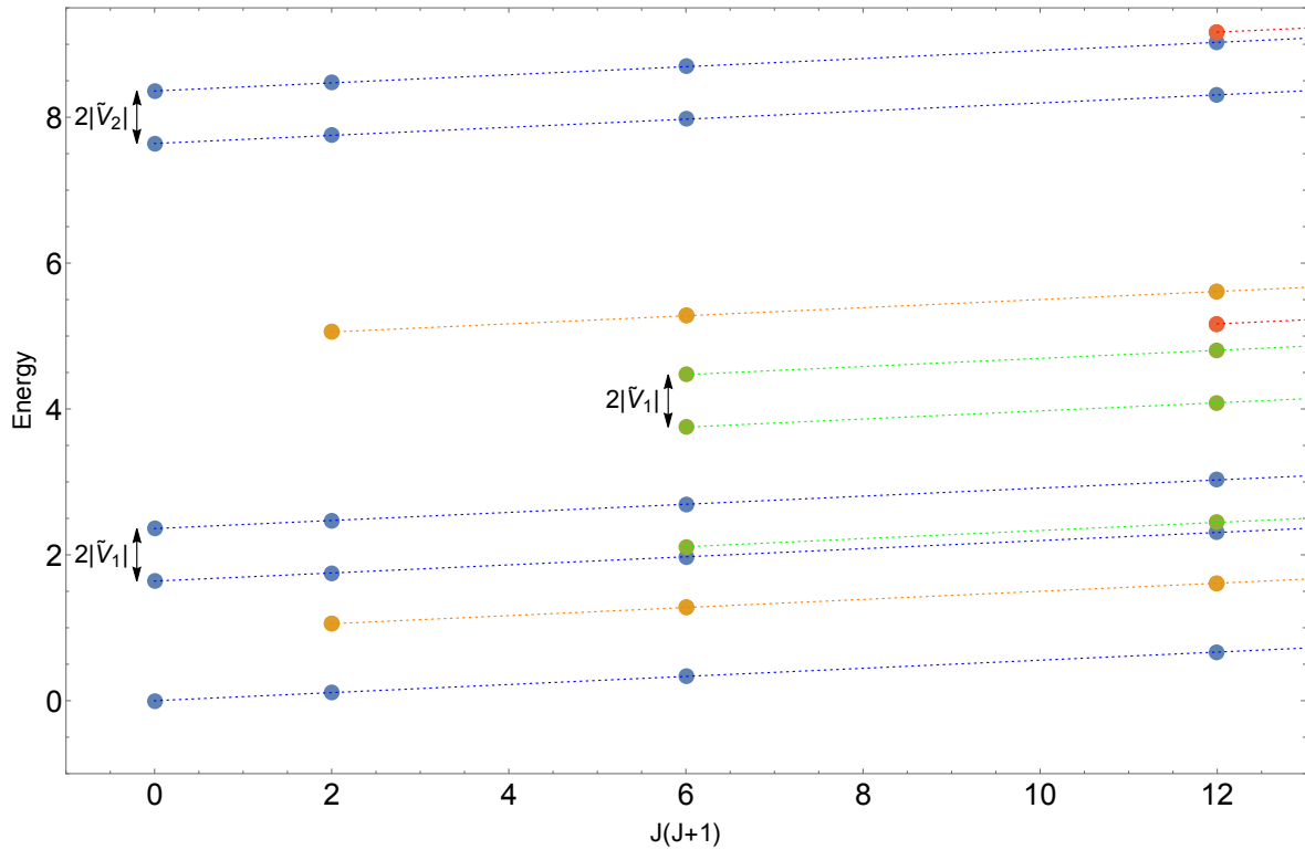
Figure 2: Symmetric-top states incorporating torsional splitting. The K = 0 states (blue points) are non-degenerate, the |K| = 1 states (orange points) are quadruply degenerate, the |K| = 2 states (green points) are doubly degenerate and the |K| = 3 states (red points) are quadruply degenerate. The dotted lines all have gradient 1/2R^2 to illustrate that the effect of increasing J on the energy levels is simply to translate the energies (as well as allowing more possibilities for K = -J, \dots, +J ). Level splittings due to the torsional potential are indicated with arrows.
