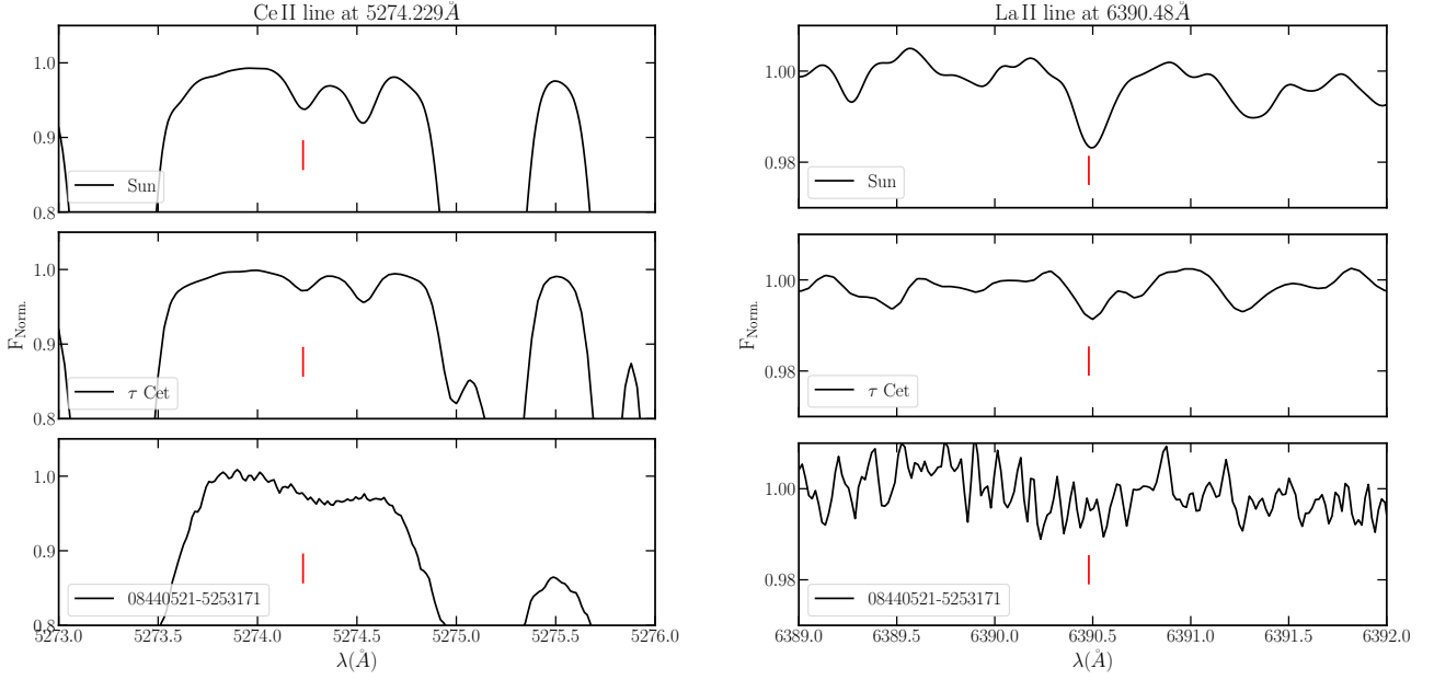
Fig. 1: Comparison of spectra of the Sun (top), \tau Cet (central), and the star 08440521-5253171 of IC 2391 (S/N=260) in two spectral regions. Shown on the left a 3 Å window around the Ce II line 5274.23 Å, while on the right a region near the La II line at 6390.48 Å.
