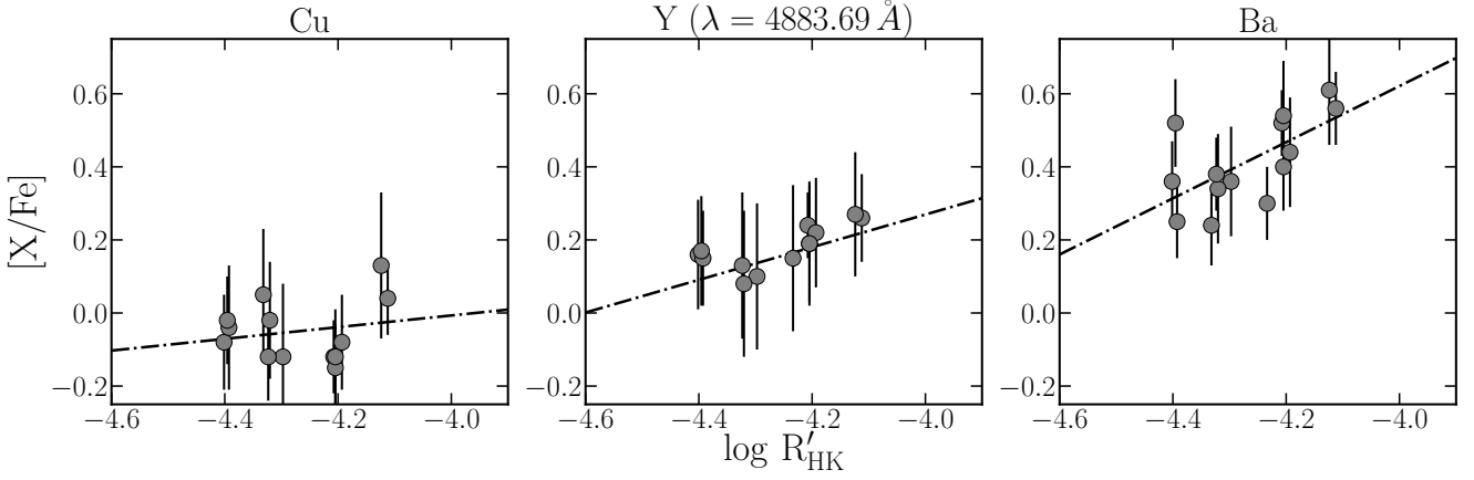
Fig. 6: [X/Fe] as a function of \log R'_{HK} , computed following Mamajek & Hillenbrand (2008) from the \log(L_X/L_{bol}) (details on the computation can be found in Paper I). The dot-dashed lines are the linear fits of the measurements.
