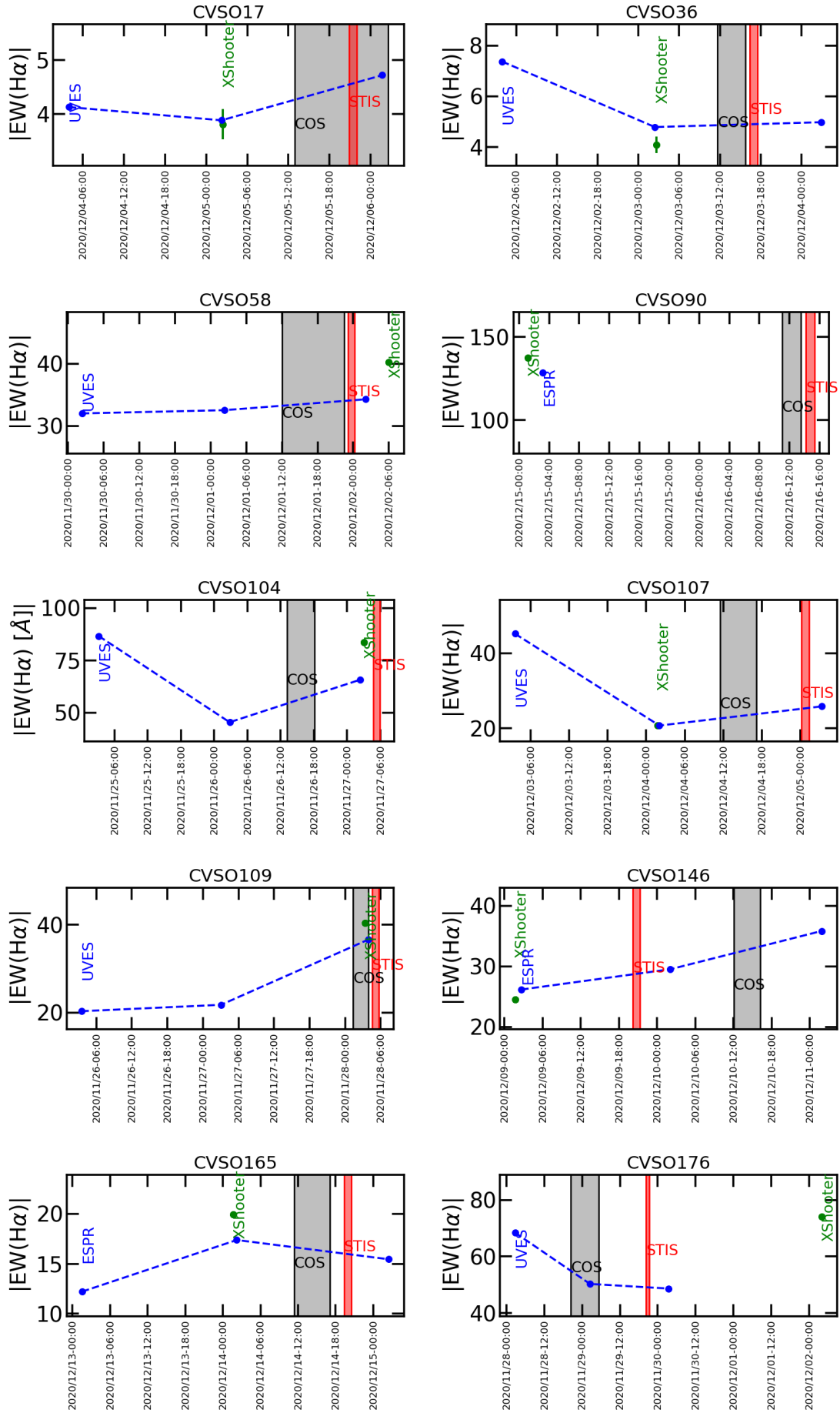
Fig. B.1. Variability of the H\alpha equivalent width for the Orion OB1 targets as measured by EPRESSO or UVES (blue) and X-Shooter (green), together with the timing of the COS (grey) and STIS (red) HST observations.
