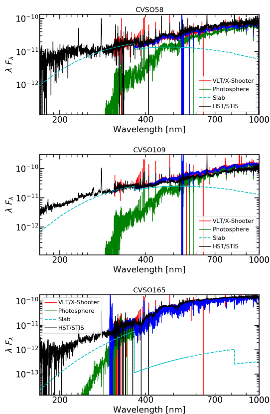
Fig. 13. Comparison of the extrapolation of the results obtained fitting the VLT/X-Shooter spectrum (best fit in blue) with the HST spectrum in the UV.
