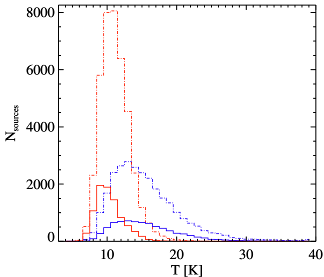
Figure 16. Distributions of MBB temperature for pre-stellar (red histograms) and protostellar (blue histograms) sources. Dot-dashed histograms are for the inner Galaxy and solid for the outer.
