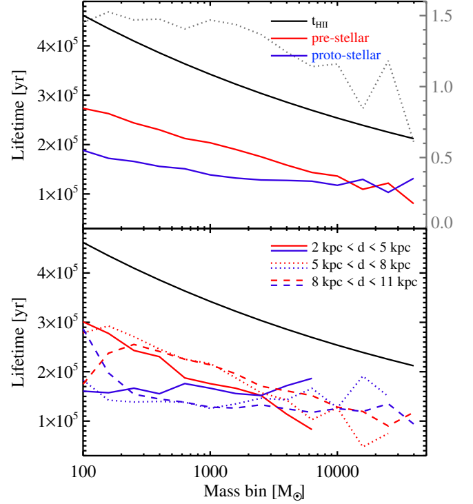
Figure 14. Lifetimes vs mass. The black line in each panel represents the mass dependence of the lifetime t_{\text{HII}} for a clump hosting an H II region according to \log(t_{\text{HII}}/\text{yr}) = -0.13 \times \log(L/L_{\odot}) + 6.1 ( Mottram et al. 2011 ) and assuming L_{\text{bol}}/M = 22.4 L_{\odot}/M_{\odot} . By definition t_{\text{HII}} is the sum of the lifetimes of the pre-stellar and protostellar phases, and so these lifetimes can be derived from the relative populations of these phases in each bin of mass (see the text). The numeric ratio of pre-stellar to protostellar clumps is also plotted as a dotted grey line, referring to the grey y-axis on the right. Top : lifetimes of pre-stellar (red line) and protostellar (blue line) clumps for the entire sample. Bottom : same as the top, but dividing the clumps into three different ranges of heliocentric distance: 2-5 kpc (solid lines), 5-8 kpc (dotted lines), and 8-11 kpc (dashed lines).
