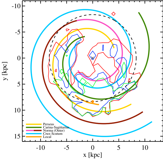
Figure 3. The same as Figure 2, but with source density contours displayed instead of source positions. Sources are counted in boxes of 1 \text{ kpc}^2 . To avoid figure crowding, only one contour, corresponding to a level of 100 \text{ sources kpc}^{-2} is plotted for each source class: green for starless unbound sources (not shown in Figure 2), red for pre-stellar, and blue for protostellar, respectively.
