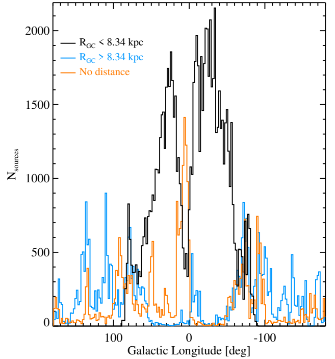
Figure 4. Histograms in 2^\circ -bins of Galactic longitude of Hi-GAL sources located inside the Solar circle (black), outside (light blue), and lacking a distance/Galactocentric radius estimate (orange), respectively.
