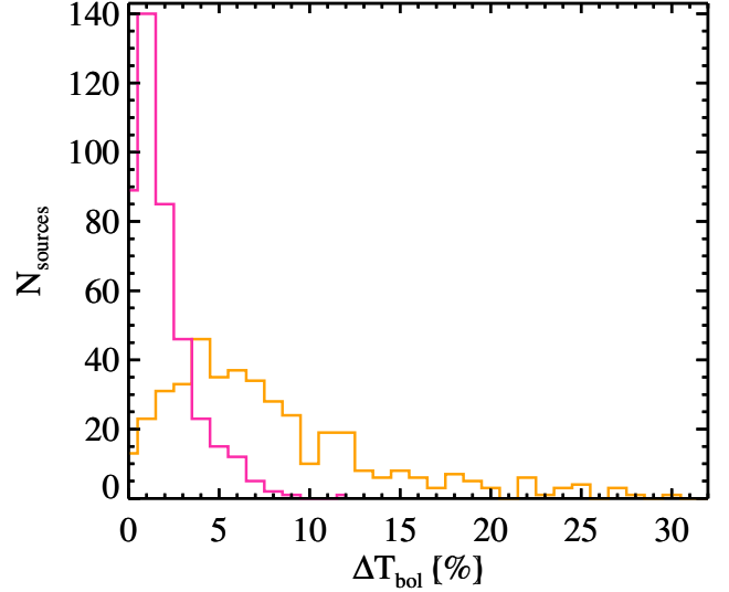
Figure B2. Distributions of the percentage increase of T_{\text{bol}} for relatively faint ( F_{70} < 2 Jy) and MIR-dark Hi-GAL sources produced by extending their SED with a MIR flux at the corresponding survey completeness limit (cf. Fig. B1): MIPSGAL, F_{24} = 0.03 Jy at 24 \mu\text{m} (magenta) and WISE, F_{22} = 0.1 Jy at 22 \mu\text{m} (orange).
