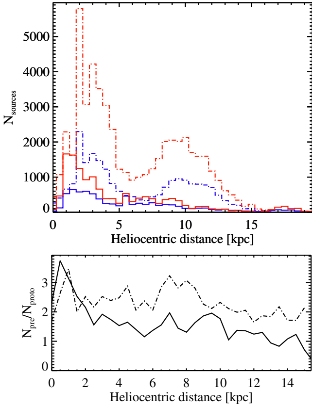
Figure 5. Top panel: number counts vs heliocentric distance for Hi-GAL pre-stellar (red) and protostellar (blue) clumps taken from both catalogues. Dot-dashed lines are used for distributions corresponding to the inner Galaxy, and solid lines for the outer one. Bottom panel: number ratio of pre-stellar to protostellar sources in the distance bins defined in the top panel, for the inner (dot-dashed) and the outer Galaxy (solid). To ensure statistical reliability, only bins in which both numerator and denominator are larger than 50 are reported, resulting in a foreshortened x -axis.
