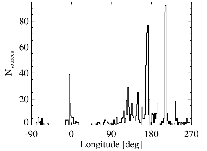
Figure 7. Number counts in 2^\circ -bins of Galactic longitude of Hi-GAL sources located in the FOG ( R_{\text{GC}} > 13.5 kpc). Both pre-stellar and protostellar sources are counted, from both catalogues. The x -axis range is set from -90^\circ to 270^\circ in order to place the local peaks around 0^\circ and 180^\circ well inside the plot area.
