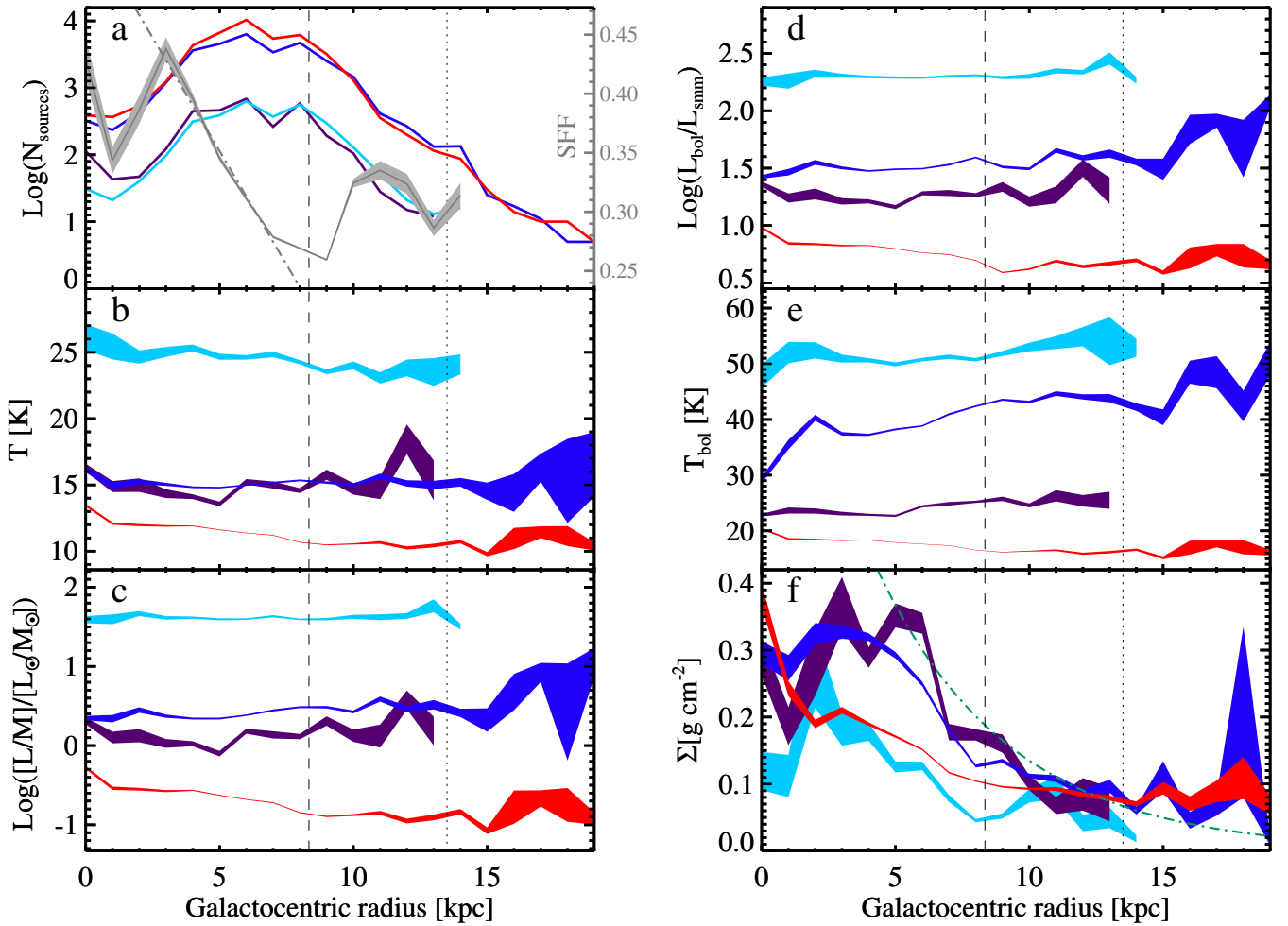
Figure 28. Characterization of sources vs Galactocentric radius in bins of 1 kpc for various populations: pre-stellar sources (red), all protostellar sources (blue), H II-region candidates (light blue), and MIR-dark protostellar clumps (dark purple). The vertical dashed and dotted lines mark the values adopted for the Solar circle and inner radius of the far outer Galaxy, respectively. Panel a : number of sources. The star-forming fraction (SFF, see the text) is also plotted in grey, referring to the grey y-axis on the right. The grey dot-dashed line represents a fit to the SFF data in the range 3 \text{ kpc} \leq R_{\text{GC}} \leq 7 \text{ kpc} . The remaining panels b through f are for T , L_{\text{bol}}/M , L_{\text{bol}}/L_{\text{smm}} , T_{\text{bol}} , and \Sigma , as labelled. In each bin the median and its uncertainty, calculated from interquartile ranges as explained in Table 4, are calculated and then the uncertainty intervals are displayed as shaded areas. Values are shown only for bins with at least 10 sources. In panel f , the green dot-dashed curve represents the radial dependence of the inverse of the gas-to-dust ratio predicted by Giannetti et al. (2017) ; the vertical scaling of the curve is arbitrary.
