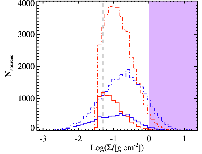
Figure 21. Distributions of surface density for pre-stellar (red histograms) and protostellar (blue histograms) in the inner Galaxy (dot-dashed histograms) and the outer (solid histograms). The zone surpassing the Krumholz & McKee (2008) threshold of 1 \text{ g cm}^{-2} is shaded purple, as in Fig. 10. The lowest surface density at which massive star formation is found by Urquhart et al. (2014), namely \Sigma = 0.05 \text{ g cm}^{-2} , is also reported as a dotted vertical line. Other thresholds for compatibility with massive star formation, discussed in Section 3.3, cannot be represented in this plot because they do not correspond to a constant value of \Sigma .
