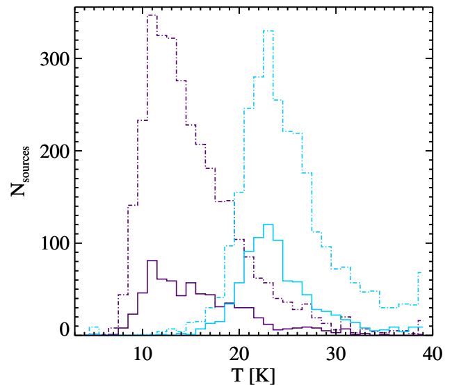
Figure 17. Same as Fig. 16 , but for two particular sub-classes of the protostellar sample: MIR-dark sources (dark purple histograms) and H II region candidates (light blue histograms).
