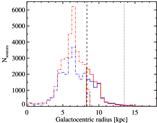
Figure 6. Same as Fig. 5, top panel, but for Galactocentric radius. The vertical dashed and dotted lines delimit the outer Galaxy and the so-called far outer Galaxy ( R_{\text{GC}} > 13.5 kpc), respectively.
