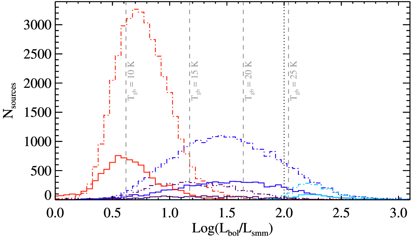
Figure 18. Distributions of the ratio of the bolometric luminosity to the portion in the sub-millimetre ( \lambda \geq 350 \mu\text{m} ) for the pre-stellar (red histograms), protostellar (blue histograms), MIR-dark protostellar (dark purple histograms, arbitrarily enhanced by a factor of 2 to improve the readability), and H II-region candidate (light blue histograms) Hi-GAL sources, respectively. Dot-dashed histograms are for the inner Galaxy and solid for the outer. For a MBB with \beta = 2 , the dashed grey vertical lines mark ratios corresponding to the different MBB temperatures indicated. The dotted black line at L_{\text{bol}}/L_{\text{smm}} = 100 marks the ratio separating Class 0 from Class I low-mass YSOs as proposed by Maury et al. (2011) .
