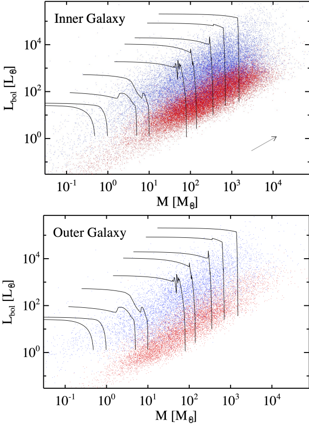
Figure 12. Top panel: bolometric luminosity vs envelope mass for pre-stellar (red) and protostellar (blue) sources in the inner Galaxy. The black lines represent evolution, upwards and then to the left, on tracks from Molinari et al. (2008) . As in Fig. 10, since the distance estimate is the main source of uncertainty for both M and L_{\text{bol}} , a hypothetical distance increase of a factor 2 is represented as an arrow at the bottom right corner. Bottom panel: same as top panel, but for the outer Galaxy.
