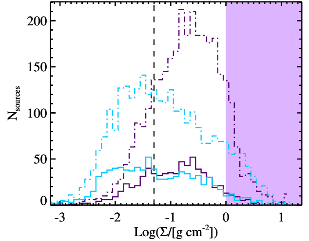
Figure 22. Same as Fig. 21, but for two sub-classes of the protostellar sample: MIR-dark sources (dark purple histograms) and H II region candidates (light blue histograms).
