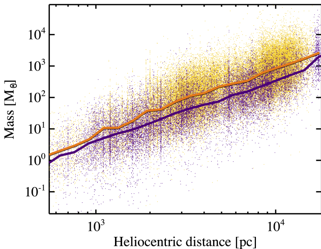
Figure 9. Clump mass vs heliocentric distance for sources in the inner (orange dots) and in the outer Galaxy (purple dots). Orange and purple thick lines represent the median mass in logarithmic bins of distance for these two populations, respectively.
