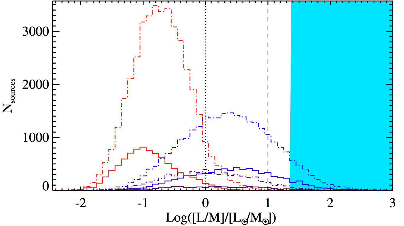
Figure 15. Distributions of the ratio of bolometric luminosity to envelope mass for pre-stellar (red histograms), protostellar (blue histograms) and MIR-dark protostellar (dark purple histograms, arbitrarily enhanced by a factor of 2 to improve the readability) Hi-GAL sources considered for science analysis in this paper. Dot-dashed histograms are for the inner Galaxy and solid for the outer. The dotted and the dashed vertical lines represent the thresholds identified by Molinari et al. (2016b) for expecting star formation to be traced by line emission of methyl-acetylene \text{CH}_3\text{C}_2\text{H}(12-11) or by the presence of a zero age main sequence (ZAMS) star inside the clump, respectively. The light blue-shaded area contains clumps that are candidates to host H II regions (see the text).
