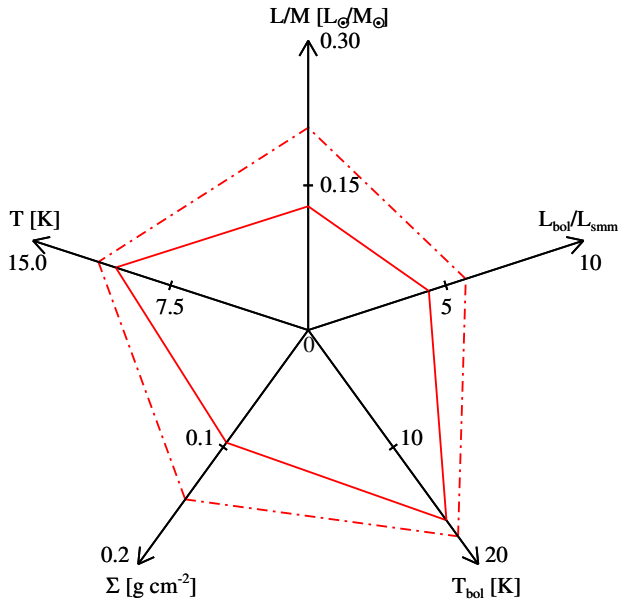
Figure 23. Radar plot for the median values of five distance-independent physical parameters (see text) for pre-stellar clumps, for the inner Galaxy (dot-dashed line) and the outer (solid line). Scales on each axis are linear, ranging from 0 to the value specified at the end.
