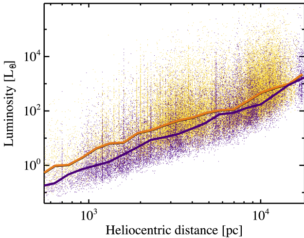
Figure 13. Same as Fig. 9, but for bolometric luminosity.
