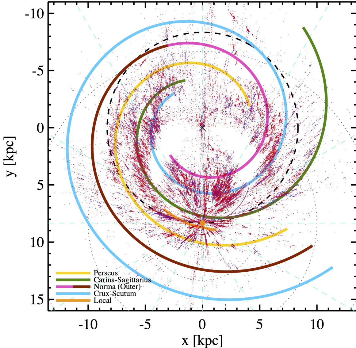
Figure 2. Positions projected in the Galactic plane for the pre-stellar (red dots) and protostellar (blue dots) Hi-GAL objects with a known distance (unbound objects not shown to reduce crowding). The Galactic centre at coordinates [x, y] = [0, 0] is indicated with a \times , and the Sun at [0.834] kpc with an orange dot. Some unnatural delineation of an imaginary circle passing through the Sun and Galactic centre arises from sources placed arbitrarily at the tangent point in the heliocentric distance estimates by Mège et al. (2021) , see the text. Cyan dashed lines indicate Galactic longitude in steps of 30^\circ . The Solar circle, separating the “inner” from “outer” Galaxy, is represented with a black dashed circle. Grey dotted circles represent heliocentric distances of 5, 10, and 15 kpc. Spiral arms from the four-arm Milky Way prescription of Hou et al. (2009) are plotted, except for the Local arm taken from Xu et al. (2016) , with the arm-colour correspondence at the bottom left. The Norma arm is represented using two colours: magenta for the inner part; and brown for the outer part, which is generally designated as the Outer arm, whose starting point is established in agreement with Momany et al. (2006) . The uniform line thickness is not representative of the actual arm widths.
