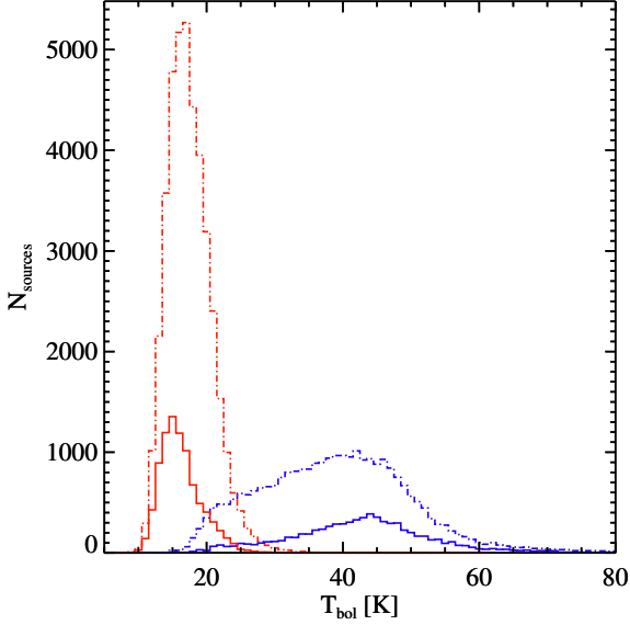
Figure 19. Distributions of bolometric temperature for pre-stellar (red) and protostellar (blue) sources. Dot-dashed histograms are for the inner Galaxy and solid for the outer.
