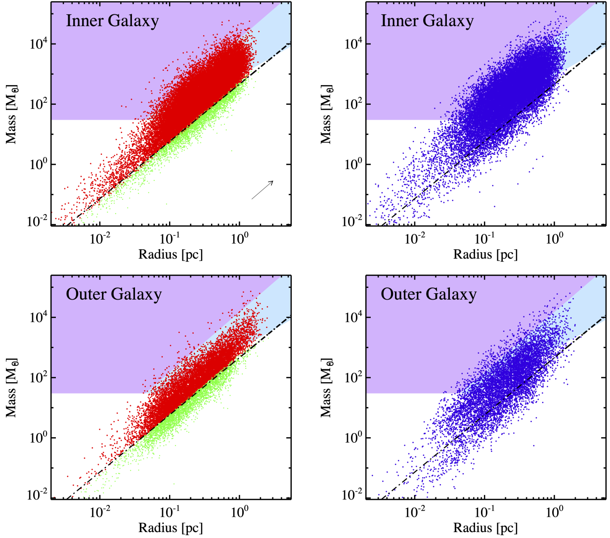
Figure 10. Mass vs radius plot for starless sources in the inner (top left-hand panel) and outer Galaxy (bottom left), and for protostellar sources in the inner (top right) and outer Galaxy (bottom right). Uncertainty in distance is the main source of error on both displayed quantities and the shift corresponding to a hypothetical distance increase of a factor 2 is shown as an arrow at the bottom right corner of the top left panel. In the left two panels containing starless sources, the dot-dashed black line M(r) = 460 M_{\odot} (r/\text{pc})^{1.9} (Larson 1981, see Section 2.1) separates pre-stellar (red) and unbound (green) sources. The area in each diagram fulfilling the Krumholz & McKee (2008) threshold for compatibility with high-mass star formation is shaded purple, and the less demanding Kauffmann & Pillai (2010) threshold contains this and extends it as indicated in light blue. Adopting 10 M_{\odot} as a lower limit for a massive star, and a star formation efficiency factor of 1/3 for the core-to-star mass transfer as in Elia et al. (2013), these shaded areas cannot extend below 30 M_{\odot} .
