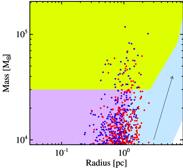
Figure 11. Mass vs radius for pre-stellar (red) and protostellar (blue) sources in the high-mass regime. As in Fig. 10, the shift corresponding to a hypothetical distance increase of a factor 2 is shown as an arrow. Purple and light blue areas are as introduced in Fig. 10. The overlying yellow sub-area towards high mass corresponds to the Bressert et al. (2012) threshold for identifying candidate massive proto-clusters.
