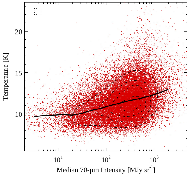
Figure 24. Temperature T of pre-stellar sources vs median intensity \bar{I}_{70} evaluated in 61 \times 61 pixel boxes centered on clump centroids in PACS 70 \mu\text{m} maps. For clarity, the density of points in the plot, evaluated on a grid whose element has the size of the dotted box placed at the top left corner of the plot, is represented with dashed contours starting from 200 and in steps of 200.
