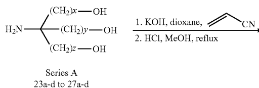
Scheme 25
