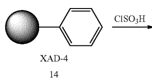
Scheme 12
