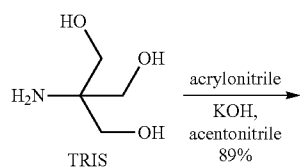
Scheme 45
