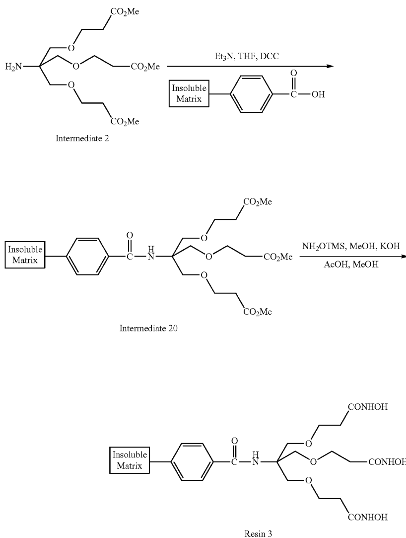
Scheme 14
