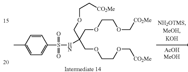
Intermediate 14
