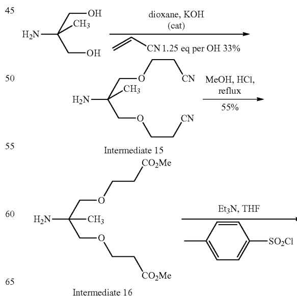
Intermediate 16
