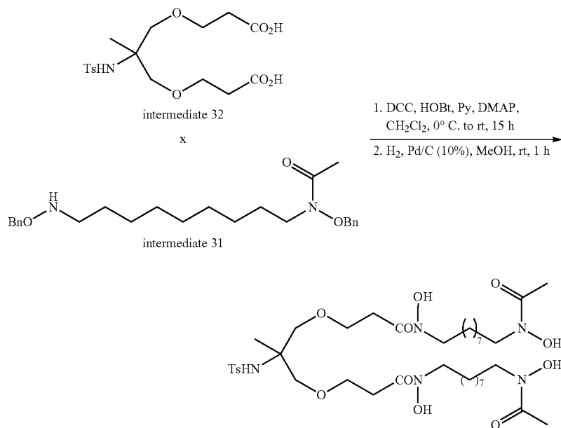
Scheme 36
