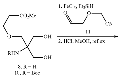
Scheme 10
