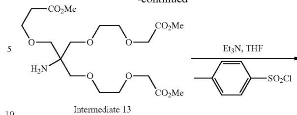
Intermediate 13
