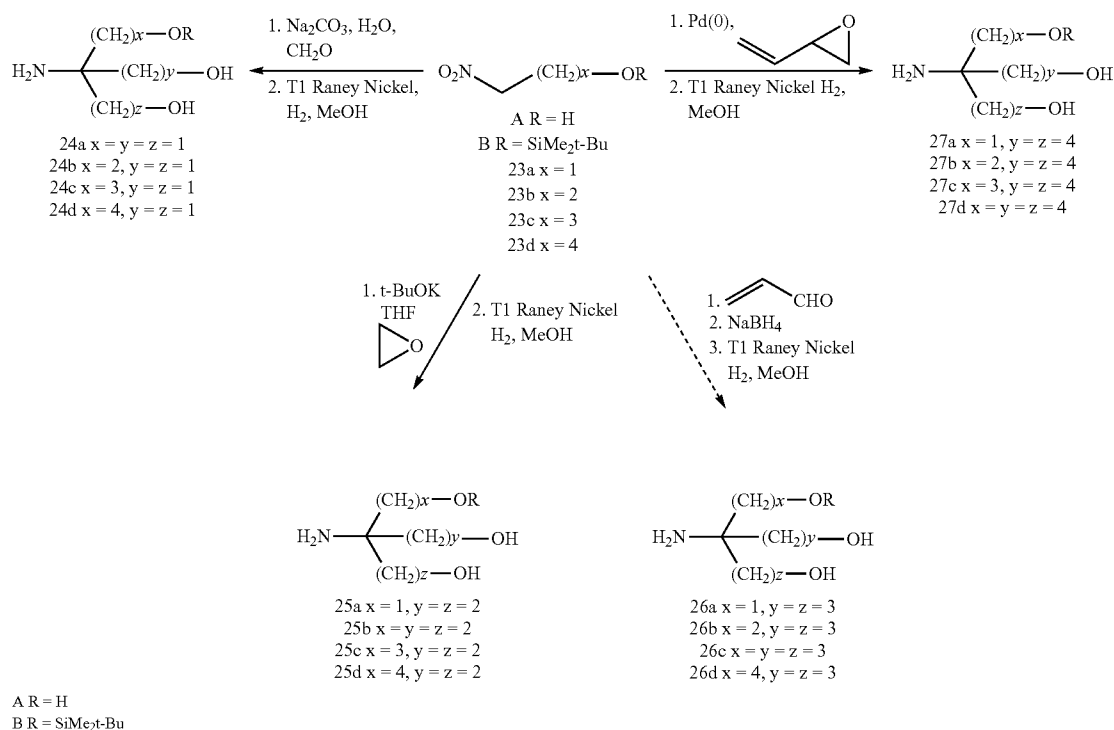
Scheme 24
