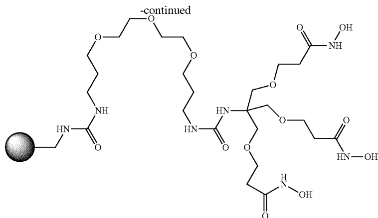
Resin 7 (0.70 meq/g)
