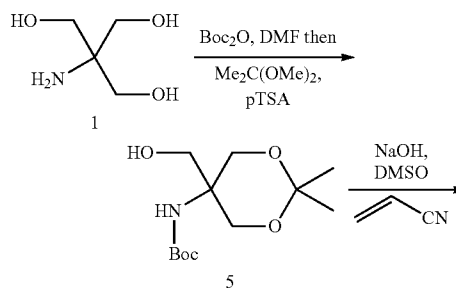
Scheme 8
