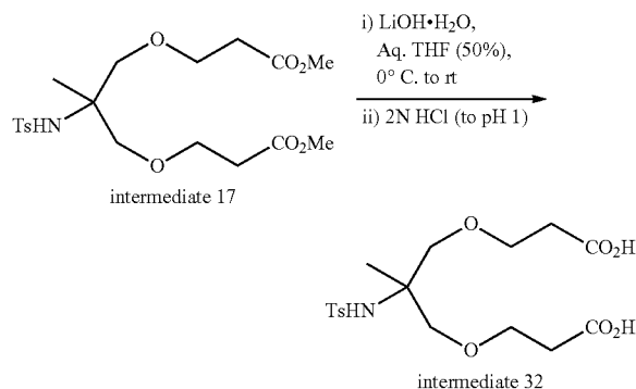
Scheme 35
