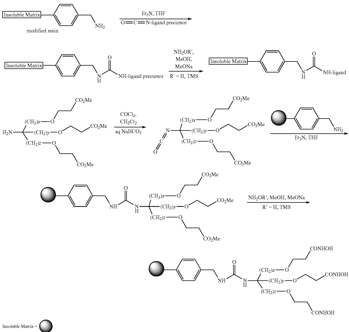
Scheme 19
