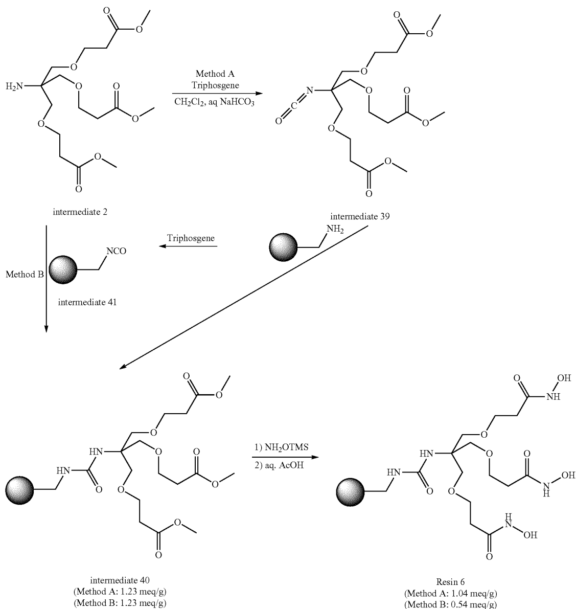
Scheme 42
