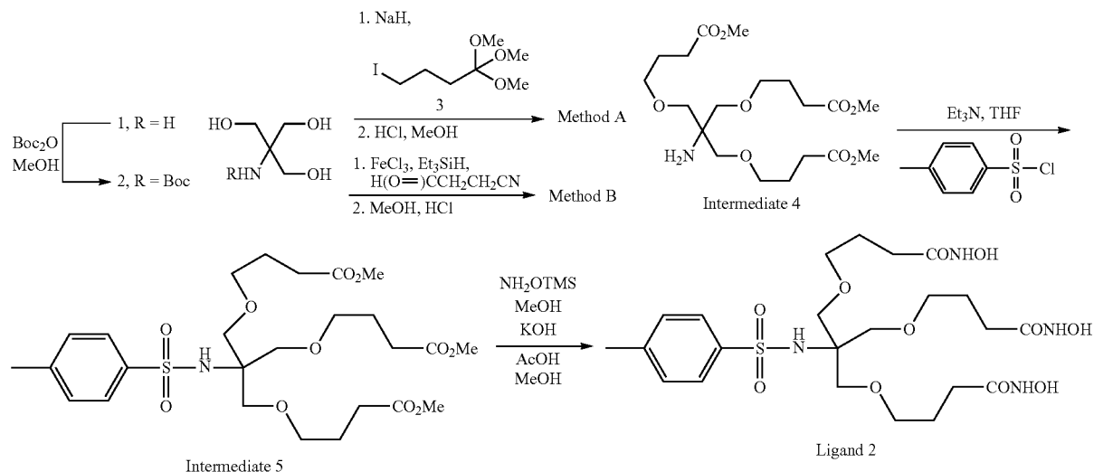
Scheme 6
