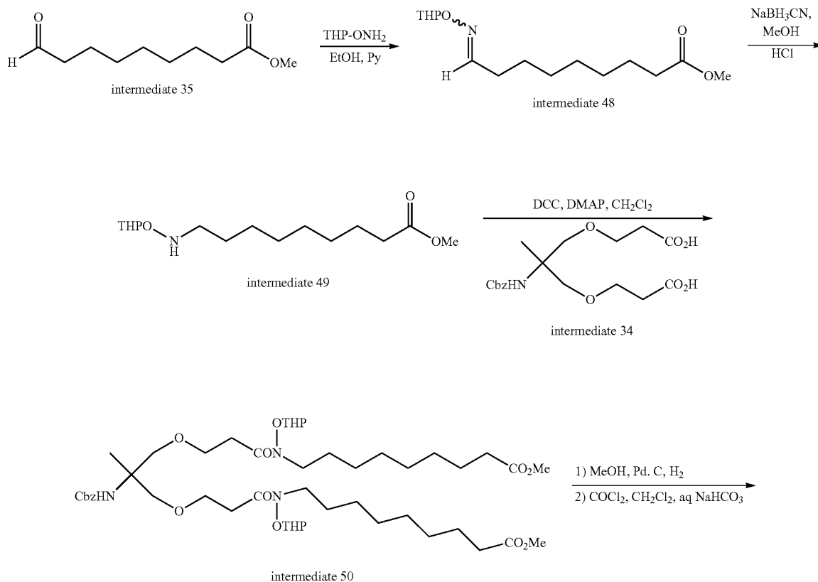
Scheme 46
