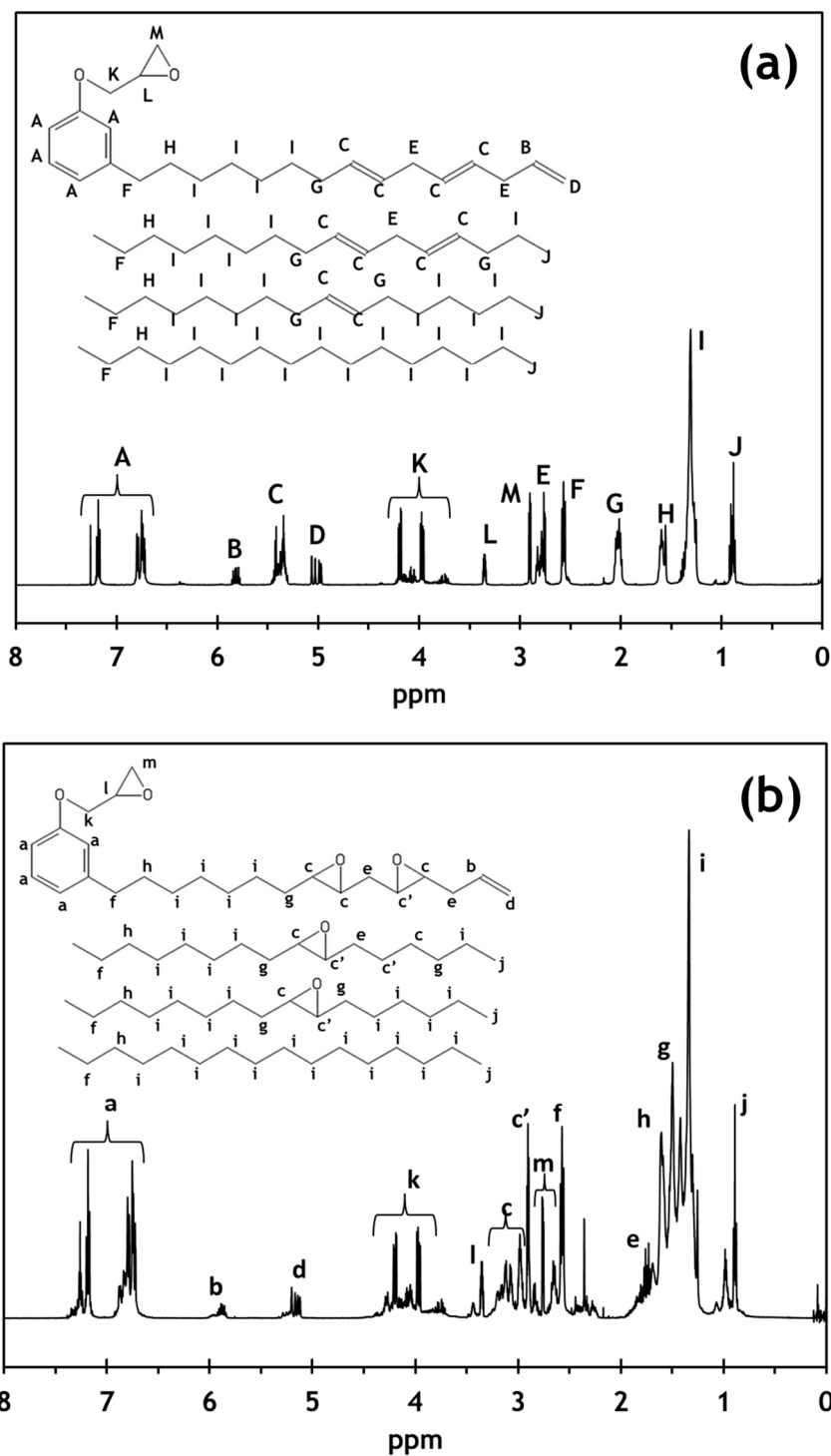
Figure 2. 1 H-NMR analysis of the reactant (a-top) and the epoxidized product (b-bottom). Chemical shift assignments are provided in Table S1 of the supplementary information.
