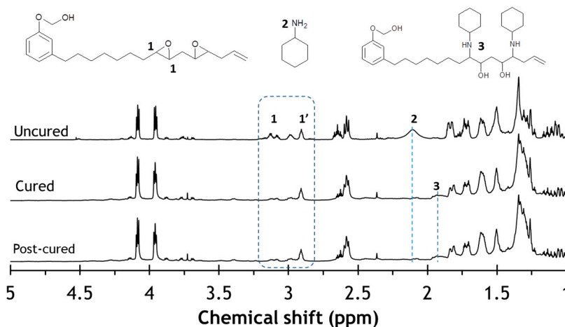
Figure 5. ^1\text{H} NMR spectra of the SCEC-MHA epoxy-amine mixture with 100% excess amine: initial uncured spectrum; spectrum of material cured at 90\text{ }^\circ\text{C} for 12 h; and spectrum of material postcured at 180\text{ }^\circ\text{C} for 24 h.
