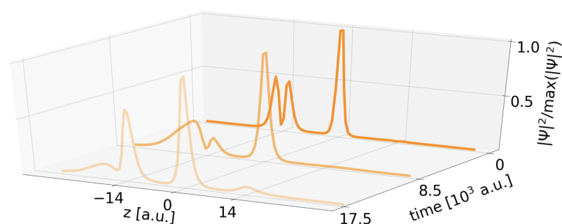
Figure 7. Illustration of the electron density distribution weighted to its maximal value for three propagation timesteps. The initial wavefunction has electron density corresponding to two electrons in one A^* state and in B separated by R_{AB} = 14 a.u., but no density in the other A site.
