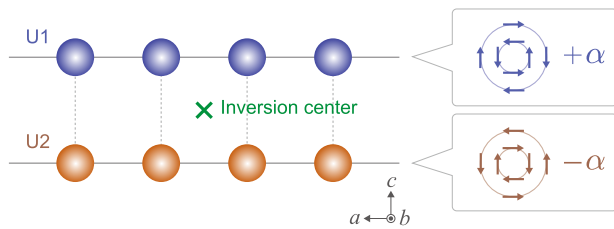
Fig. 2 Schematic of local \mathcal{P} -symmetry breaking in UTe 2 . U atoms form a ladder structure along the a axis. The ladder structure generates two non-equivalent sublattices U1 (blue circle) and U2 (orange circle). Since the \mathcal{P} -symmetry is locally broken in this crystal structure, a sublattice-dependent Rashba-type spin-orbit coupling (SOC) appears. To maintain the global \mathcal{P} -symmetry, the magnitude of Rashba SOC \alpha changes sign at each sublattice (i.e., +\alpha for U1 and -\alpha for U2).
