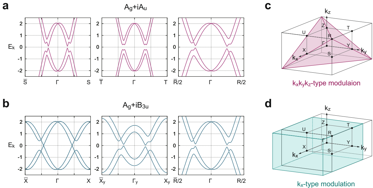
Fig. 3 Asymmetric Bogoliubov spectrum (BS) for the UTe_2 model. a, b Numerical results of BS in the UTe_2 model for the A_g + iA_u state and the A_g + iB_{3u} state. c Schematic of k_x k_y k_z -type asymmetric modulation in the Brillouin zone that is induced in the BS of A_g + iA_u state in a . d Schematic of k_x -type asymmetric modulation that is induced in the BS of A_g + iB_{3u} state in b . The symbols of the horizontal axis in a and b denote the \mathbf{k} -points in the Brillouin zone of a primitive orthorhombic lattice; \Gamma = (0, 0, 0) , X = -\bar{X} = (\pi, 0, 0) , S = -\bar{S} = (\pi, \pi, 0) , T = -\bar{T} = (0, \pi, \pi) , R = -\bar{R} = (\pi, \pi, \pi) , \Gamma_y = (0, \pi/4, 0) , and X_y = -\bar{X}_y = (\pi, \pi/4, 0) . In the numerical calculations, parameters are set to be t_i = 1.0 , \mu = -4.0 , \alpha = 0.4 , and (\Delta_1, \Delta_2) = (0.2, 0.2i) . The BS asymmetry appears in a and b consistent with the symmetry analysis of \text{Tr}[M^{(0)}(\mathbf{k})\hat{H}_0(\mathbf{k})] \propto \mathbf{g}_k \cdot (\mathbf{d}_k^g \times \mathbf{d}_k^u) .
