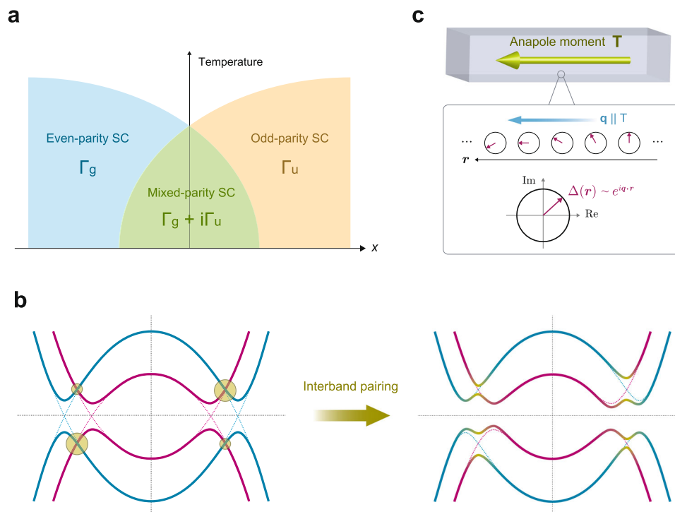
Fig. 1 Schematics of \mathcal{PT} -symmetric mixed-parity superconductivity (SC). a Schematic phase diagram in a superconductor with comparable strength of even- and odd-parity pairing interactions. The transition between the even-parity superconducting phase ( \Gamma_g ) and the odd-parity superconducting phase ( \Gamma_u ) is induced by tuning a control parameter x . For centrosymmetric systems with \mathcal{T} -symmetry, there is generally an intermediate mixed-parity superconducting phase ( \Gamma_g + i\Gamma_u ) where even- and odd-parity pairing components are coexistent with the relative phase difference \pm\pi/2 . b Illustration for a mechanism of the asymmetric Bogoliubov spectrum (BS) in \mathcal{PT} -symmetric mixed-parity multiband superconductors. \mathcal{P} - and \mathcal{T} -symmetry breaking interband pairing induces an asymmetric modulation of the BS. c Schematic figure of the anapole superconducting states. In real space, the phase of the superconducting order parameter \Delta(\mathbf{r}) becomes nonuniform along a direction parallel to the effective anapole moment \mathbf{T} as \Delta(\mathbf{r}) \propto e^{i\mathbf{q}\cdot\mathbf{r}} with \mathbf{q} \parallel \mathbf{T} , where \mathbf{q} is the center-of-mass momentum of Cooper pairs.
