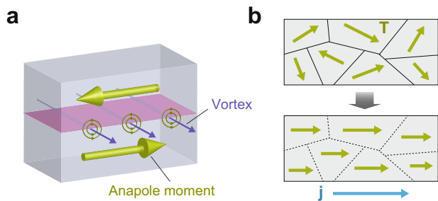
Fig. 4 Anapole domain and domain switching through supercurrent. a Vortices at the boundary of anapole superconducting domains. b The proposed domain switching in anapole superconductors. The effective anapole moment T is aligned along the injected supercurrent j .
