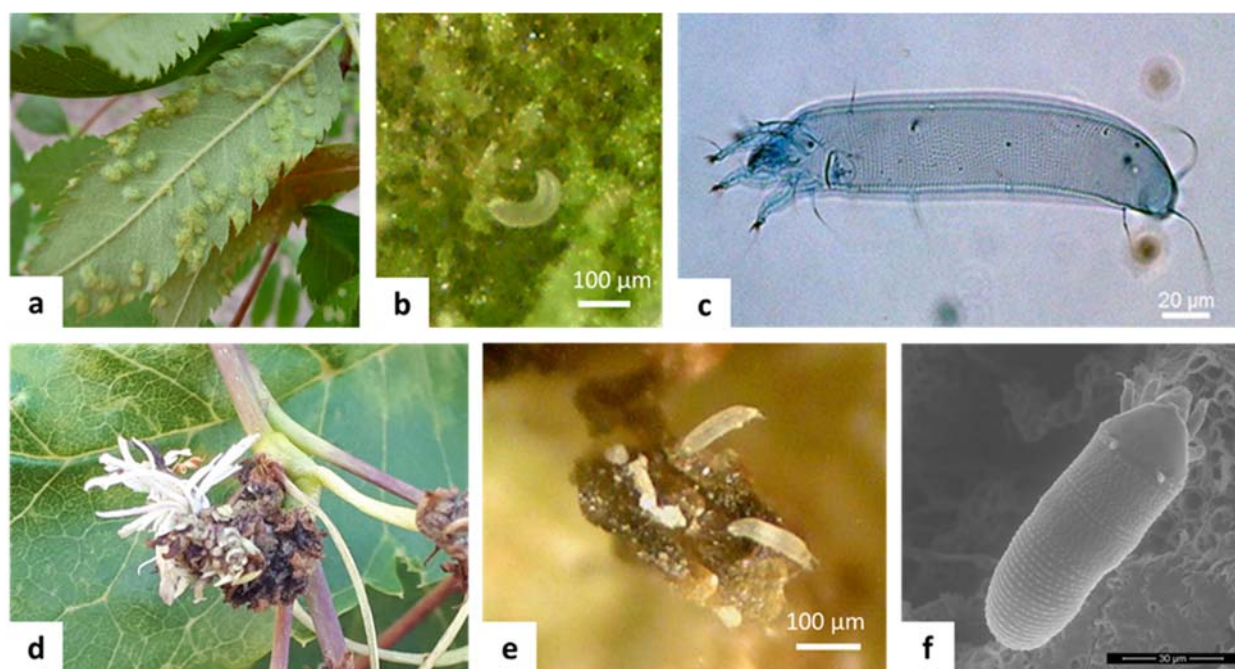
Figure 3. Gall mite symptoms and gall mite vectors associated with emaraviruses. (a) Galls induced by the pear leaf blister mite Phytoptus pyri (Pagenstecher) on the underside of an S. aucuparia leaf, (b) P. pyri in the erineum of the galls and (c) close up of the mite under a light microscope. (d) Cauliflower galls induced by the mite Aceria fraxinivora (Nalepa) in inflorescences of Fraxinus ornus and F. excelsior , (e) close up of A. fraxinivora mites inside the galls, and (f) detail of the mites as seen in electron microscopy, showing the characteristic prodorsal shield.
