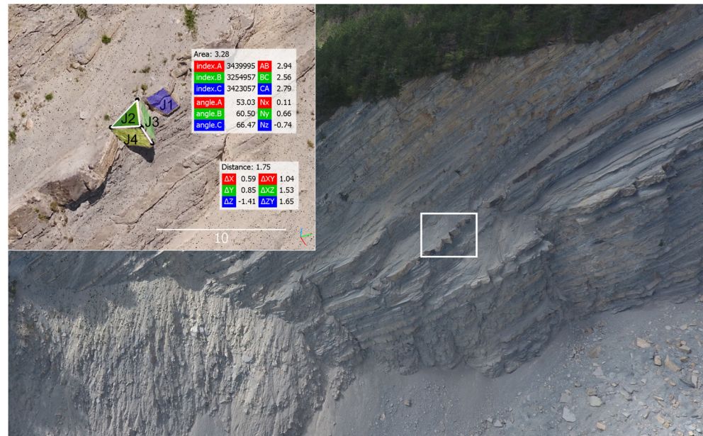
Figure 15. Overview of the left part of the Poggio Baldi landslide rock scarp and details of typical in situ rock block dimensions measured from the point cloud (white box).
