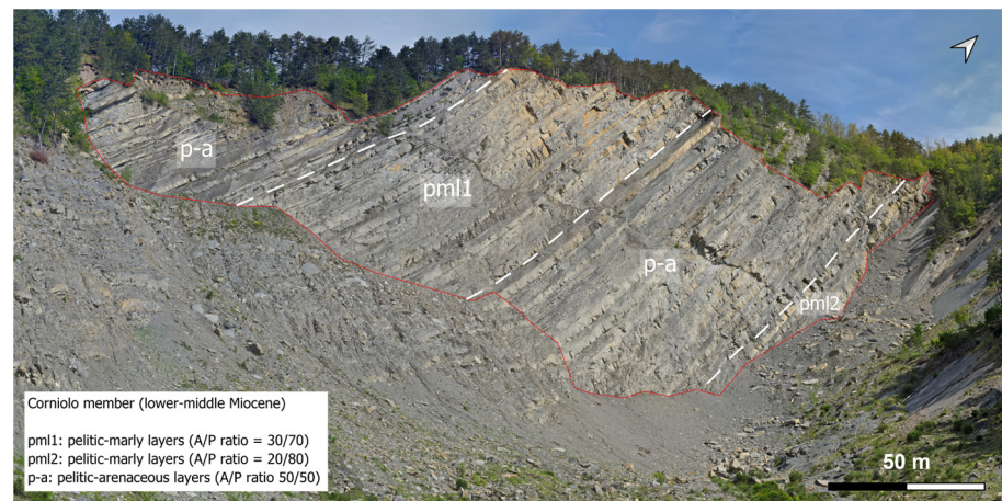
Figure 2. Front view of the main Poggio Baldi landslide scarp. The three different members of the Marnoso-Arenacea Formation are distinguished by the different content ratios of marly and arenaceous strata.
