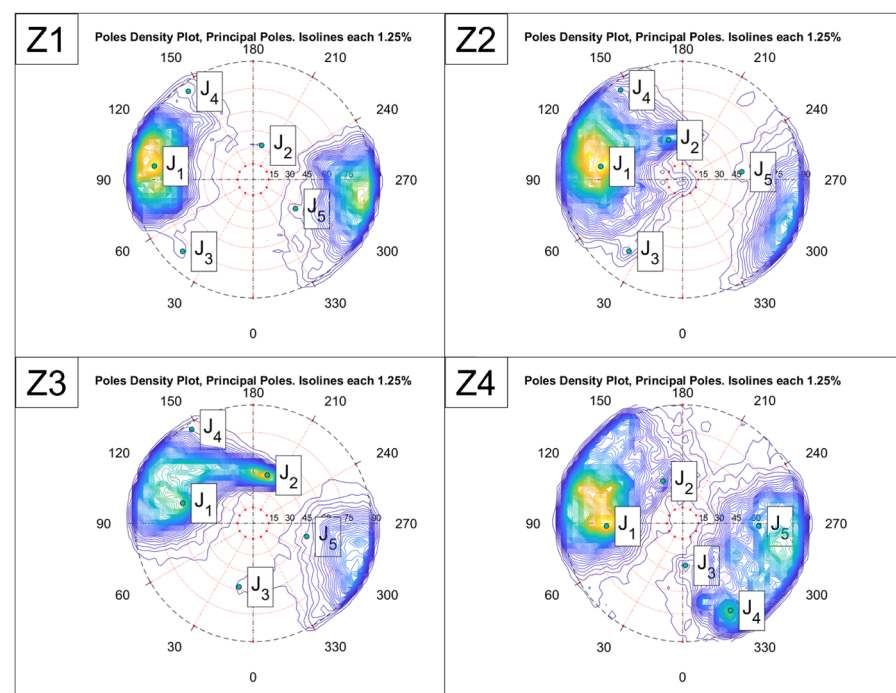
Figure 7. Stereoplots of discontinuity planes extracted utilizing DSE software at the selected source sectors.
