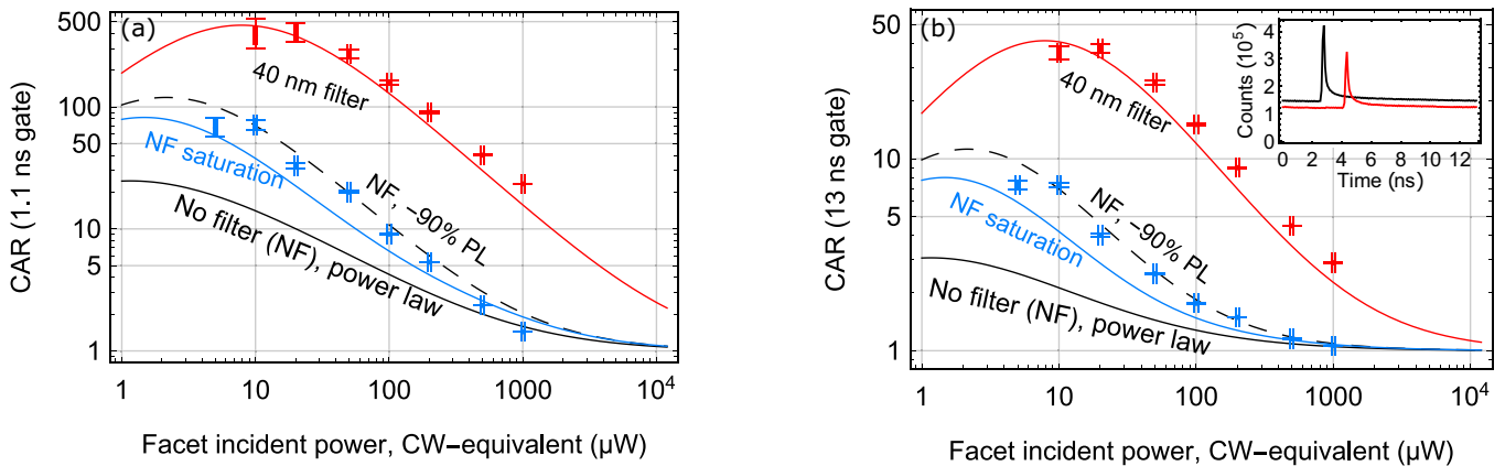
Figure 8. Predicted CAR values for different conditions with a pulsed pump at 76.2 MHz repetition rate. At low powers, the CAR is limited by the dark counts of the detectors ( 300 \text{ s}^{-1} ), at high powers by the accidental coincidences. Both the raw data (symbols) from figures 4 and 5 and curves derived from the different models (40 nm, red and No filter, black and blue) are shown. The black solid line depicts the no filter power law model, while the blue line is the corresponding saturation model, showing better agreement to the measurements, especially at low powers. The dashed line is a hypothetical sample, with the photoluminescence reduced by 90%. Here, choosing either the power law or saturation model made no significant difference. (a) shows the time filtered case with a 1.13 ns time gate, (b) the unfiltered with 13.1 ns. Note that the vertical scales are different by an order of magnitude. The inset in the upper right shows the time traces of the signal (red) and idler (black) emission when utilizing the pulsed laser at 1000 \mu\text{W} power with no filter. In comparison to the sharp peaks of the PDC signal, the photoluminescence appears as a very broad background—further emphasizing the benefit of short time gates.
