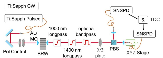
Figure 2. Sketch of the main setup for the pulsed excitation. The selected pump laser is coupled into the waveguide via an aspheric lens (AL) or a microscope objective (MO) on one side and the generated PDC is collected with another AL at the output facet. After collimation, the pump is suppressed by two longpass filters, followed by an optional bandpass. The photon pair is split deterministically at the polarizing beam splitter (PBS) and coupled to fibers via ALs on the XYZ translation stages and detected and correlated subsequently.
