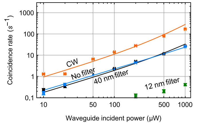
Figure 5. Recorded coincidences using a narrow 1.13 ns window. Here, photoluminescence models are not needed ( f(P) = 0 ) to explain the curves statistically well enough.
