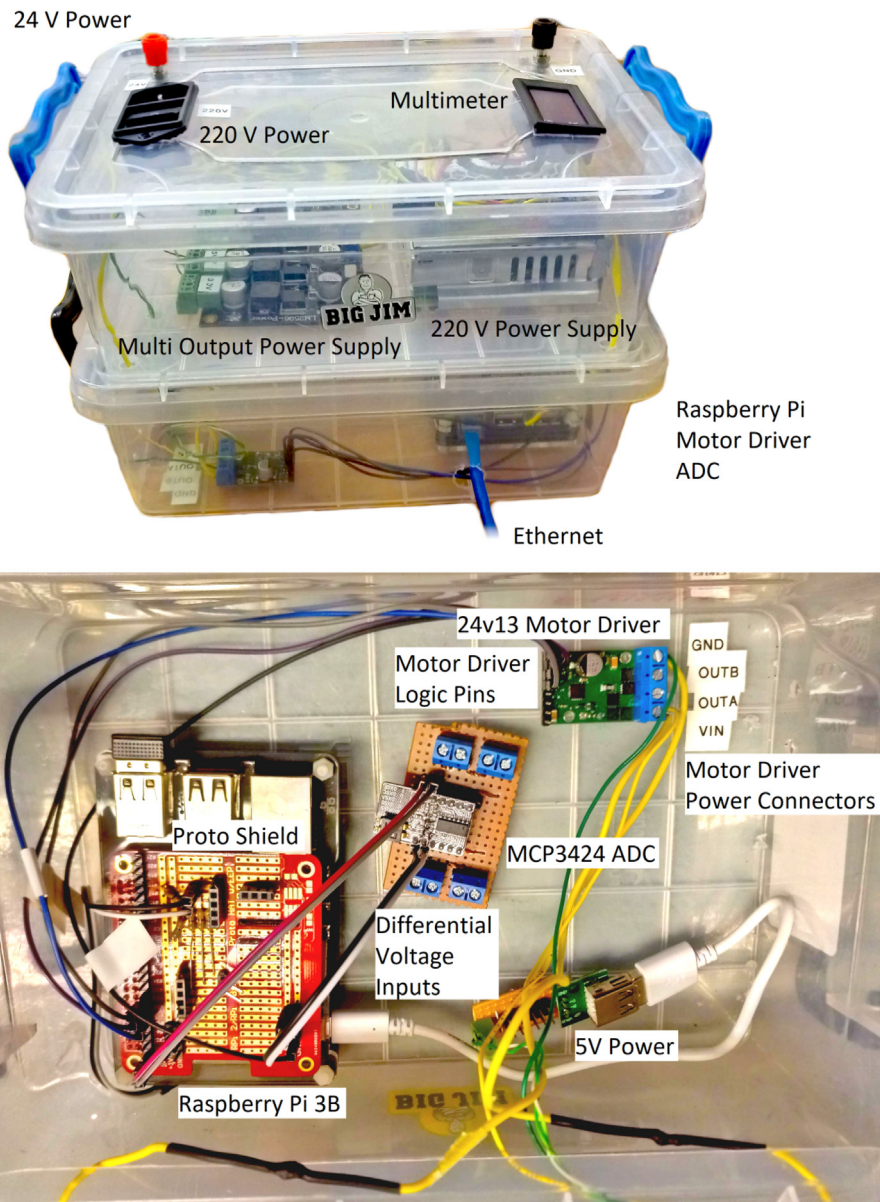
Fig. 5. Fly-by-Pi controller installed within a plastic container.
