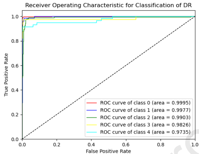
Figure 11. ROC matrix of ELM for APTOS 2019 dataset
