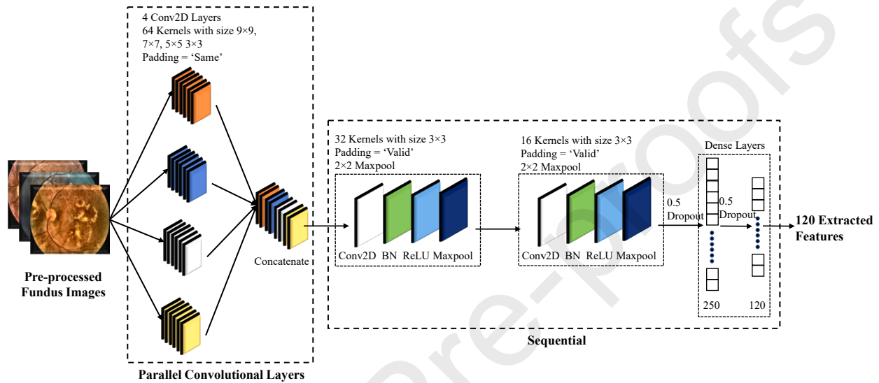
Figure 5. The lightweight parallel CNN to extract the features from FIs.
