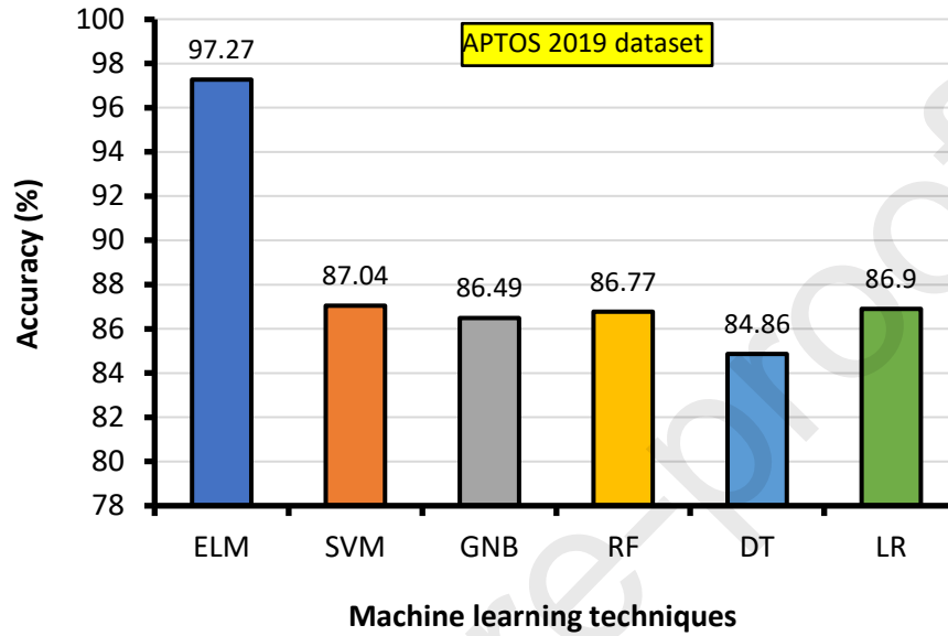
Figure 10. Accuracies of employed ML techniques for Dataset-1
