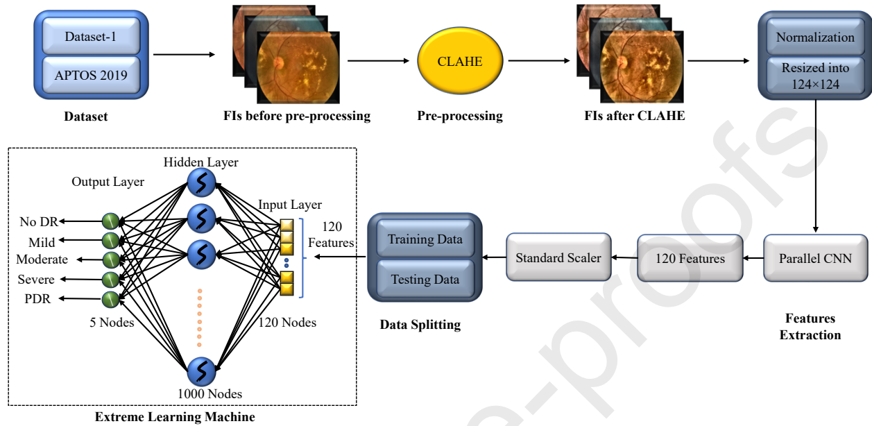
Figure 3. A proposed framework to detect the five levels of DR.
