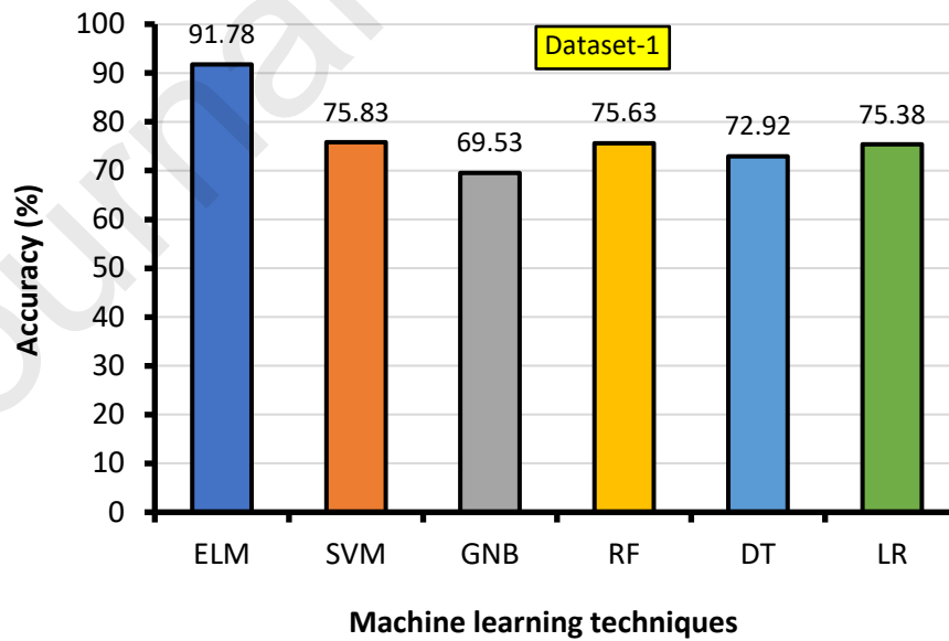
Figure 7. Accuracies of employed ML techniques for Dataset-1
