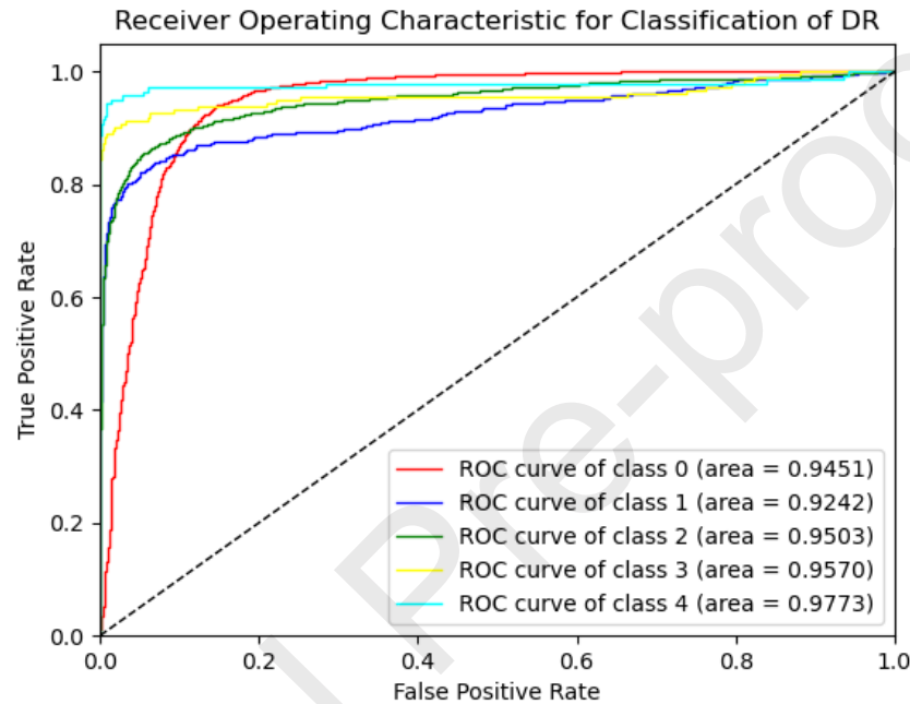
Figure 8. Receiver Operating Characteristic (ROC) curve of ELM for Dataset-1
