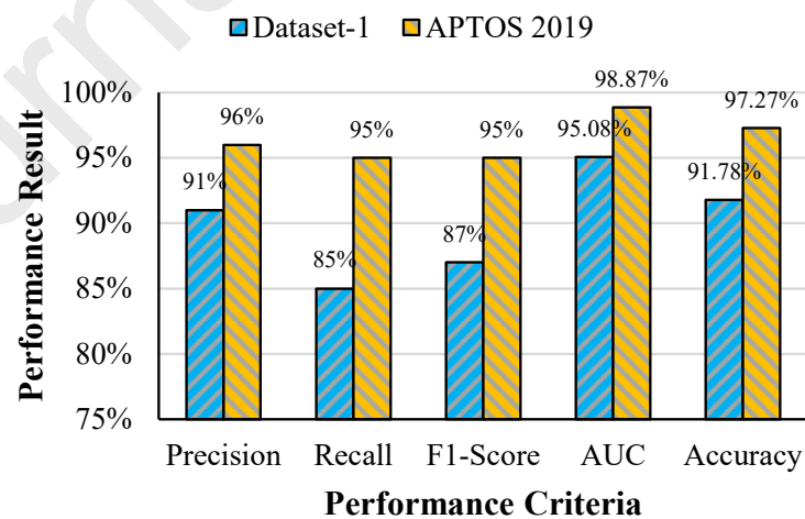
Figure 12. Graphical illustration of the classification performance of proposed framework
