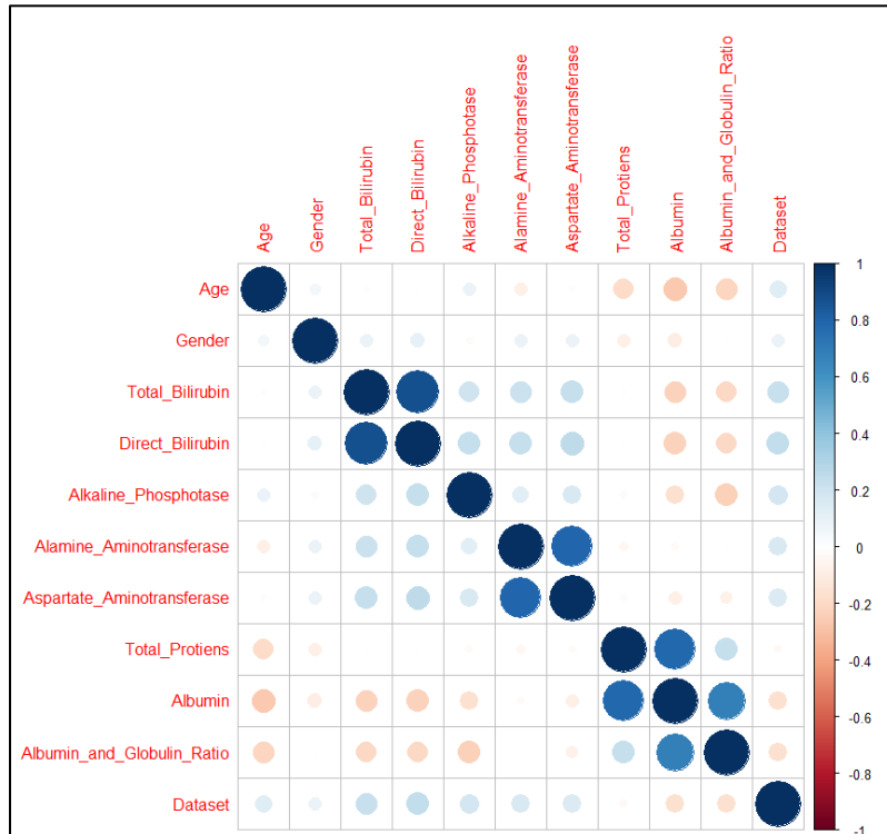
Figure 11: Correlation between the attributes
