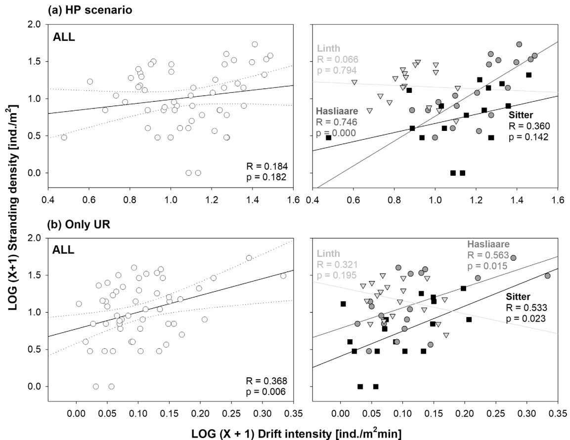
FIGURE 4 Relationship between drift intensity (ind./m 2 min) and stranding density (ind./m 2 ) based on linear regression models across all three HP reaches (“ALL”) and separated by reach (Sitter: black square; Hasliaare: dark grey circle; Linth: light grey triangle). (a) Drift data of an entire HP experiment: UR, P1, P2 and DR phase. (b) Only drift data of the UR phase. Solid lines: linear regressions; dashed black lines in the left plots: 95% confidence intervals. To better meet assumptions of normality and homogeneity of variances, all data were log transformed ( X + 1 ) prior to computing regressions. Although, in (b) the data for “ALL” and Hasliaare are not normally distributed. R: coefficient of multiple correlation. Please note different scales on x-axes of the upper (a) and lower (b) panels
