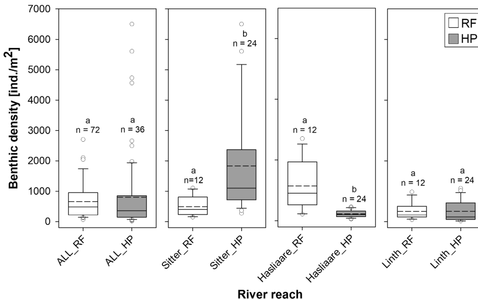
FIGURE 6 Benthic density (ind./m 2 ) across all three RF, respectively, all three HP reaches (“ALL_RF”, “ALL_HP”) and separated by reach. Numbers indicate the sample size, whereas letters show group affiliation according to Mann-Whitney tests
