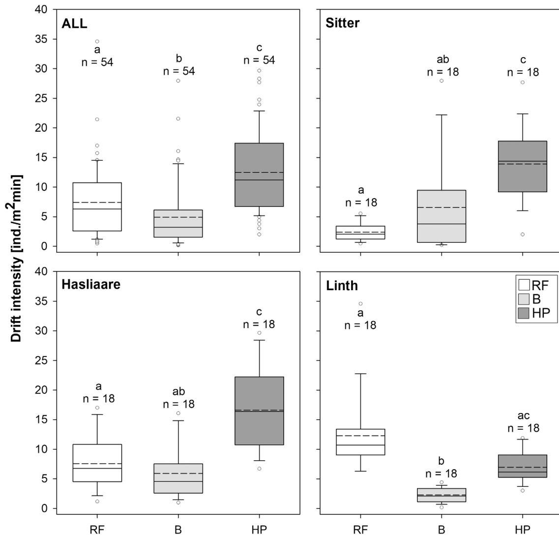
FIGURE 3 Drift intensity (ind./m 2 min) across all reaches (“ALL”) and separated by reach. RF: residual flow reach; B: base flow; HP: during hydropeaking (i.e. entire HP experiment: UR, P1, P2 and DR phase). Boxplots show the 25th and 75th percentiles, median (solid line in the box), mean (dashed line in the box), whiskers (10th and 90th percentiles) and outliers (white dots). Numbers indicate the sample size, whereas letters show group affiliation according to post hoc tests with Bonferroni correction
