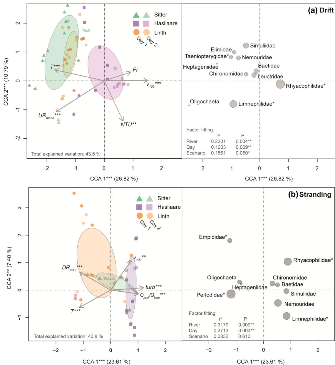
FIGURE 5 Biplot of Canonical Correspondence Analysis (CCA) based on (a) drift propensity and (b) stranding propensity of the most common taxa in the three HP reaches. Left panels: confidence ellipses (95% confidence limit, SD) are fitted on the CCA plots to depict differences between river reaches. Right panels: distribution of the species scores of the most common taxa (the larger the circle the higher the propensity). Asterisks indicate taxa with abundances >1% in the drift/stranding but not in the benthic samples (Appendix C in Data S1). Factor fitting shows the statistical differences in drift/stranding propensity between HP reaches (Sitter vs Hasliaare vs Linth), sampling day (day 1 vs day 2) and HP experiment (EXP1 vs EXP2 vs EXP3). Significant abiotic variables ( Q_{\text{peak}}/Q_{\text{base}} , flow ratio; UR_{\text{mean}} , mean up-ramping rate; DR_{\text{max}} , max. Down-ramping rate; v_{100} , flow velocity near the surface; Fr, Froude number; T, water temperature; NTU, turbidity) are depicted as grey arrows. Significance levels: *.05, **.01, ***.001 [Color figure can be viewed at wileyonlinelibrary.com ]
