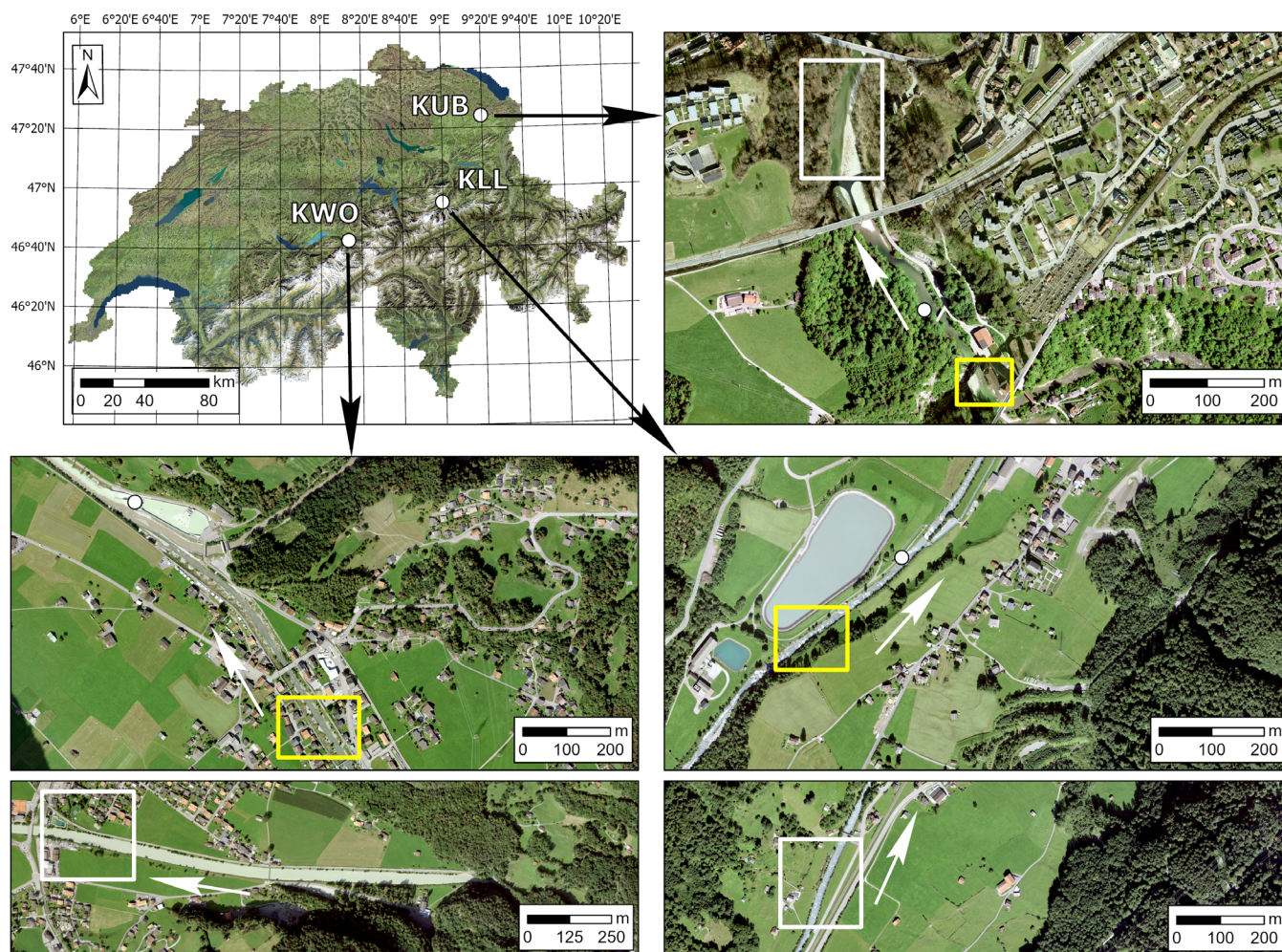
FIGURE 1 Overview map of the three study sites. White dots show the water releases of the hydropower plant KUB (river Sitter) and of the retention basins KWO (river Hasliaare) and KLL (river Linth). HP and RF reaches are identified with white and yellow rectangles, respectively. White arrows show the flow direction. Source background Orthophotos: Swisssimage © Swisstopo [Color figure can be viewed at wileyonlinelibrary.com ]
