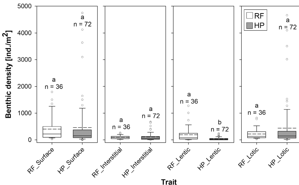
FIGURE 8 Benthic density (ind./m 2 ) across all three RF, respectively, all three HP reaches separated by the two traits “interstitial/surface” and “lentic/lotic”. Numbers indicate the sample size, whereas letters show group affiliation according to Mann–Whitney tests
