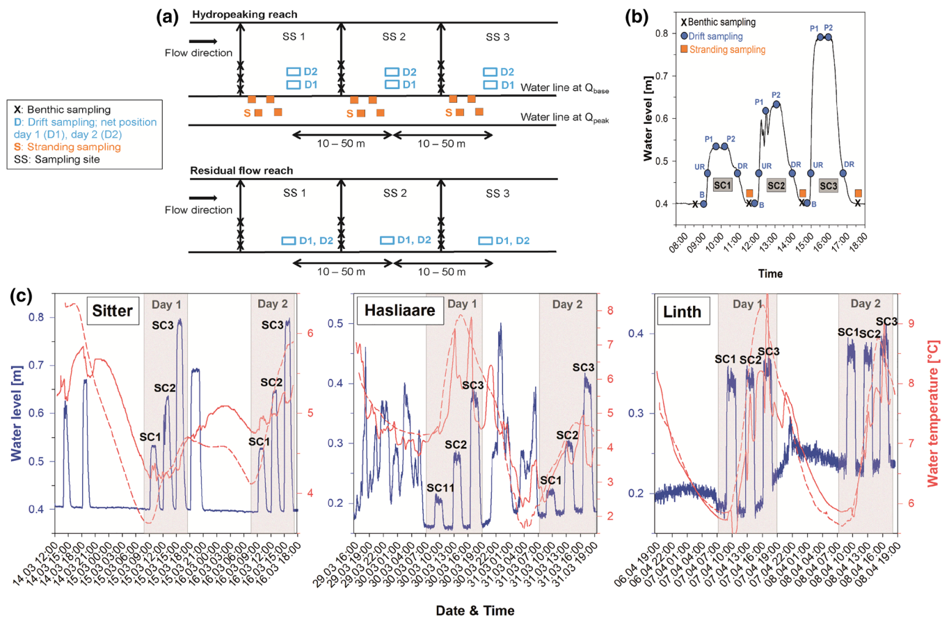
FIGURE 2 Experimental setup. (a) Schematic sampling design for HP (top panel) and RF reaches (bottom panel). (b) Chronological sampling illustrated as example of the three HP experiments (EXP1, EXP2, EXP3) at day one in the HP reach of the Sitter. Drift samples were collected separately at base flow (B) and during each HP phase: up-ramping (UR), first and second peak (P1, P2), down-ramping (DR). (c) HP experiments. Water level (blue solid line) and water temperature (red solid line) measured in the HP reaches as well as water temperature measured in the RF reaches (red dotted line). Grey squares indicate sampling period at day one and two. Please note different scales on y-axes [Color figure can be viewed at wileyonlinelibrary.com ]
