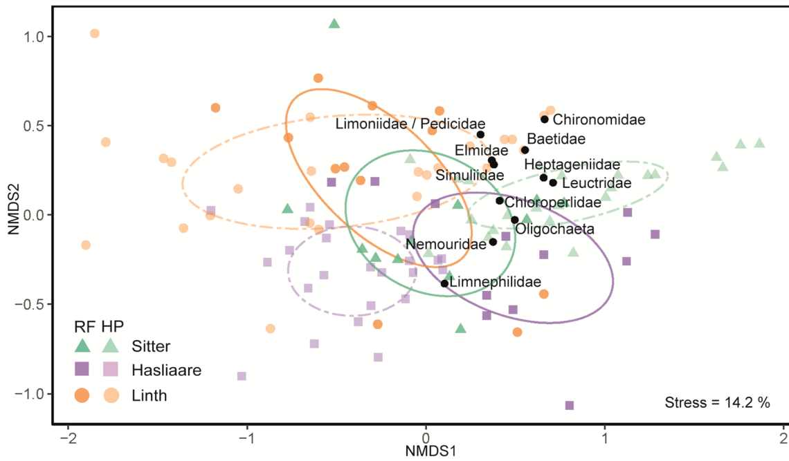
FIGURE 7 NMDS ordination of the three RF and three HP reaches based on benthic densities (ind./m 2 ) of the most common taxa (relative abundance >1%, Appendix C in Data S1). 95% confidence ellipses of the SDs of site scores of the three rivers (Sitter, Hasliaare, Linth) within the two respective reaches (RF, solid ellipses; HP, dashed ellipses) are depicted. Taxa that most contributed to dissimilarity ( p < .05 ) are fitted on the NMDS plot and indicated with black dots and taxon name [Color figure can be viewed at wileyonlinelibrary.com ]
