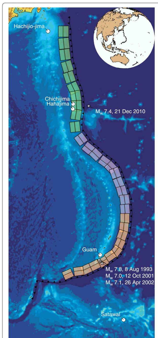
Fig. 1 Location of the Izu–Bonin–Mariana subduction system. Stars represent the four largest, shallow focus, instrumentally located earthquakes in the subduction system. Circles represent locations mentioned in this manuscript. Colored rectangles denote faults from the NOAA SIFT fault model database. The colors represent the fault segments used in this paper: the green segment is the Izu–Bonin segment, the purple segment is the north Mariana, and the orange is the south Mariana segment
