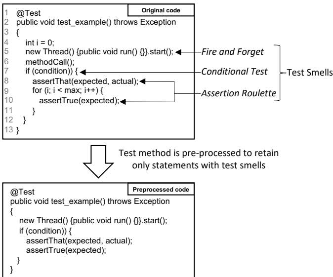
Figure 3: Example of pre-processing the source code of a test case, which leads to reducing the number of tokens from 62 down to 43
