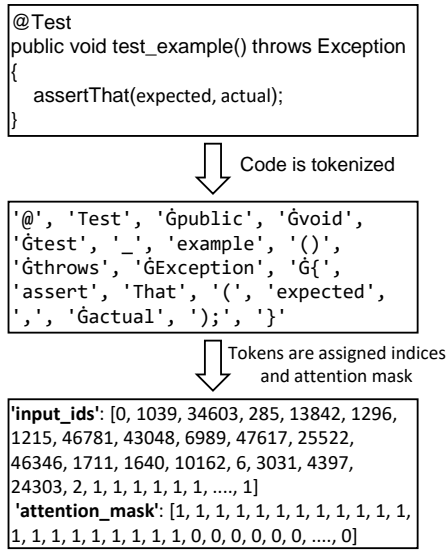
Figure 1: The process of converting the source code of a test case into a sequence of tokens, where each token is assigned an input index (id) and attention mask. Dots ‘...’ are used to save space, since the actual length is 512. The input id of each token refers to a 768-dimensional vector representation.
