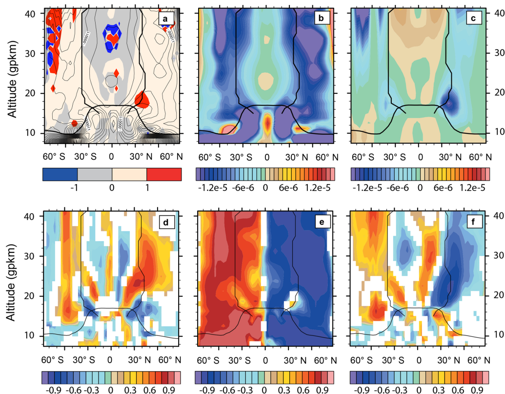
Figure A1. (a) GWD / EPFD ratio of the Ref period. The color scale is chosen so that the regions with the absolute value of zonal mean zonal GWD stronger than EPFD are highlighted. The contours show the total drag Ref climatology. (b) EPFD and (c) GWD climatology of the Ref period (units \text{kg m s}^{-2} ). Correlations between (d) GWD and EPFD, (e) EPFD and \bar{v}^* , and (f) GWD and \bar{v}^* in the Ref period. The vertical axis is in geopotential kilometers (gpkm). The plots are overlaid by the mean tropopause and turnaround latitude positions in the Ref period. Only regions with a statistical significance of correlations exceeding the 95 % confidence level are plotted.
