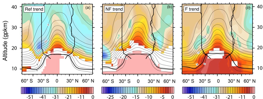
Figure 6. CMAM zonal mean AoA annual trend (days per decade) after the correction of the pressure levels trend for the Ref (a), NF (b) and F (c) period, in colors. Only trends that exceed the 95 % significance level are plotted. The mean AoA climatology of the respective period is contoured, and the tropopause and the turnaround latitudes (computed from the residual circulation field interpolated to the geopotential height corrected to the upward shift of the pressure levels) are shown by bold black lines. The turnaround latitude of the preceding period is illustrated by a dashed line.
