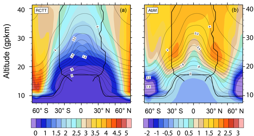
Figure 8. (a) CMAM zonal mean RCTTs (year) and (b) AbM averaged over the 1970–2000 period. The thick black lines show the mean tropopause and the turnaround latitude positions in the Ref period.
