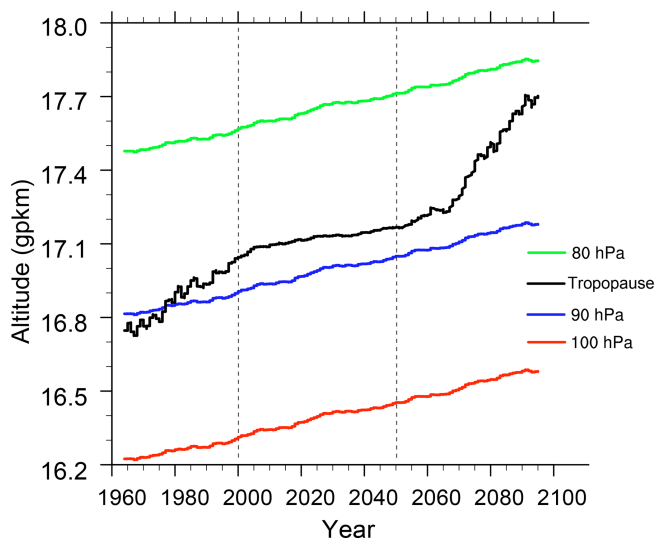
Figure 4. Time evolution of CMAM zonal mean geopotential height (gpkm) of selected pressure levels and of a first lapse rate tropopause averaged between 30° S and 30° N smoothed by a decadal running average.
