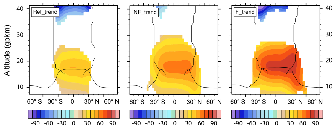
Figure 3. CMAM trend of geopotential height of pressure levels (gpm per decade) interpolated to the climatological geopotential height of the selected pressure levels in each period. The mean tropopause and turnaround latitude positions are marked with black lines. Only the trends in the regions where they exceed the statistical significance of 95 % confidence level are plotted.
