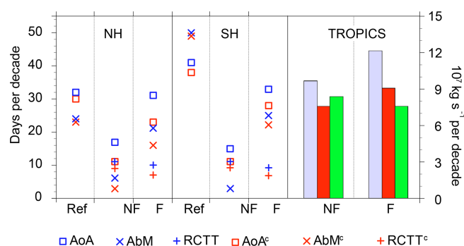
Figure 5. Trends of AoA (squares), AbM (crosses) and RCTT's (pluses) averaged over the Ex regions (ExNH on the left, ExSH in the middle) in the Ref, NF and F period in days per decade. Blue markers denote the trends in the geopotential height vertical coordinates and red markers the trends computed after the correction for the vertical shift of pressure levels. On the right (tropics), bars represent UP_{wstar} trends at 20 gpkm before (blue) and after the correction (red) for the vertical shift of pressure levels and also after the correction for the tropopause shift (green) given in 10^7 \text{ kg s}^{-1} per decade. The Ref period is not included as there are no significant UP_{wstar} trends. Presented are only trend values significant at least at the 90 % confidence level. AbM and RCTT trends are computed in a reduced Ref period (1970–2000).
