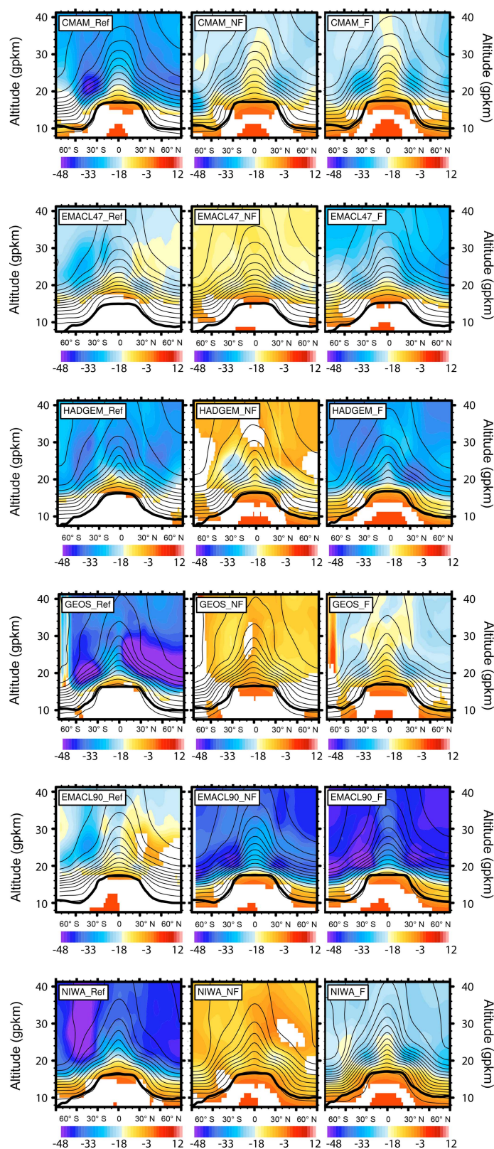
Figure 2. Zonal mean AoA trends (days per decade) (colors) and AoA climatology (contours) of the analyzed CCMI-1 REF-C2 simulations. The left column shows the Ref period, the middle column the NF period and the right column the F period. The vertical axis is in geopotential kilometers (gpkm). The mean tropopause position is indicated by the bold black line. White regions mark where the significance level of the trends does not exceed 95 %.
