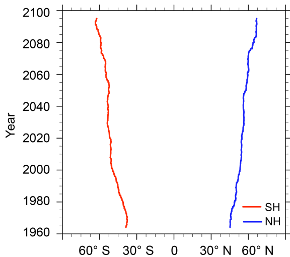
Figure 7. Time evolution of the meridional position of the zonal mean AoA = 2 years isoline at 20 gpkm after the correction to the upward shift of pressure levels for CMAM. The evolution is smoothed by a decadal running mean.
