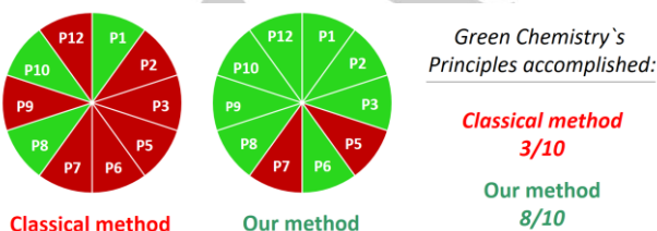
Scheme 2. (a) Gram-scale reaction with sunlight irradiation and with TBHP at 70 °C and semi-quantitative evaluation using the Ecoscale. (b) Qualitative evaluation of the accomplishment of Green Chemistry's principles (P1-P12).
