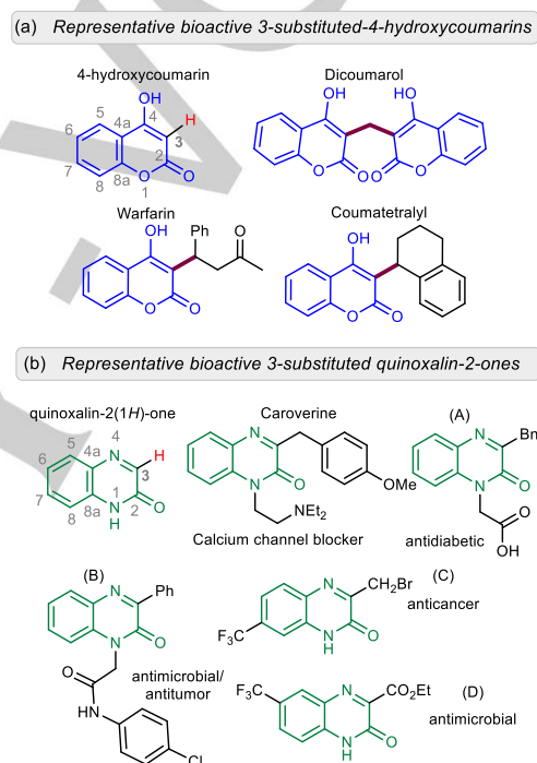
Figure 1. Representative bioactive 4-hydroxycoumarins and quinoxalin-2(1 H )-ones.
