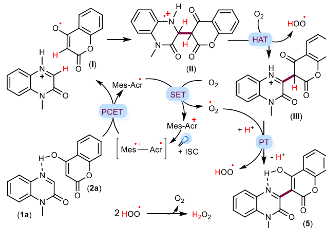
Scheme 5 Plausible mechanism.
