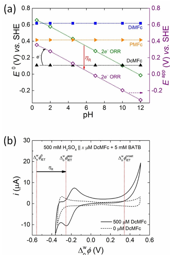
Figure 3. (a) Taking the intrinsic overpotential (η R ) of the biphasic 2e - ORR at a polarised L|L interface into account, the apparent redox potential (E app , purple diamonds) required for O 2 to undergo a biphasic 2e - ORR shifts negatively compared with E 0 (green diamonds). (b) In turn, as overlaid on the CV obtained at pH 0.55 in the presence of 500 μM DcMFC at a scan rate of 20 mVs -1 (shown previously in Figure 2b), the apparent Galvani IET potential (Δ o w φ IET app ) shifts positively by η R on the Galvani scale compared with Δ o w φ IET o . The positive shift of Δ o w φ IET app is also shown in a plot of Δ o w φ versus pH for the biphasic 2e - ORR with DcMFC in Figure S5. A further reason for the positive shift of Δ o w φ IET app compared to Δ o w φ IET o is that the Δ o w φ IET o values were calculated using the E 0 values for ORRs with aqueous H 3 O + as the proton source, whereas more negative E app values for ORRs involving interfacial [H + ...TB - ] as the proton source may be more appropriate. Clearly, a major mismatch exists between the predicted value of Δ o w φ IET app and the experimentally observed onset interfacial Galvani potential difference (Δ o w φ IET onset ) for the biphasic 2e - ORR with DcMFC, which appears at a much more positive applied Δ o w φ.
