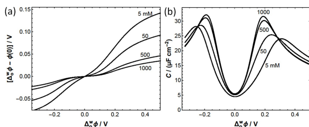
Figure 8. (a) The Galvani potential drop \Delta_0^w \phi - \phi(0) in the aqueous phase, where \phi(0) is the potential at the L|L interface, is significantly smaller than \Delta_0^w \phi because most of the applied interfacial Galvani potential difference drops in the organic phase. These calculations correspond to Electrochemical Cell 1 (see Scheme 2a), 5 mM BATB (TFT) || y mM \text{H}_2\text{SO}_4 (aq), for y = 5, 50, 500 , and 1000, using a modified Verwey-Niessen model that accounts for the finite size of the organic phase ions. Their maximum concentration has been given the roughly estimated value of 2 M. (b) The differential capacitance curves show local maxima due to finite ion size effects. The local maxima of the capacitance curves roughly correspond to the applied \Delta_0^w \phi where the organic ions reach their maximum concentration (see concentration profiles in Figure S10). The curvature of the capacitance curve at its minimum decreases with decreasing sulfuric acid concentration, in agreement with observations in Figure 5a.
