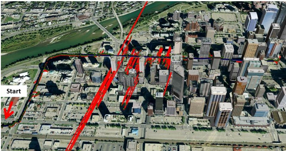
Fig. 7.8. Position solution using GPS measurements only (position green dot, path red line) and compared to ground truth (blue) in an urban canyon in downtown of Calgary, shown in Google Earth.
