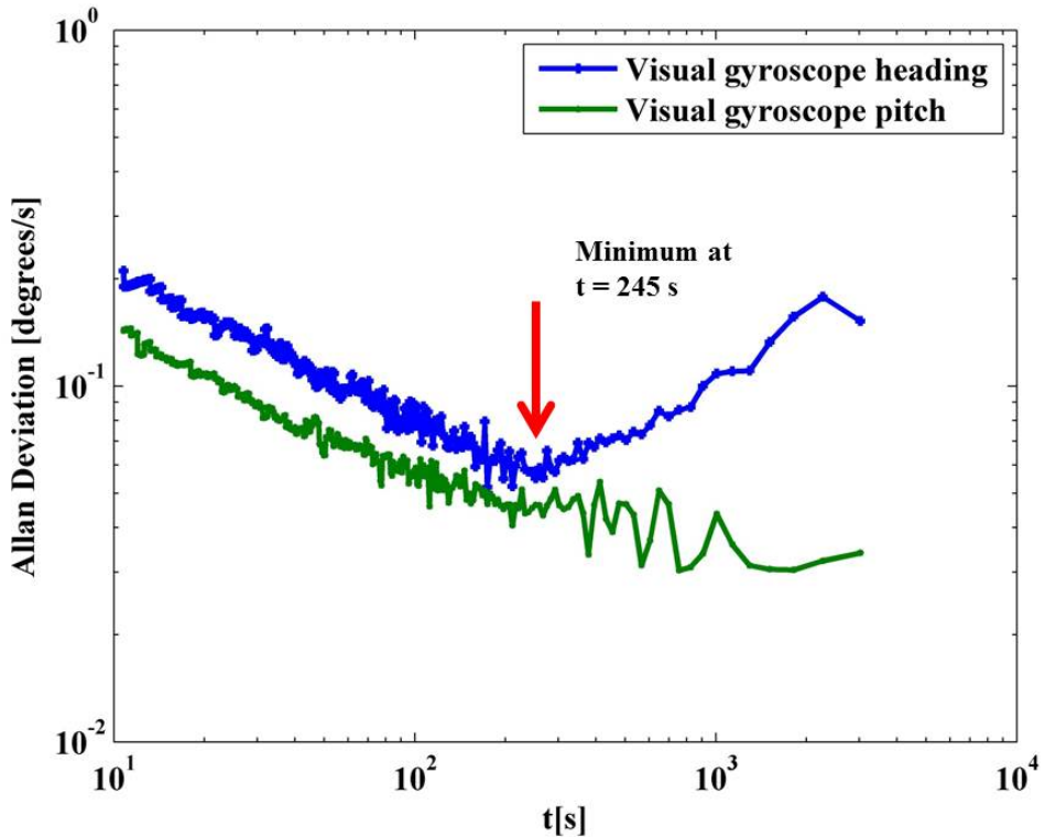
Fig. 4.4. Allan deviation plot showing the noise in the visual gyroscope.
