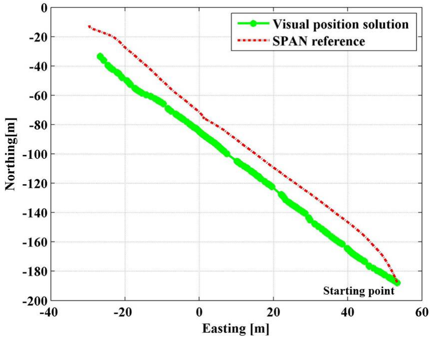
Fig. 6.7. The two-dimensional position solution in the Iso Omena shopping centre with visual stand-alone solution (green) and SPAN reference (red).
