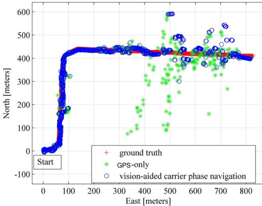
Fig. 7.5. Position solution in an urban canyon using the ground truth (red), GPS-only (green) and vision-aided carrier phase navigation (blue).
