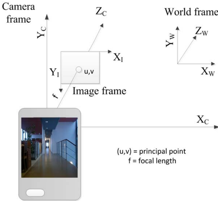
Fig. 3.1. Camera, image and world coordinate frames.
