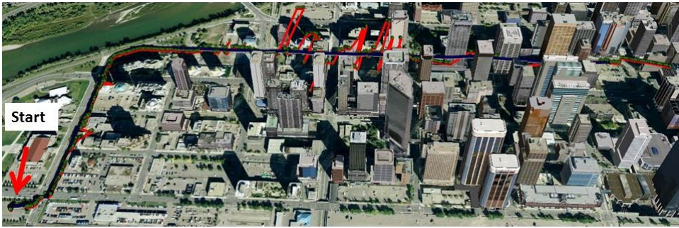
Fig. 7.7. Position solution using vision-aided carrier phase navigation (position green dot, path red line) and compared to ground truth (blue) in an urban canyon in downtown of Calgary, shown in Google Earth.
