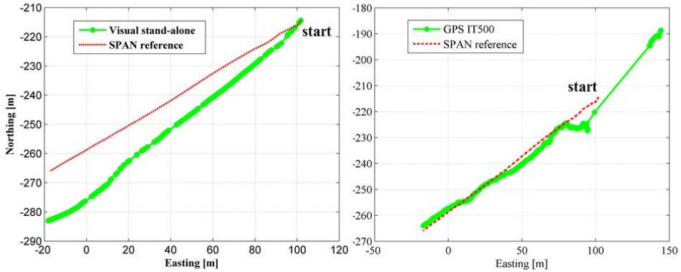
Fig. 6.9. Position solutions obtained in an urban canyon using a visual stand-alone system (green, on left) and an IT500 GPS receiver (green, on right). The ground reference is shown in red.
