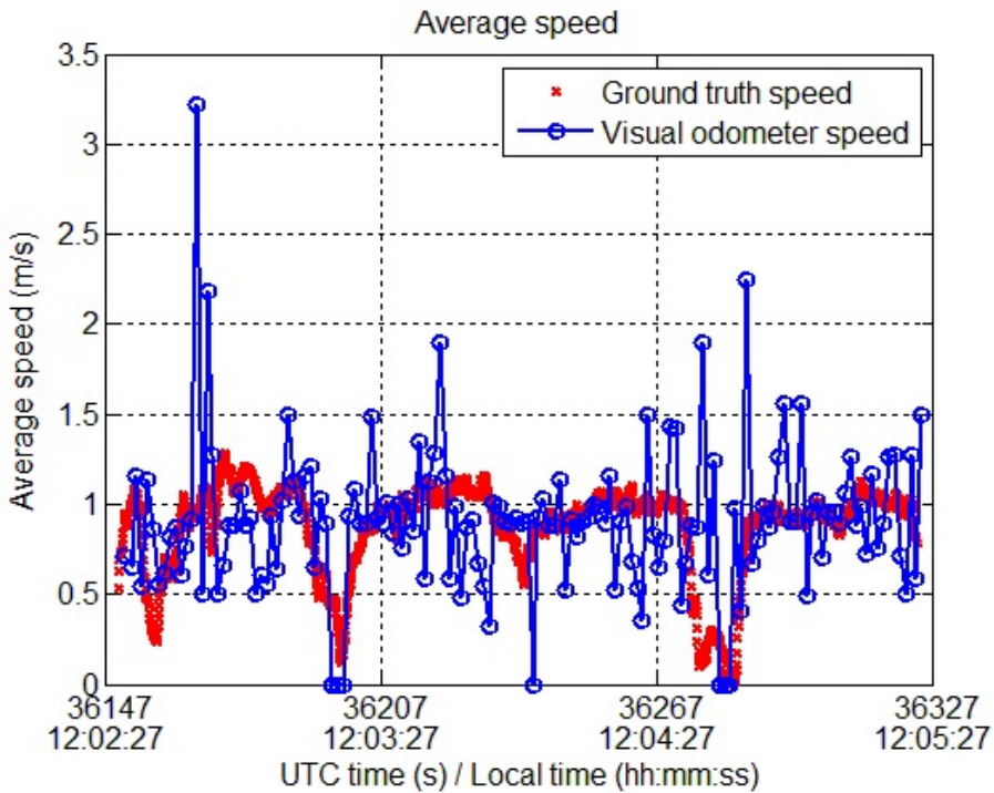
Fig. 6.3. Average speed from ground truth (red) and visual odometer (blue).
