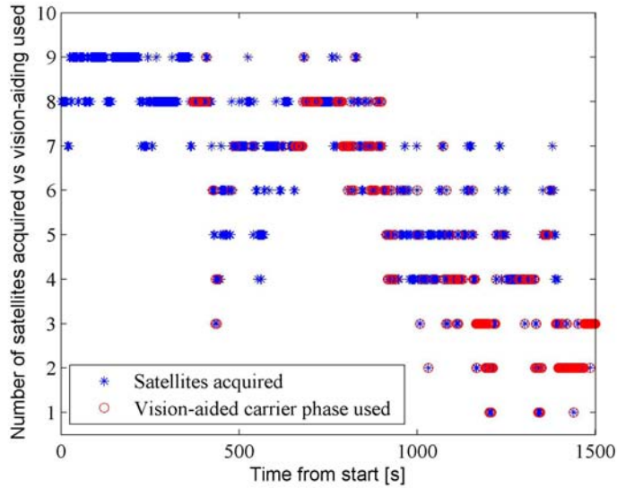
Fig. 7.4. Number of satellites acquired in an urban canyon for each time epoch of the experiment (blue) and the epochs when vision-aided carrier phase navigation used due to too few satellites or large residuals in GNSS pseudorange position estimations (red above the blue mark).
