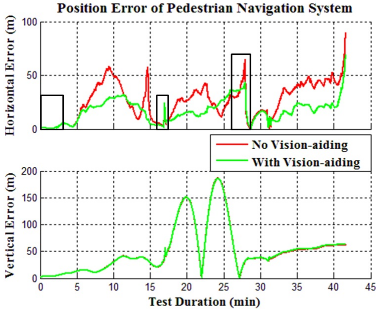
Fig. 6.16. RMS position errors obtained for foot-mounted IMU with (green) and without vision-aiding (red).
