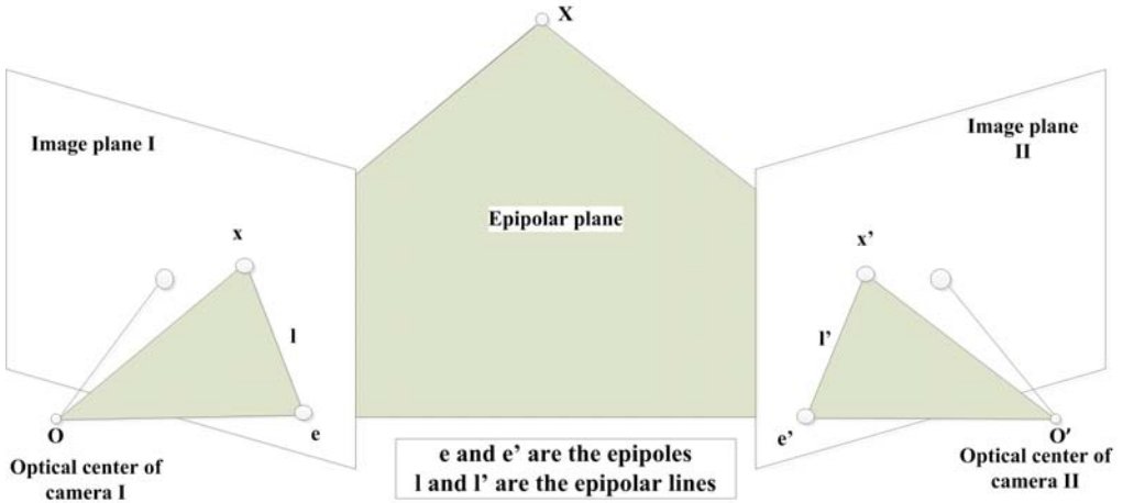
Fig. 3.2. The epipolar geometry between two images including epipolar plane, epipoles (e, e') and epipolar lines (l, l') [31].
