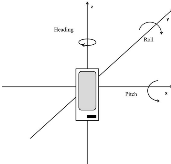
Fig. 2.1. Heading, pitch and roll in Navigation frame.
