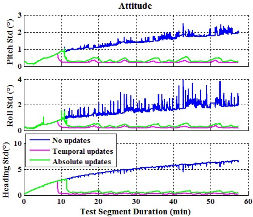
Fig. 6.12. Standard deviation for different integration schemes, namely no visual updates used (blue), using temporal updates (purple) and absolute updates (green).
