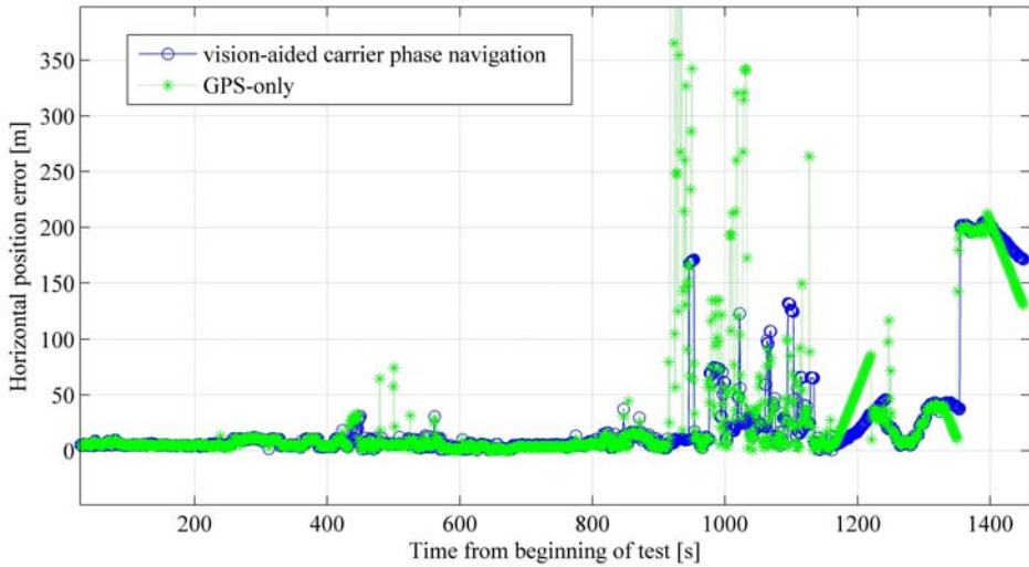
Fig. 7.6. Horizontal position error in an urban canyon obtained using vision-aided carrier phase navigation and GPS-only.
