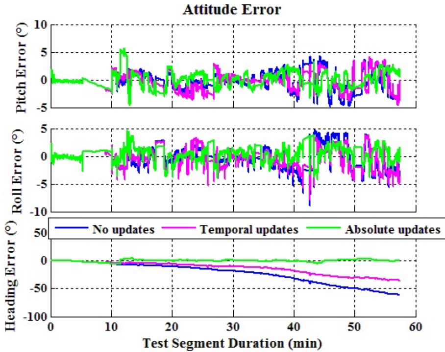
Fig. 6.13. Attitude error using different integration schemes, namely no visual updates used (blue), using temporal updates (purple) and absolute updates (green).
