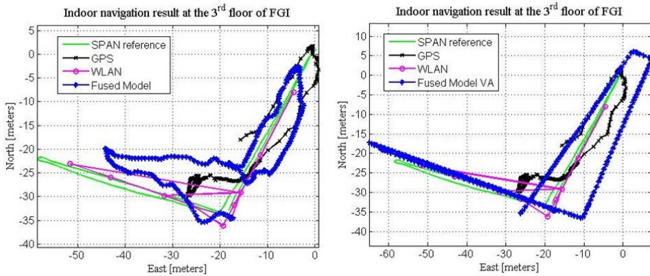
Fig. 6.5. Indoor positioning results for a pedestrian using different sensors and fused solutions in an office corridor with an outdated WLAN radio map. The figure on the left has a fused solution without visual-aiding (blue) and the figure on the right a fused solution using visual-aiding from the visual gyroscope and visual odometer (blue), ground truth (green), GPS position solution (black) and WLAN position solution (purple).
