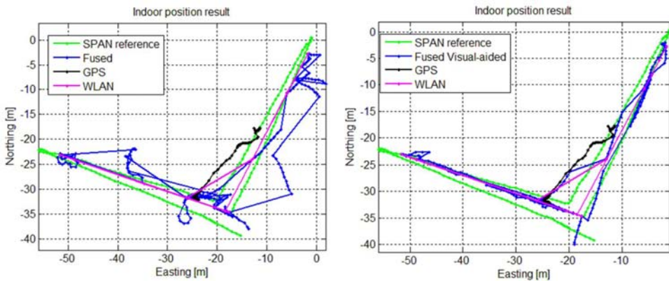
Fig. 6.4. Indoor positioning results for a pedestrian using different sensors and fused solutions. The figure on the left has a fused solution without visual-aiding (blue) and the figure on the right a fused solution using visual-aiding from the visual gyroscope and visual odometer (blue), ground truth (green), GPS position solution (black) and WLAN position solution (purple).
