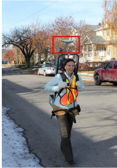
Fig. 7.1. Setup for data collection used in verification of vision-aided carrier phase navigation.
