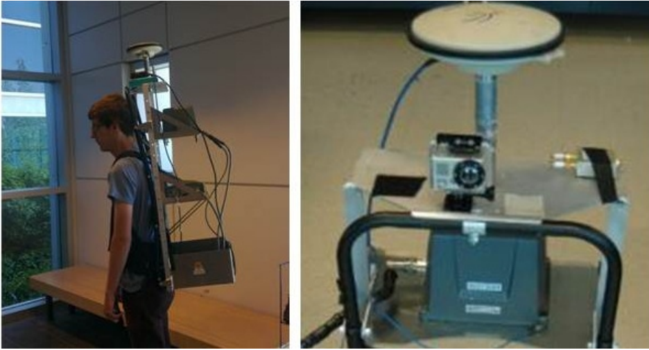
Fig. 6.11. Equipment attached to a backpack and carried by a user in a body mounted test (on left) and a close-up of the equipment (on right).
