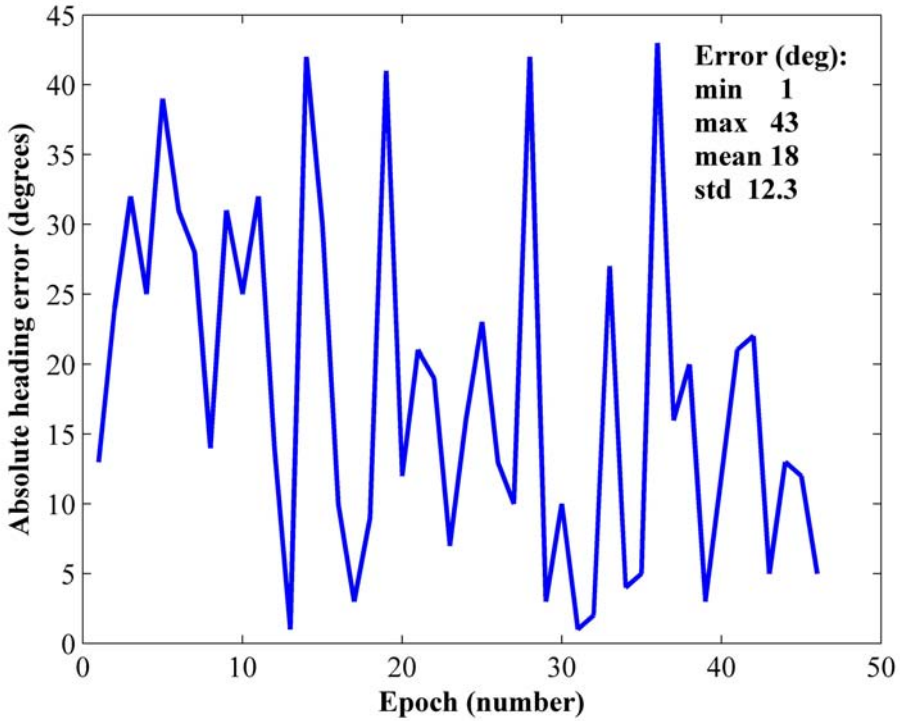
Fig. 2.2. Absolute heading error obtained with a digital compass of a smartphone indoors.
