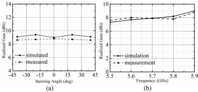
Fig. 6. Simulated gains and measured gains (a) versus steering angles at 5.9 GHz. (b) Simulated gains and measured gains of broadside beam versus frequencies.
