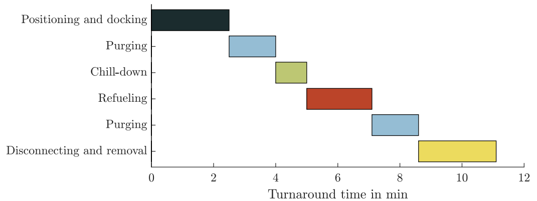
Figure 6. Gantt chart for LH2 refueling of 5350 kg; the energy corresponds to the maximum kerosene volume of A320-like aircraft.
