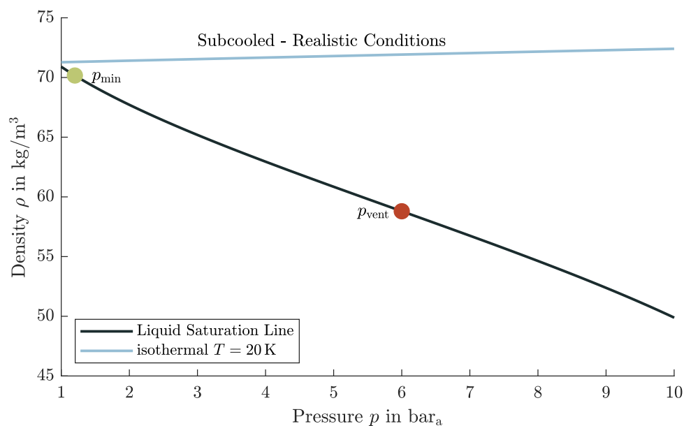
Figure 7. Density of LH2 over pressure for short term storage; difference between saturated and subcooled conditions.
