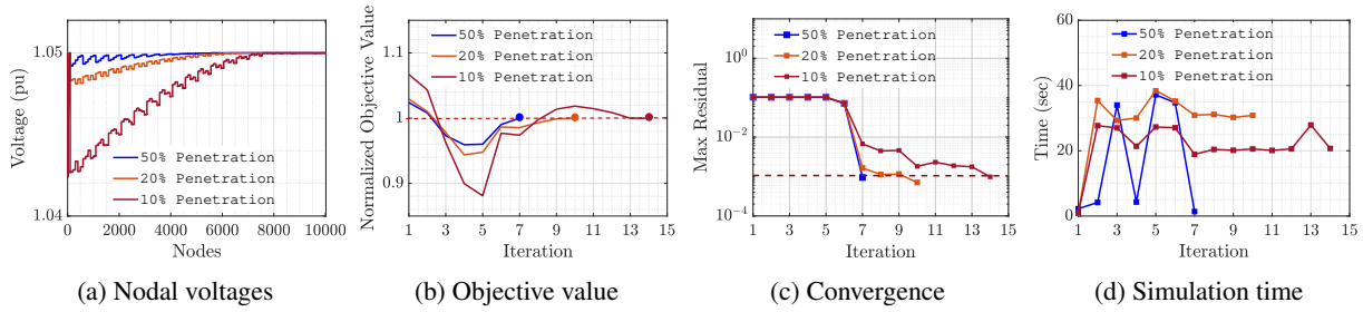
Figure 3: Numerical Results for DER Maximization Objective for Synthetic 10,000 Node System
