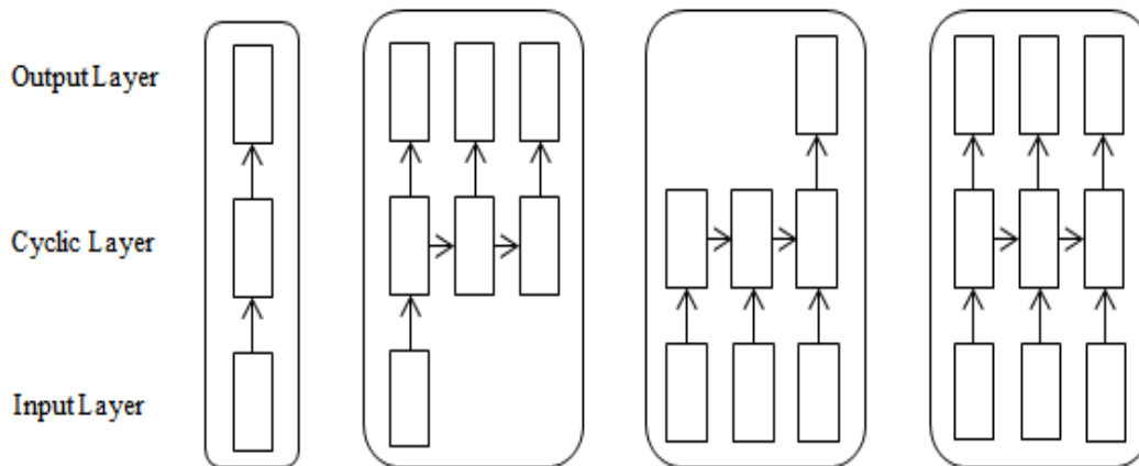
Figure 2. Common structure of cyclic neural network
