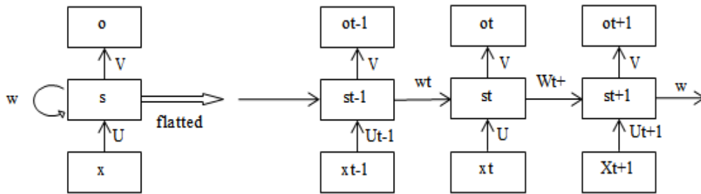
Figure 1. Basic structure of rnn network
