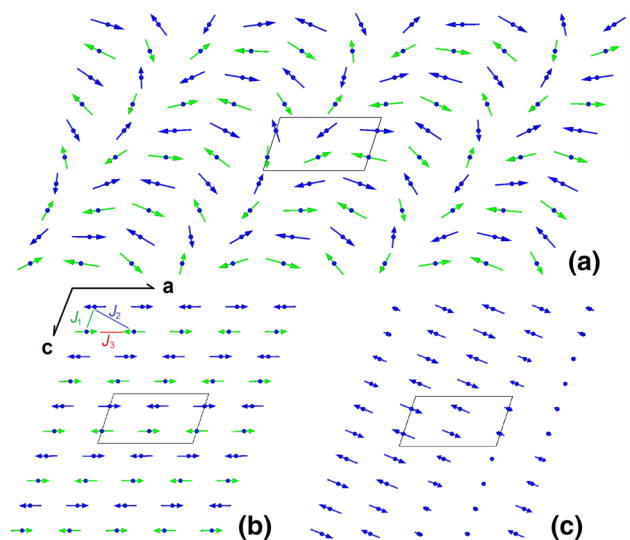
Fig. 11 Schematic drawings of the different magnetic structures in sample \text{Li}_{0.12}\text{Na}_{0.88}\text{FeGe}_2\text{O}_6 in a projection onto (0\ 1\ 0) : a cycloidal structure at 4 K, b simple collinear structure at 4 K and c spin density wave structure at 12.5 K
