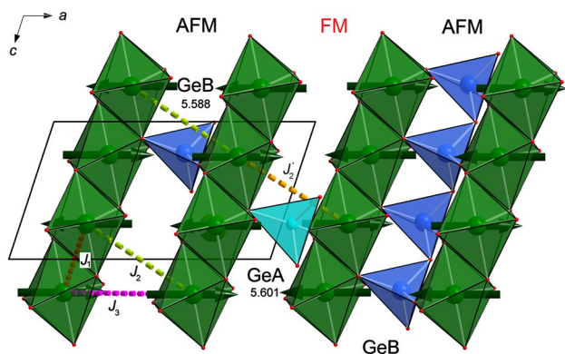
Fig. 6 Magnetic spin structure of P_{2_1}/c \text{Li}_{0.31}\text{Na}_{0.69}\text{FeGe}_2\text{O}_6 in a projection onto (0 1 0) at 4 K, as determined from neutron diffraction data. Note the different inter-chain couplings via GeA and GeB tetrahedral sites; J_1 , J_2 and J_2 and J_3 denote the possible pathways for magnetic super-exchange
