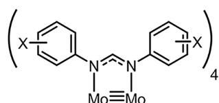
Figure 1. General structure of a homoleptic dimolybdenum tetraformamidinate complex [ \text{Mo}_2(\text{NN})_4 ].
