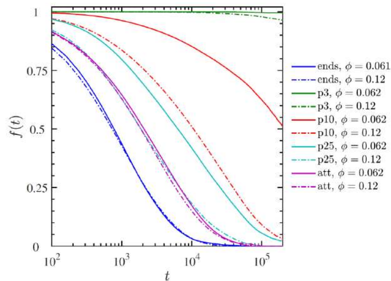
Figure 19. Survival probability f(t) versus reduced time t of ionic crosslinks for different nanoparticle volume fractions, polymer charge density, and localization of charges. Reprinted with permission from Mugemana et al. [120].
