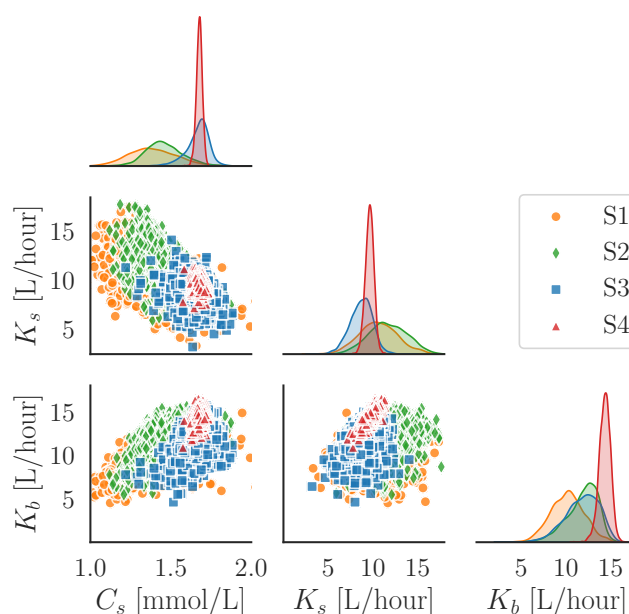
Figure 11. Plot of the posterior density and correlation for the parameter estimates for the four scenarios, S1, S2, S3, and S4. The density plots show the posterior density functions, and the scatter plots show the posterior samples. The uncertainty associated with the posterior mean of the parameters decreases as more information is included in terms of relapse measurement and /or consecutive sessions.
