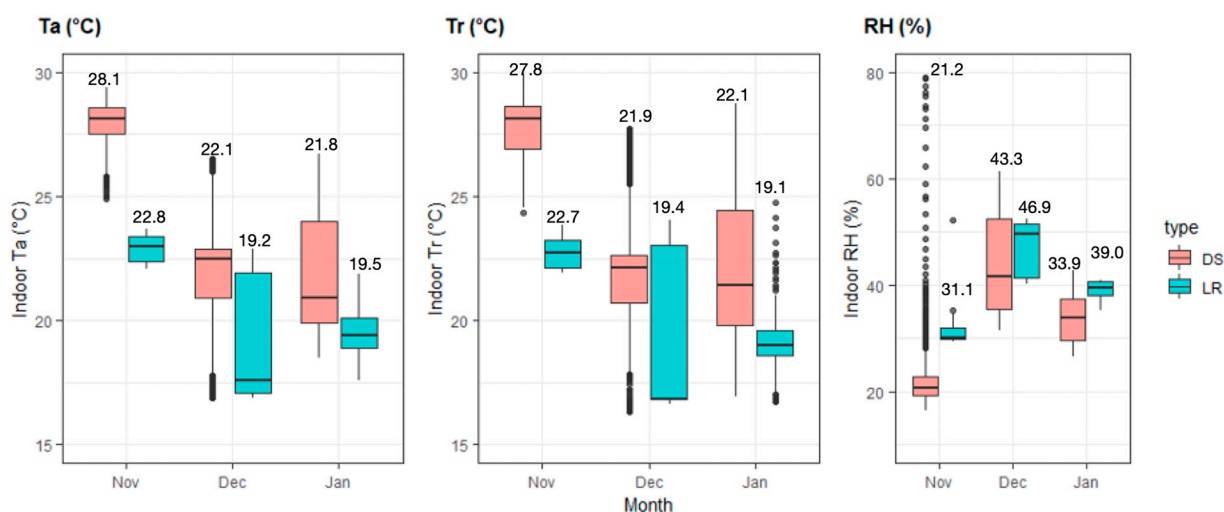
Figure 5. The monitored thermal conditions (i.e., T_a , T_r , RH) in the surveyed lecturer rooms between Nov 2021 and Jan 2022. Data were grouped on the basis of the university hall type; DS refers to the architecture design studio, LR refers to lecture rooms, whiskers indicate the minimum and maximum readings, black dots indicate the outliers, a bold black line indicate the median score, and the value beside each box-plot represents the mean score.
