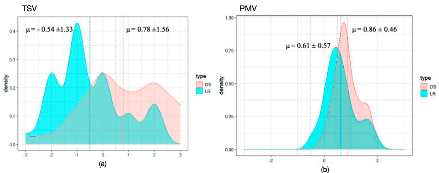
Figure 8. (a) Comparison of the observed TSV in design studios (DS) and lecture rooms (LR), and (b) the predictive mean vote (PMV) as predicted by Fanger's model ISO 7730 (2005). PMV data were calculated using spot measurements. The coloured dashed lines represent the mean score of variables, and the dotted grey line represents the recommended range by ISO 7730 [-0.5, +0.5] ; n_{\text{students}} = 173 .
