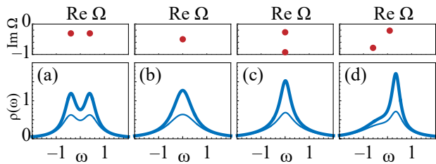
FIG. 1. Complex eigenvalue spectrum \Omega_k (top) and density of states \rho(\omega) (bottom) for the effective Hamiltonian (5). The couplings are fixed to b = c^* = 0.4 - 0.3i , while (a) a = \sqrt{-bc} - 0.2i (PT symmetric case), (b) a = \sqrt{-bc} (EP), (c) a = \sqrt{-bc} + 0.1i (dynamically broken phase), and (d) a = \sqrt{-bc} + 0.2 (symmetry explicitly broken). The thick lines are for the limit of weak couplings \Gamma = 0 , where the life times are maximized. At the exceptional point, \rho(\omega) is then a simple Lorentzian, which does not reveal the extreme mode nonorthogonality of the system. The thin lines are for finite \Gamma = 0.1 , where a squared-Lorentzian background of limited contrast appears at the EP.
