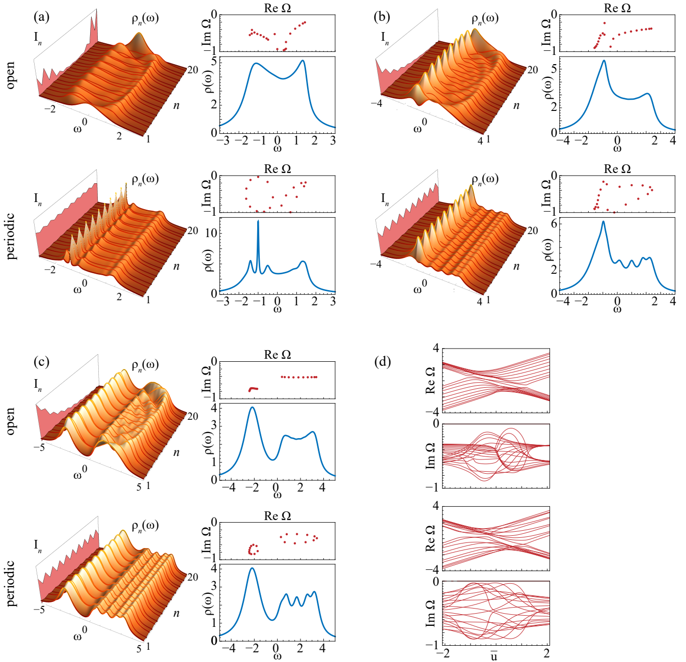
FIG. 6. Analogous to Fig. 5, but including next-nearest neighbour couplings w_1 = 0.2 , w_2 = 0.4 , while here (a) \bar{u} = 0 , (b) \bar{u} = 1 , (c) \bar{u} = 2 .
