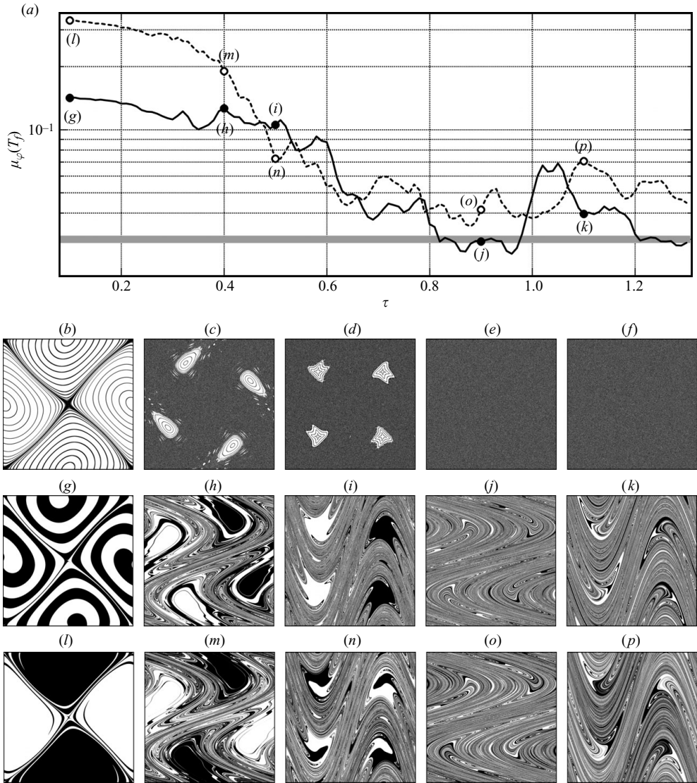
FIGURE 5. (a) Value of the mix-norm induced by the reference mixer at time T_f = 6 vs. switching time \tau for the ‘vertical’ (solid line) and the ‘envelope’ (dashed line) initial configurations. The grey horizontal line indicates the target mixing performance. (b–f) Poincaré sections of the reference mixer operating at switching time values 0.1 (b), 0.4 (c), 0.5 (d), 0.9 (e) and 1.1 (f). (g–k) Snapshots at time T_f = 6 of the concentration field \varphi stirred by the reference mixer operating at switching time values 0.1 (g), 0.4 (h), 0.5 (i), 0.9 (j) and 1.1 (k) when applied to the ‘vertical’ initial configuration. (l–p) Snapshots at time T_f = 6 of the concentration field \varphi stirred by the reference mixer operating at switching time values 0.1 (l), 0.4 (m), 0.5 (n), 0.9 (o) and 1.1 (p) when applied to the ‘envelope’ initial configuration. The filled circle and the open circle markers within panel (a) correspond to the concentration fields (g–k) and (l–p), respectively.
