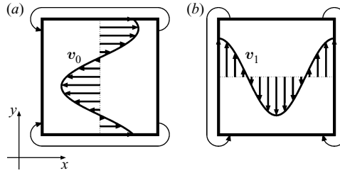
FIGURE 8. The schematic of the mixing device equipped with the new actuating system defined by velocity fields (5.1). (a,b) The stirring velocity fields v_0 shifted by \psi = 0.333 and v_1 shifted by \psi = 0.25 . The curves joining the opposite sides of the square mixing domain indicate periodic boundary conditions.
