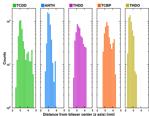
Fig. 7 Distribution of distances between cluster and membrane centers along the z axis. Line height represents the number of occurrences.
